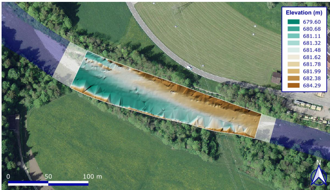
815 Figure A3. High-resolution (25 cm) riverbed DEM used to define the 3D meshes of the test case (background image from © Google Maps 2024).
