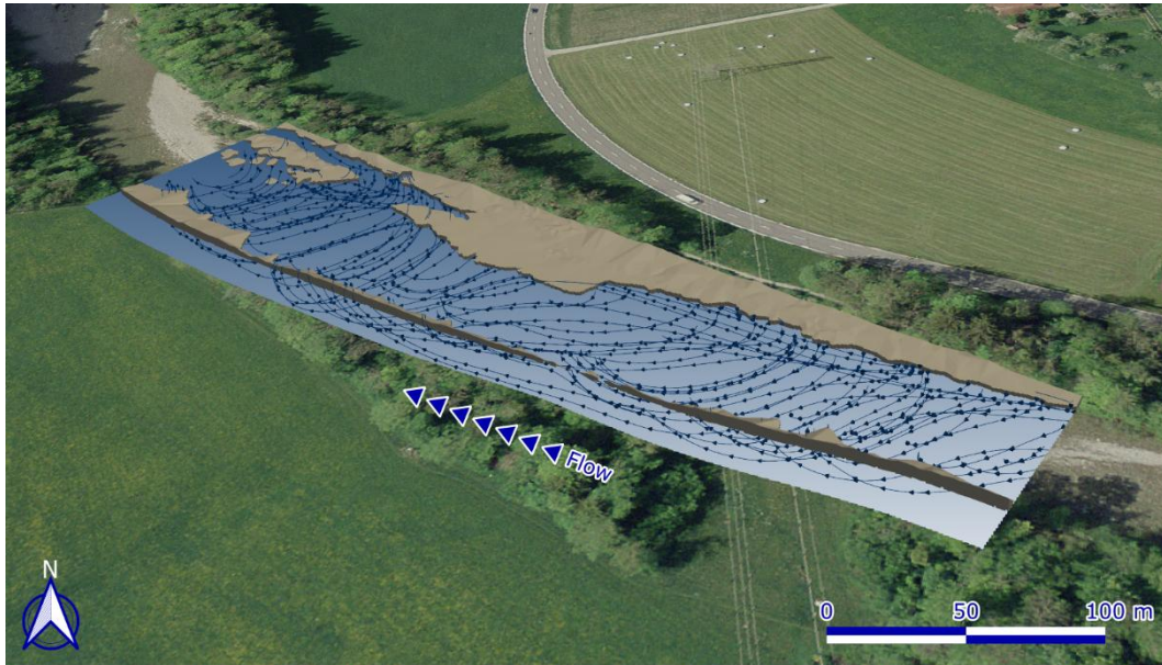
825 Figure A4. 3D view of the simulated groundwater flowpaths underneath the riverbed (background image from © Google Maps 2024).
