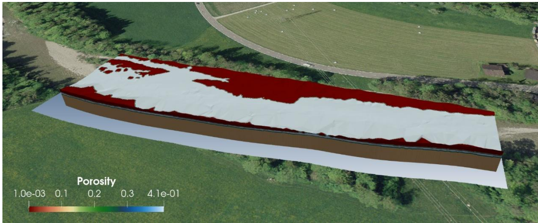
605 Figure 4. Porosity field ( \theta_i ) of the test case (background image from © Google Maps 2024).
