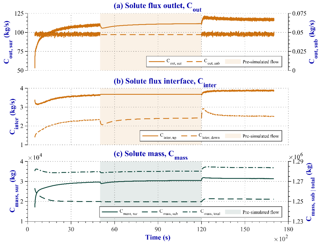
775 Figure 10. Solute flux across the (a) outlet and (b) interface boundaries. (c) Solute mass in each simulated domain and total mass in the system. The subscripts sur and sub refer to surface and subsurface domains, respectively, while up and down indicate upwelling and downwelling fluxes. The coloured area corresponds to the simulation period in which the pre-simulated flow field was used to only run solute transport.
