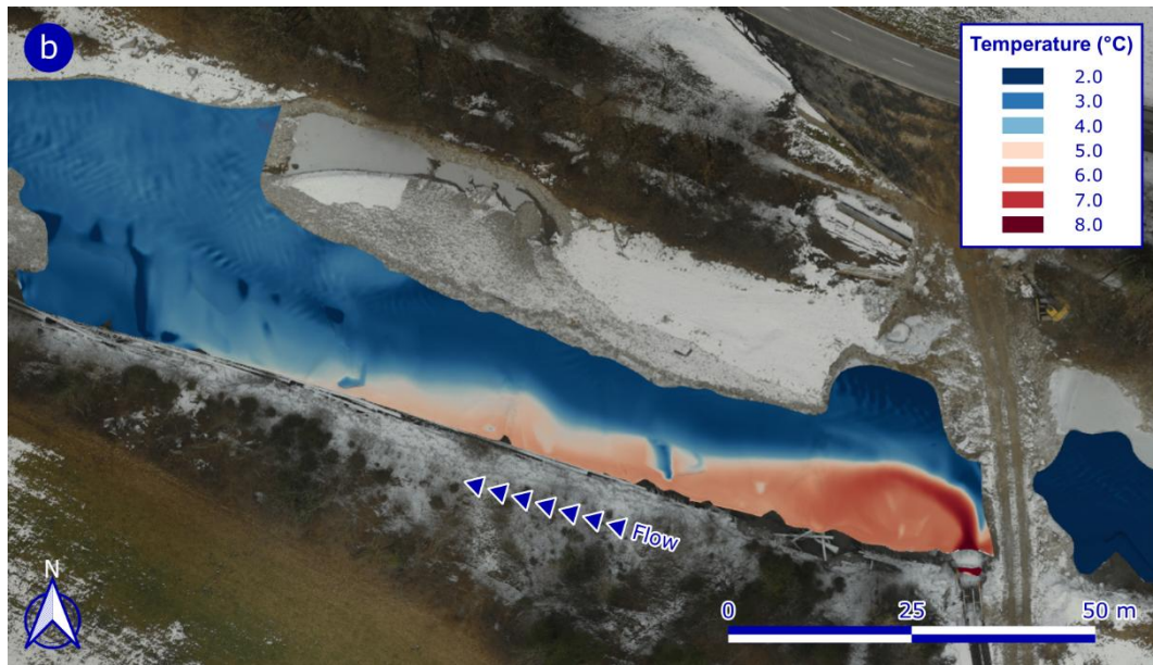
Figure 6. (a) Drone-measured and (b) simulated temperature plumes generated by the groundwater jet at the water surface (background image captured on site by the drone).
