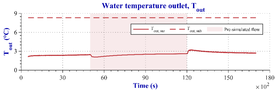
745 Figure 8. Average water temperature across the surface and subsurface outlet boundaries. The subscripts sur and sub refer to surface and subsurface domains, respectively. The coloured area corresponds to the simulation period in which the pre-simulated flow field was used to only run heat transfer.
