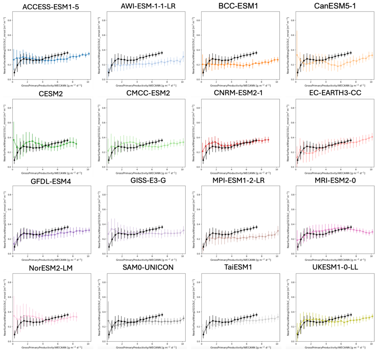
460 Figure 8: Similar to the bias plots shown in Figure 7A, but for all models. These plots highlight the observed relationships (black curves) between the surface SM (from the Wang2021OLC top 10 cm SM product) and GPP (from WECANN), as well as the relationship shown in each model (colored curves) using the simulated mrsol to 10 cm and gpp variables.
