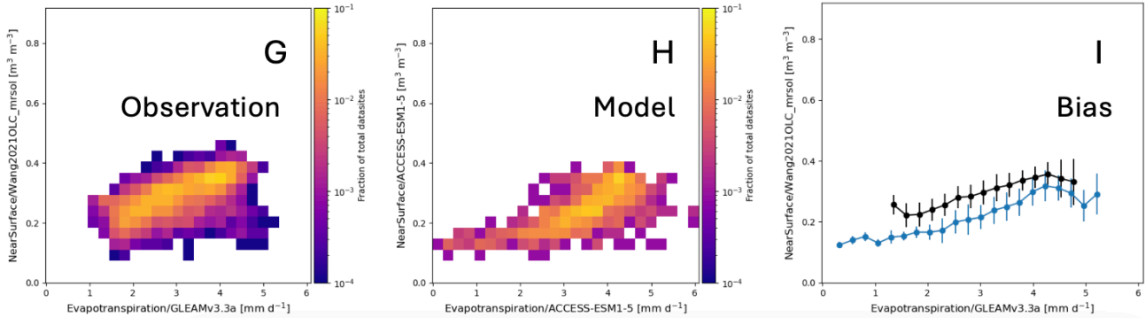
Figure A6: Relationships between surface SM and ecohydrologic variables, similar to Figure 7, but for the “Tropical” Köppen region. The model results shown here are for the ACCESS-ESM1-5 model. Panels A, D, and G show the heat maps of the observed relationships, panels B, E, and H show the heat maps of simulated relationships in the ACCESS-ESM1-5 model, and panels C, F, and I portray both the observed and simulated relationships in the form of dot and whisker plots for easy comparison.
