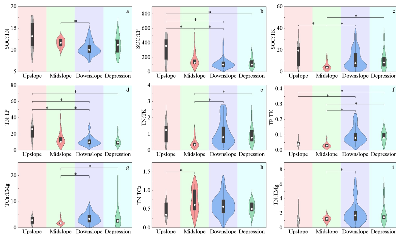
Figure 4. Distribution differences in stoichiometric ratios of major soil nutrients across different slope position types, presented as violin plots overlaid with box plots. The Y-axis of each subplot denotes the values of corresponding ratios, while the X-axis represents slope position types. An asterisk (*) indicates significant intergroup differences ( P < 0.05 ), with black horizontal lines connecting groups exhibiting differences. The number of samples (n) for each slope position type is as follows: upslope (n = 6), midslope (n = 18), downslope (n = 49), depression (n = 13).
