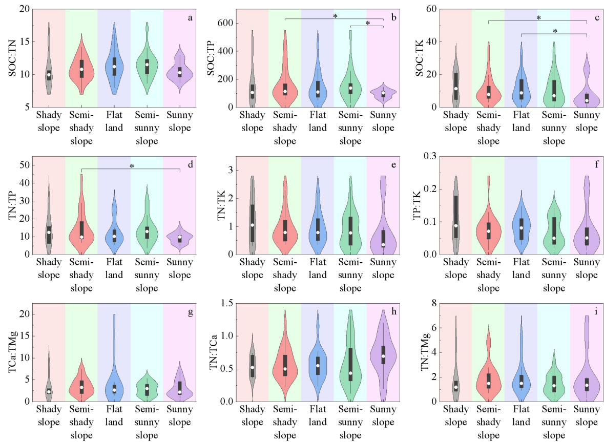
275 Figure 3. Distribution differences in stoichiometric ratios of major soil nutrients across different slope aspect types, presented as violin plots overlaid with box plots. The Y-axis of each subplot denotes the values of corresponding ratios, while the X-axis represents slope aspect types. An asterisk (*) indicates significant intergroup differences ( P < 0.05 ), with black horizontal lines connecting groups exhibiting differences. The number of samples ( n ) for each slope aspect type is as follows: shady slope ( n = 6 ), semi-shady slope ( n = 22 ), flat land ( n = 16 ), semi-sunny slope ( n = 19 ), sunny slope ( n = 23 ).
