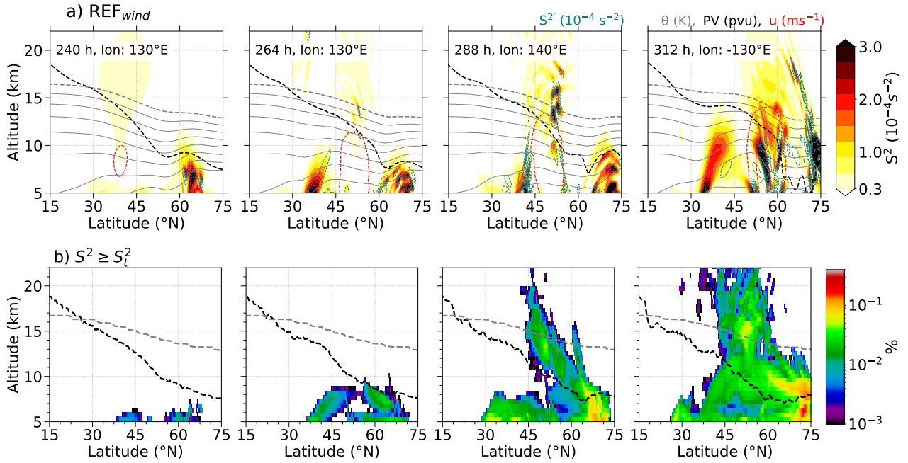
Figure 13. The temporal evolution of (a) vertical cross section of shear through the identified regions of GWs from time 240 h onward for REF wind simulation with S^{2'} (dashed green), potential temperature (grey), zonal wind (30 m.s -1 , red) and dynamical tropopause (black) and (b) the respective Northern hemispheric occurrence frequency distribution of grid volumes that exhibit S^2 \geq S_t^2 . Logarithmic frequency contour, vertically binned in dz=500 m is applied. The zonal mean value of 3.5 PVU in the potential vorticity field is indicated by the dashed black line, and the zonal mean value of 380 K in the potential temperature field is indicated by the grey dashed line.
