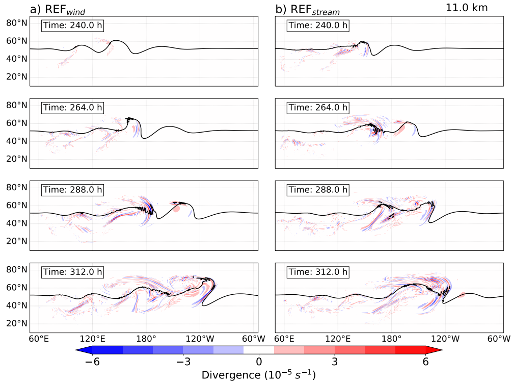
Figure 3. The evolution of the GWs for the (a) \text{REF}_{\text{wind}} and (b) \text{REF}_{\text{stream}} simulation. Horizontal cross sections of horizontal divergence at 11 km altitude over the Northern Hemisphere after 240 h, 264 h, 288 h and 312 h of model integration time, respectively. The solid black line represents the dynamical tropopause.
