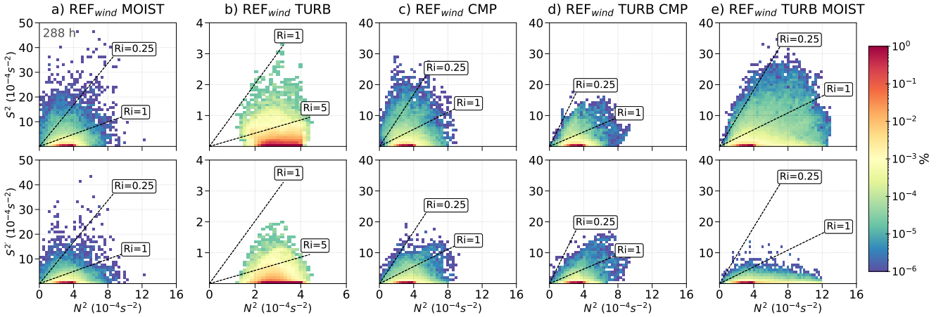
Figure 10. As in Figure 9 but after 288 h for the REF wind simulations with varying physical processes.
