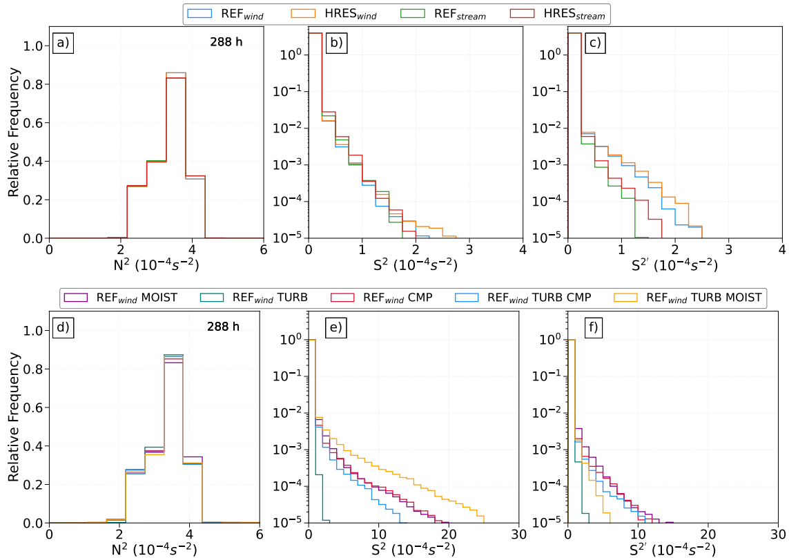
Figure 8. Temporal evolution of relative occurrence frequency distribution of N^2 (a, d), S^2 (b, e) and S^{2'} (c, f) in the lowermost stratosphere over the Northern Hemisphere. Upper panel (a, b, c) represents grid spacing sensitivity experiments. Lower panel (d, e, f) represents physics sensitivity experiments performed using wind perturbation function. LMS is defined as the region between 3.5 PVU, a dynamical tropopause and 380 K isentropic surface.
