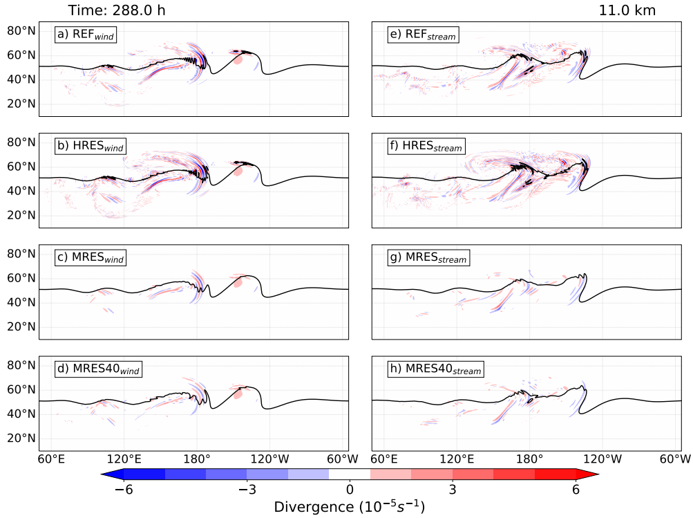
Figure 4. Evolution of GWs for simulations with varying grid spacings. Panels (a-d) represent simulations with wind perturbations for experiments REF, HRES, MRES, and MRES40, respectively, while panels (e-f) show simulations with stream perturbations for the same configurations. The figure displays the distribution of the horizontal divergence field at 11 km altitude over the Northern Hemisphere after 288 h of model integration.
