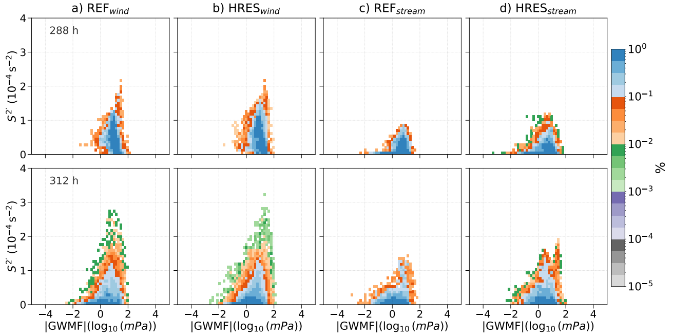
Figure 11. Relative occurrence frequency or probability density distribution of absolute momentum flux due to GWs |GWMF| -vertical shear perturbations S^{2'} pair in the LMS for Ri \leq 5 after 288 h (upper panel) and 312 h (lower panel) for simulations with grid spacing sensitivity. Normalized counts of PDFs distribution. Logarithmic occurrence frequency color scale is applied.
