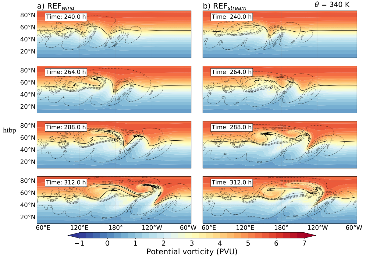
Figure 2. The evolution of the baroclinic life cycle for the (a) \text{REF}_{\text{wind}} and (b) \text{REF}_{\text{stream}} simulation. Horizontal cross sections of potential vorticity at 340 K isentropic surface and surface pressure (dashed contours) over the Northern Hemisphere after 240, 264, 288 and 312 h of model integration. The solid black line represents the 3.5 PVU, regarded as a dynamical tropopause.
