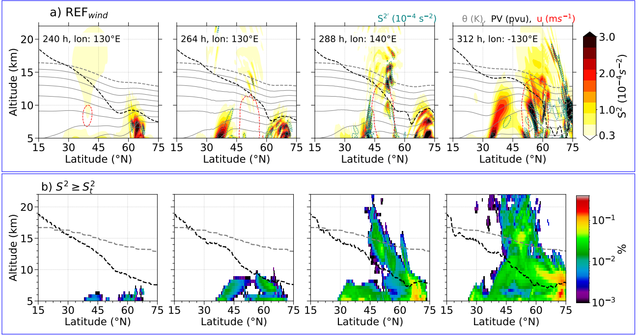
Figure 13. The temporal evolution of (a) vertical cross section of shear through the identified regions of GWs from time 240 h onward for \text{REF}_{\text{wind}} simulation with S^2 (dashed green), potential temperature (grey), zonal wind ( 30 \text{ m.s}^{-1} , red) and dynamical tropopause (black) and (b) the respective Northern hemispheric occurrence frequency distribution of grid volumes that exhibit S^2 \geq S_t^2 . Logarithmic frequency contour, vertically binned in dz=500 \text{ m} is applied. The zonal mean dynamical tropopause altitude value of 3.5 PVU in the potential vorticity field is indicated by the dashed black line, and tropical tropopause (the zonal mean value of 380 K isentrope) in the potential temperature field is indicated by the grey dashed line.
