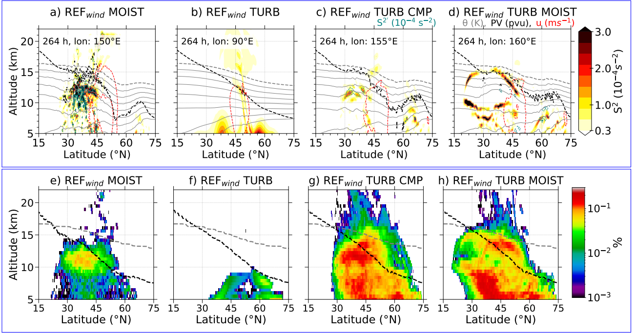
Figure 14. Vertical cross section of shear ( upper-panel a-d ) through the identified regions of GWs at 264 h \text{REF}_{\text{wind}} simulations with physical processes sensitivity and the respective Northern hemispheric occurrence frequency distribution of grid volumes that exhibit S^2 \geq S_t^2 ( lower-panel e-h ). Logarithmic frequency contour, vertically binned in \text{dz}=500 m is applied . The zonal mean dynamical tropopause altitude is indicated by the dashed black line and tropical tropopause (380 K isentrope) by grey dashed line.
