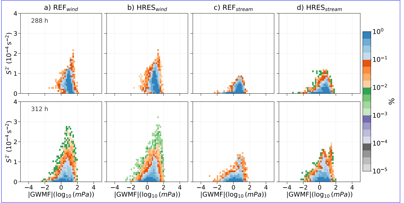
Figure 11. Relative occurrence frequency or probability density distribution of absolute momentum flux due to GWs |GWMF| -vertical shear S^{2'} on small scale, pairs perturbations S^{2'} pair in the LMS for Ri \leq 5 for simulations with grid spacing sensitivity. Normalized counts of PDFs distribution. Logarithmic occurrence frequency color scale is applied.
