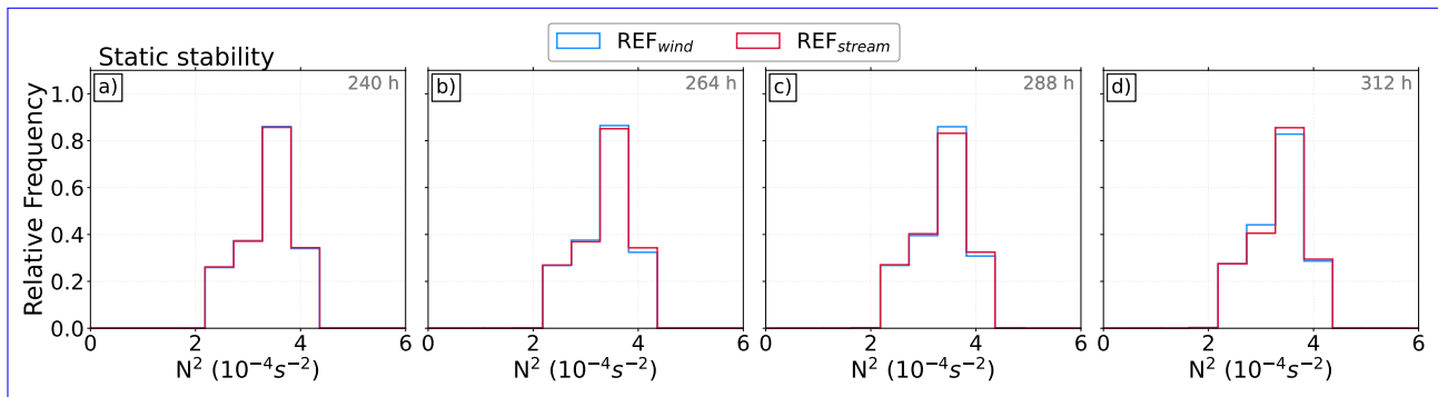
Figure A1. The temporal evolution of PDFs of static stability, N^2 in the lowermost stratosphere for dry reference experiments.
