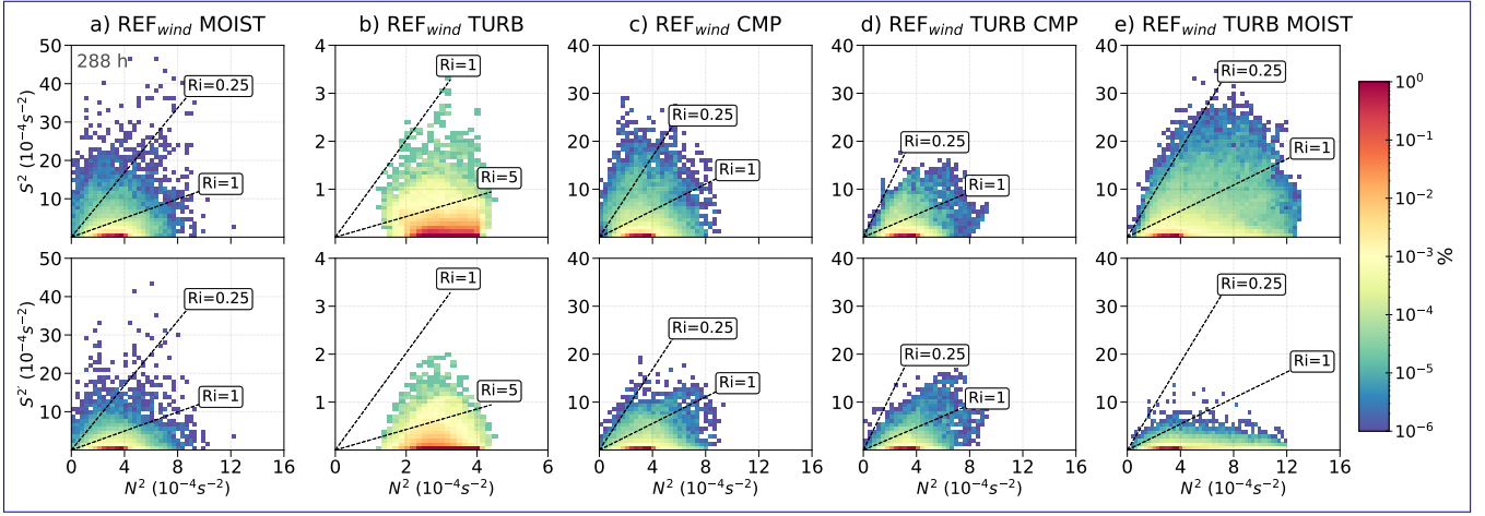
Figure 10. As in Figure 9 but after 288 h for the REF wind simulations with varying physical processes.
