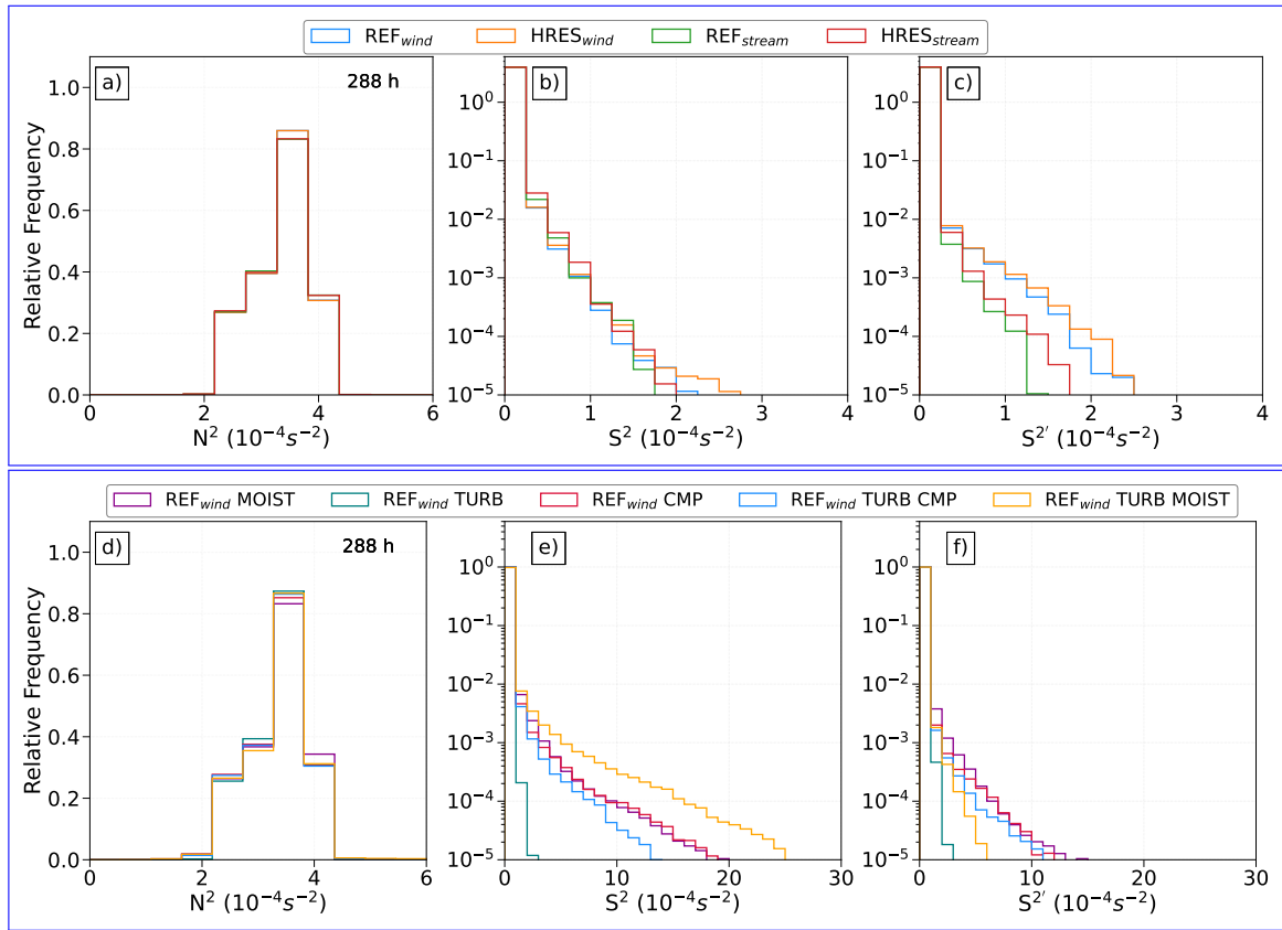
Figure 8. Temporal evolution of relative occurrence frequency distribution of N^2 (a-d), S^2 (b-e) and S'^2 (c-f) in the lowermost stratosphere over the northern hemisphere Northern Hemisphere . Upper panel (a-b-c) represents grid spacing sensitivity experiments. Lower panel (d-e-f) represents physics sensitivity experiments performed using wind perturbation function. LMS is defined as the region between 3.5 pva PVU , a dynamical tropopause and 380 K isentropic surface.
