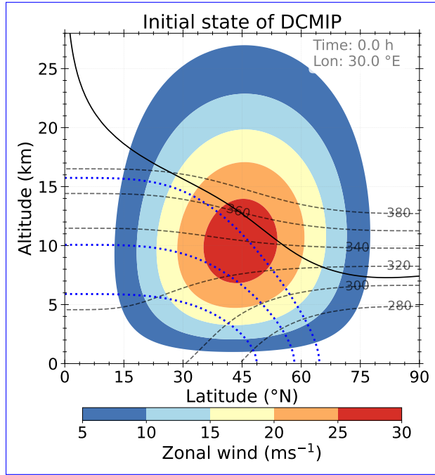
Figure 1. Zonally symmetric balanced initial conditions at 30° E longitude: zonal wind \bar{u} (shaded contours, 5 ms -1 spacing), potential temperature \theta (solid black dashed grey lines, 15-20 K spacing, starting with 380-280 K in the lower right corner) and specific humidity q_v for values 0.002, 0.02, 0.052, 0.2, 0.5, 1, g kg -1 and 0.02 g kg -1 (dotted blue lines, from bottom to top), the black thick dashed line marks the location of dynamical tropopause, defined as the 3.5 PVU potential vorticity isosurface.
