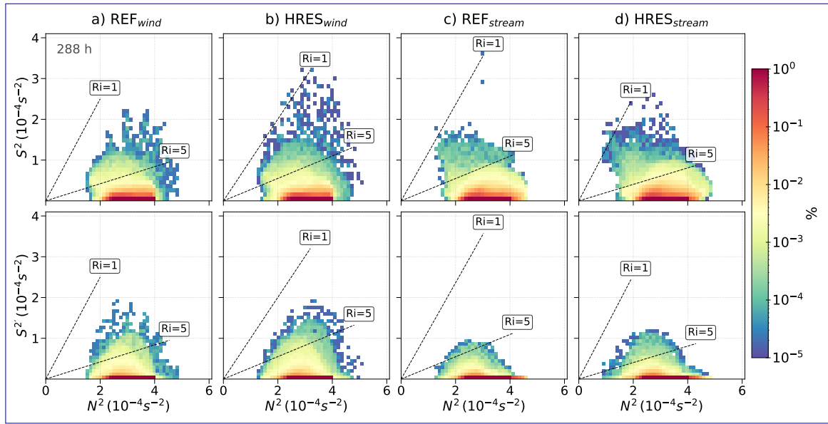
Figure 9. Relative occurrence frequency distribution of N^2 - S^2 (upper panel) and N^2 - S^2' (lower panel) pairs-pair plot after 288 h for simulations with varying grid sensitivity over northern-hemisphere-Northern Hemisphere in the lowermost stratosphere. Logarithmic occurrence frequency color scale is applied. Dashed lines indicates the gradient Richardson numbers.
