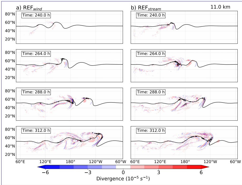
Figure 3. The evolution of the GW for the a) \text{REF}_{\text{wind}} and b) \text{REF}_{\text{stream}} simulation. Horizontal cross sections of horizontal divergence at 11-km-11 km altitude over the Northern Hemisphere after 240 h, 264 h, 288 h, and 312 h of model integration time, respectively. The solid black line represents the dynamical tropopause.
