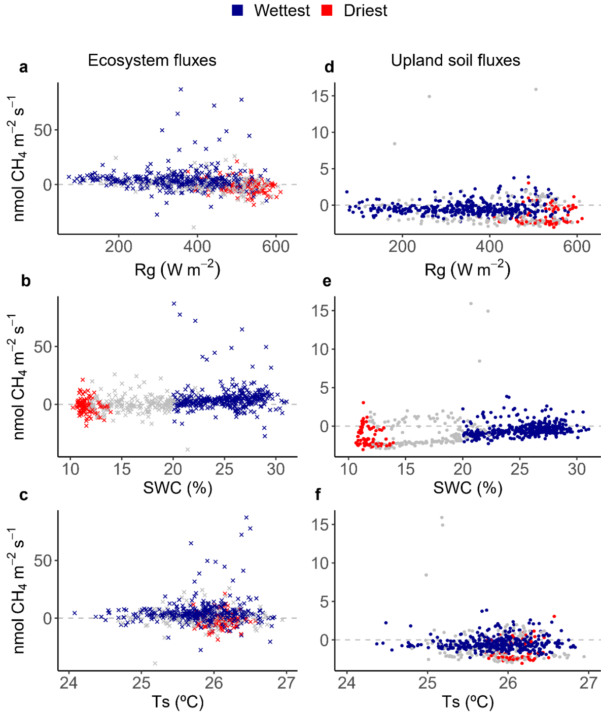
Figure 4. Relationships between environmental drivers (global radiation (Rg), soil water content (SWC) and soil temperature (Ts)) and daily average ecosystem (crosses on the left) and upland soil (solid dots on the right) \text{CH}_4 fluxes for the wettest (blue) and driest (red) seasons, with remaining data in grey, from 17 May, 2016 to 2 August, 2018 in the Guyaflux tropical forest, French Guiana. Positive fluxes above the horizontal “0” line indicate \text{CH}_4 emissions and negative fluxes below the horizontal “0” line indicate \text{CH}_4 uptake. Comparable relationships with the 1 st - 99 th percentile range of \text{CH}_4 flux data are shown in Fig. S6.
