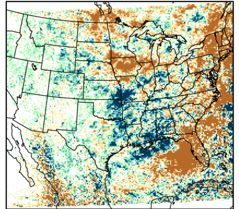
GLENS-PSAI
