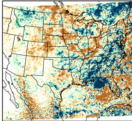
GLENS-PGW
