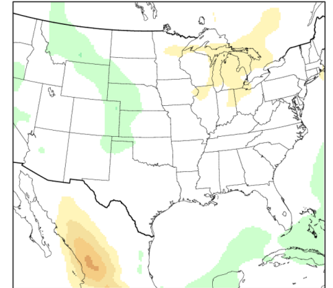
GLENS-PSAI
