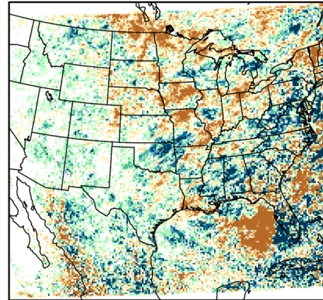
ARISE-PSAI
