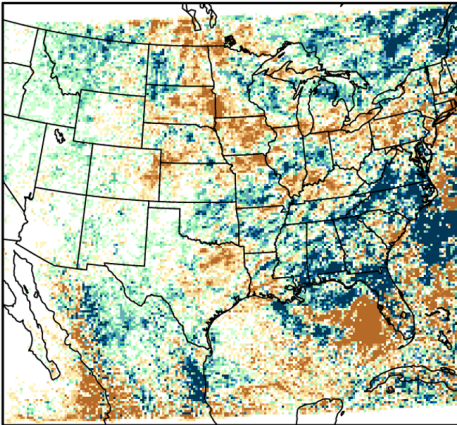
ARISE-PGW
