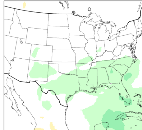
ARISE-PSAI
