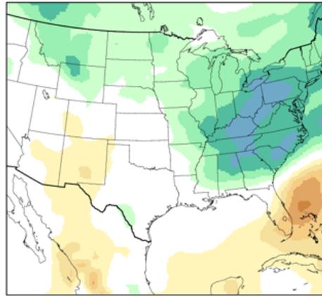
GLENS-PGW
