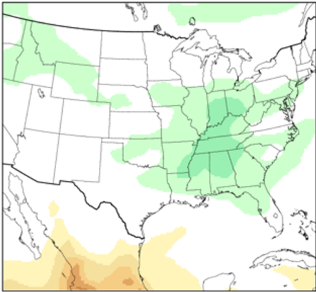
ARISE-PGW
