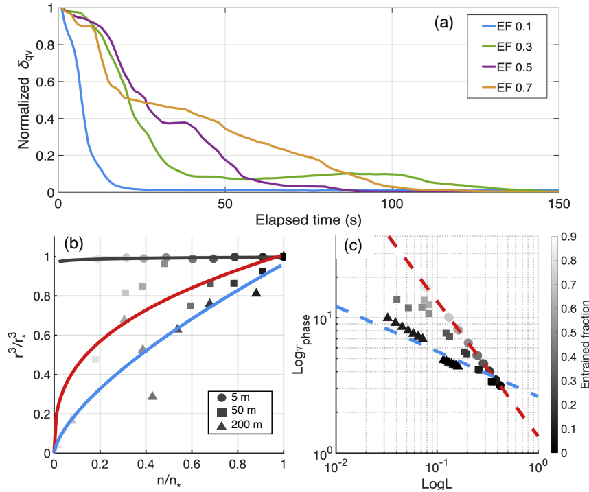
951 Figure 4: (a) Normalized standard deviation of water vapor ( \delta_{qv} ) in the parcel after entrainment 952 for the control experiment. The blue, green, purple and yellow line represents the parcel with EF 953 of 0.1, 0.3, 0.5 and 0.7. (b) and (c): Mixing diagrams for control experiment. The left panel (b) 954 represents the n-r^3 mixing diagram where the circle, square and triangle represents simulations at 955 5, 50 and 200m from cloud top. The black (IM-like), red (HM-like) and blue (HM-like) lines 956 represent the polynomial fitting of the parcels at each height level. (c) The right panel indicates 957 the L-\tau_{\text{phase}} mixing diagram, where the circle, square and triangle represents simulations at three 958 heights as indicated in (b). The red, blue dashed line represents the IM and HM reference line with 959 slope of -1 and -1/3.
