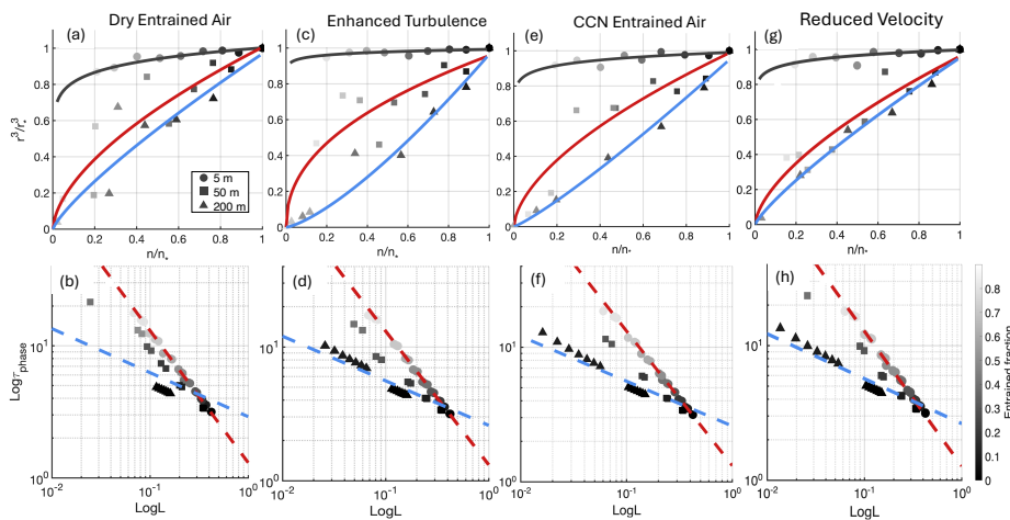
Figure 5: Same as Figure 4, but for the four sensitivity experiments: (a)–(b) correspond to the Dry-Entrained-Air experiment; (c)–(d) to the Enhanced-Turbulence experiment; (e)–(f) to the CCN-Entrained-Air experiment; and (g)–(h) to the Reduced-Velocity experiment.
