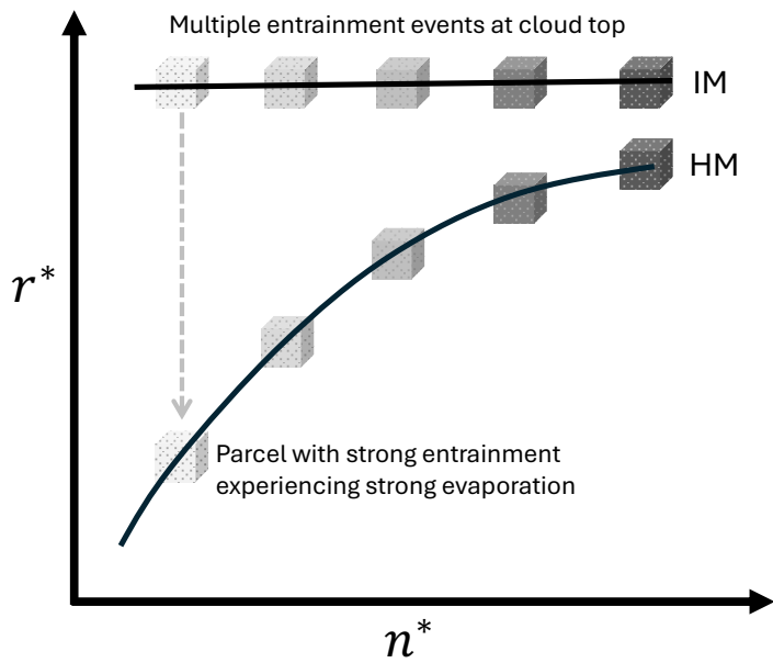
1074 Figure 10; Illustration of the IM-HM transition within Sc from the bulk perspective. Parcels with 1075 darker (lighter) shading corresponds to samples with lower (higher) entrainment fractions. The 1076 horizontal black line represents the IM behavior occurring near cloud top, the curved line 1077 represents the HM behavior occurring within cloud.
