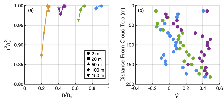
1023 Figure 7: a) n-r^3 mixing diagram from the parcel-based perspective for the strict IM experiment. 1024 The circle, square, triangle, diamond and the reverse-triangle indicate the parcel at height of 2m, 1025 20m, 50m, 100m and 150m from cloud top. The blue, green, purple and yellow represents parcel 1026 with EF of 0.1, 0.3, 0.5 and 0.7. b) The homogeneous mixing degree ( \psi ) as a function height for 1027 the strict IM experiment. The blue, green, purple color represents parcel with EF of 0.1, 0.3, 0.5.
