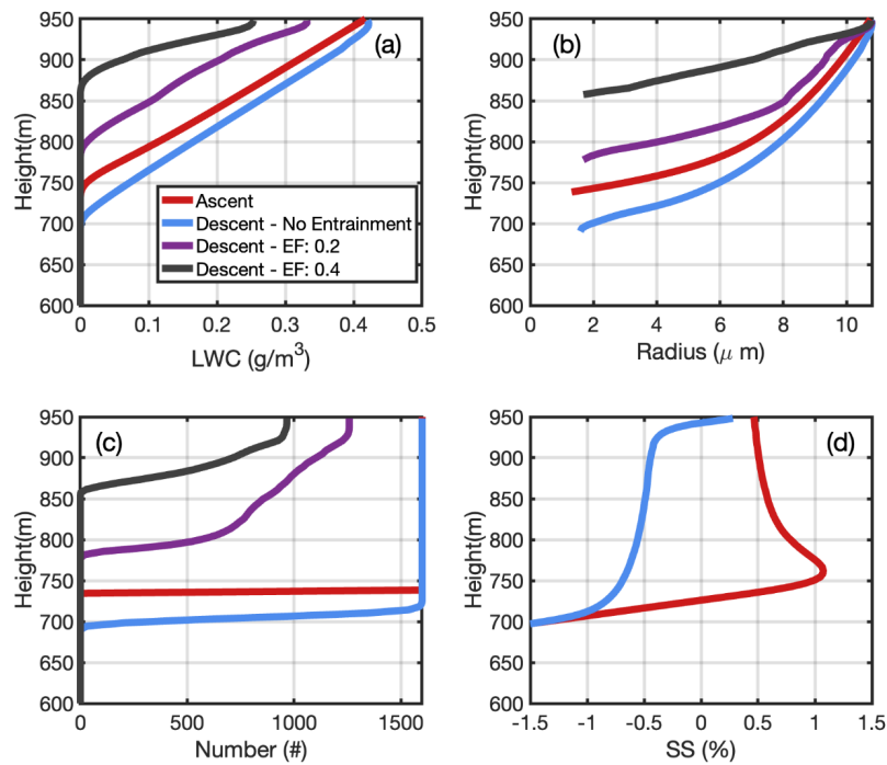
944 Figure 3: For the control experiment, domain-averaged cloud properties as function of height: a) 945 LWC, b) radius, c) droplet number d) supersaturation. The red line represents the ascending parcel, 946 while the blue, purple and black lines represent the descending parcel with entrainment fraction of 947 0, 0. 2 and 0.4 respectively. In (d) only the ascending parcel and the descending parcel with EF of 948 0. 4 is shown.
