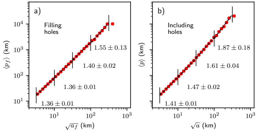
Figure 5. Dependence of the individual cloud fractal dimension on scale for clouds without with holes filled (a) and with without filling holes (b) for a threshold R = 0.1 . The perimeters p_f and areas a_f are obtained from clouds after any holes are filled in, while p and a are calculated as described in Sect. 2. Each point represents the mean perimeter in a logarithmically-spaced area bin. The listed fractal dimensions D_i are calculated using regressions (dashed lines) to four different size ranges delineated by the vertical black lines.
