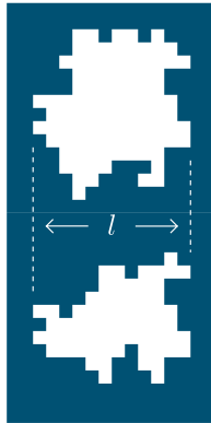
Figure 3. Two clouds may have different perimeters even if they are have the same size l (defined here as bounding box width) and are measured at the same resolution \xi .
