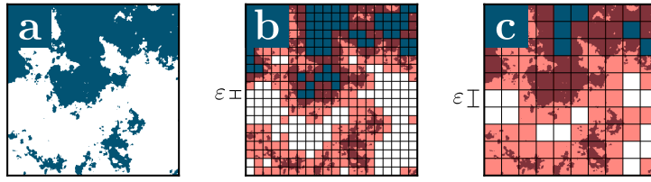
Figure 8. Calculation of the box dimension from a binary cloud mask (panel a). A grid with varying box size \varepsilon is overlaid on the cloud mask (panels b and c) such that each box contains \varepsilon \times \varepsilon image pixels. Here, \varepsilon = 25 for panel b and \varepsilon = 50 for panel c. The number of boxes required to cover all cloud edges (marked in red) are counted as a function of \varepsilon to obtain N(\varepsilon) .
