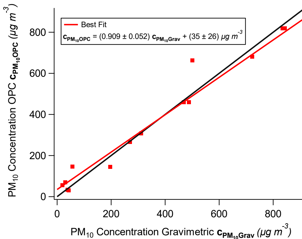
305 Figure 5. Comparison of PM 10 measurements at 3 m using OPC and Gravimetry. The black line represents the unity function. The linear function of best fit is presented along with associated standard errors.
