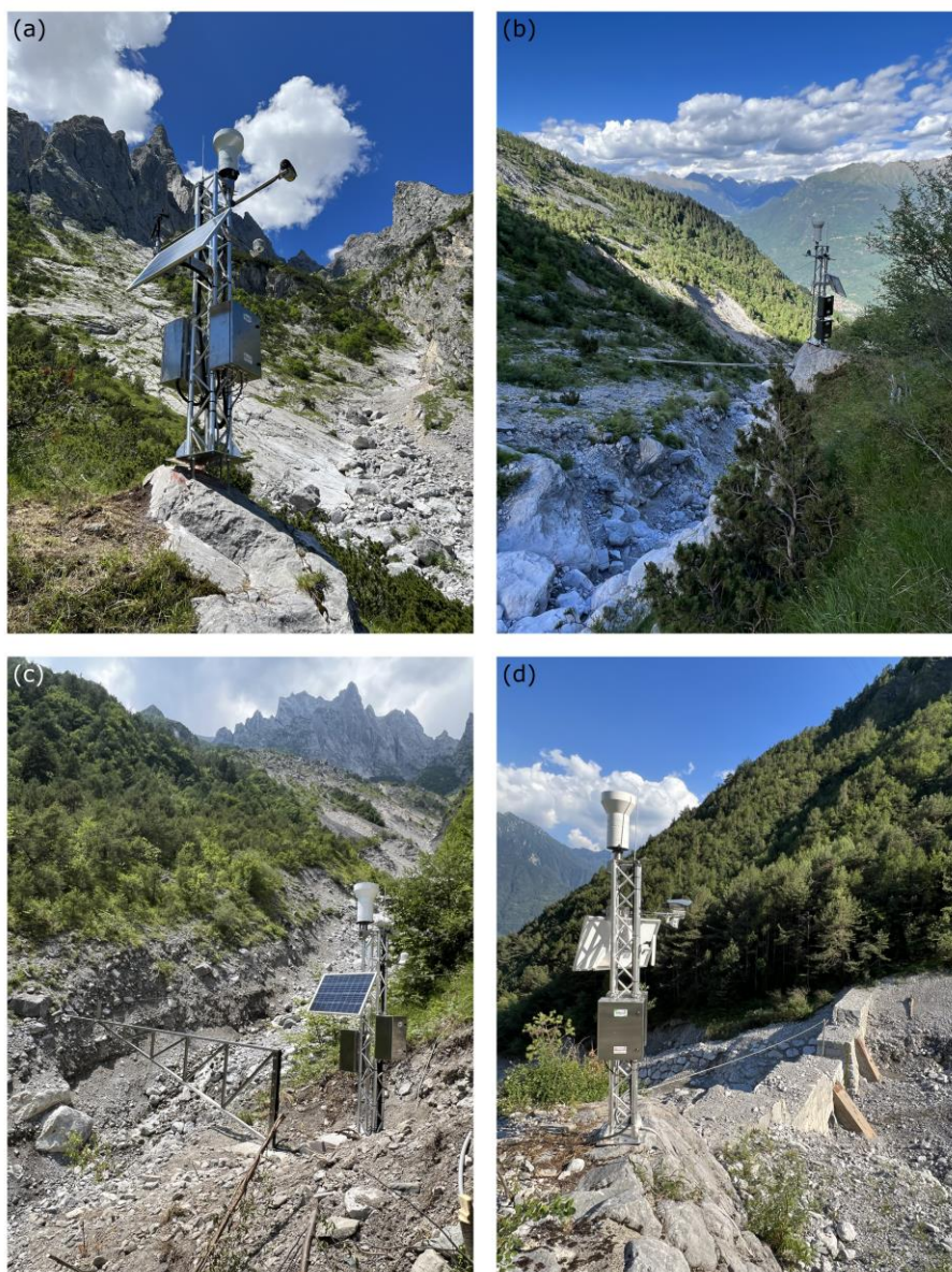
135 Figure 5: Photos of the four uppermost stations of Hortus S.r.l. network for monitoring and warning a) H1, b) H2, c) H3, d) H4.
