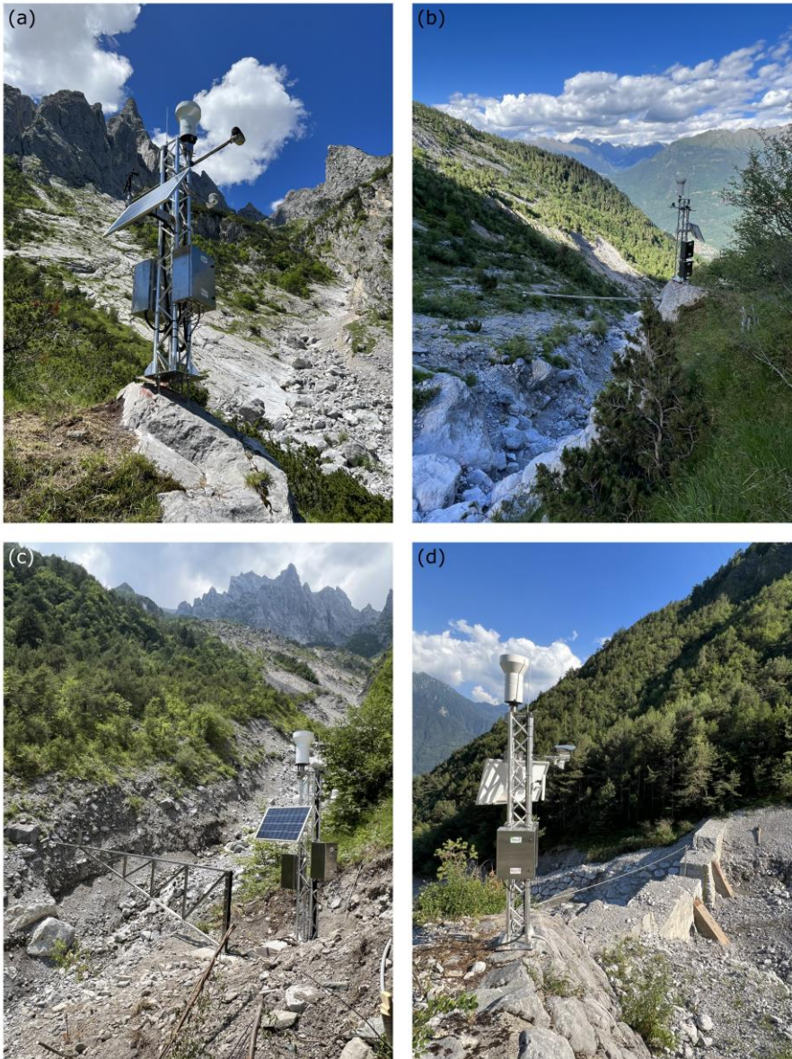
Figure 5: Photos of the four uppermost stations of Hortus S.r.l. network for monitoring and warning a) H1, b) H2, c) H3, d) H4.
