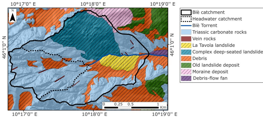
100 Figure 2: Geological map of the Blè catchment, showing lithology and deposits. The map is adapted from the Geoportal of Lombardia Region.
