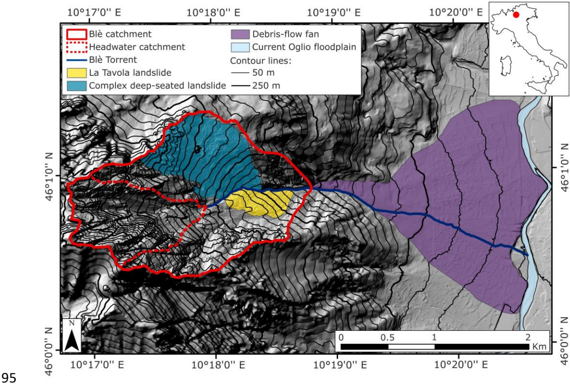
Figure 1: Map of the main geomorphological features of the Blè catchment. The base map is adapted from the Geoportal of Lombardia Region.
