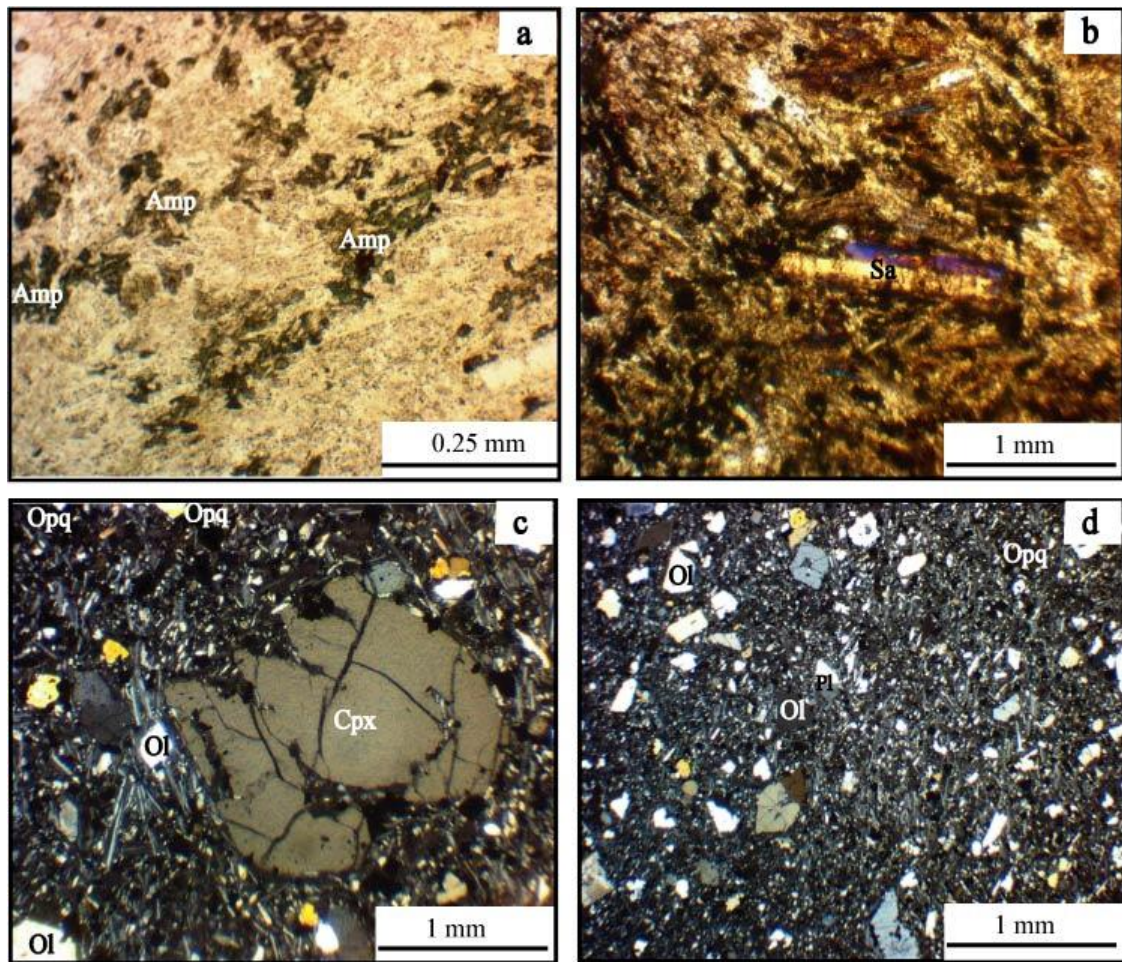
Fig. 4. Photomicrographs of thin sections of representative samples from the study area. (a) and (b) Aphyritic texture of Minawao trachyte showing mineral assemblages. (c) and (d) Porphyritic texture of Gawar basalt showing mineral assemblages. Ol: olivine. Cpx: clinopyroxene. Pl: plagioclase. Opq: opaque minerals. Sa: sanidine. Amp: amphibole. Mineral abbreviations from Whitney and Evans (2010).
