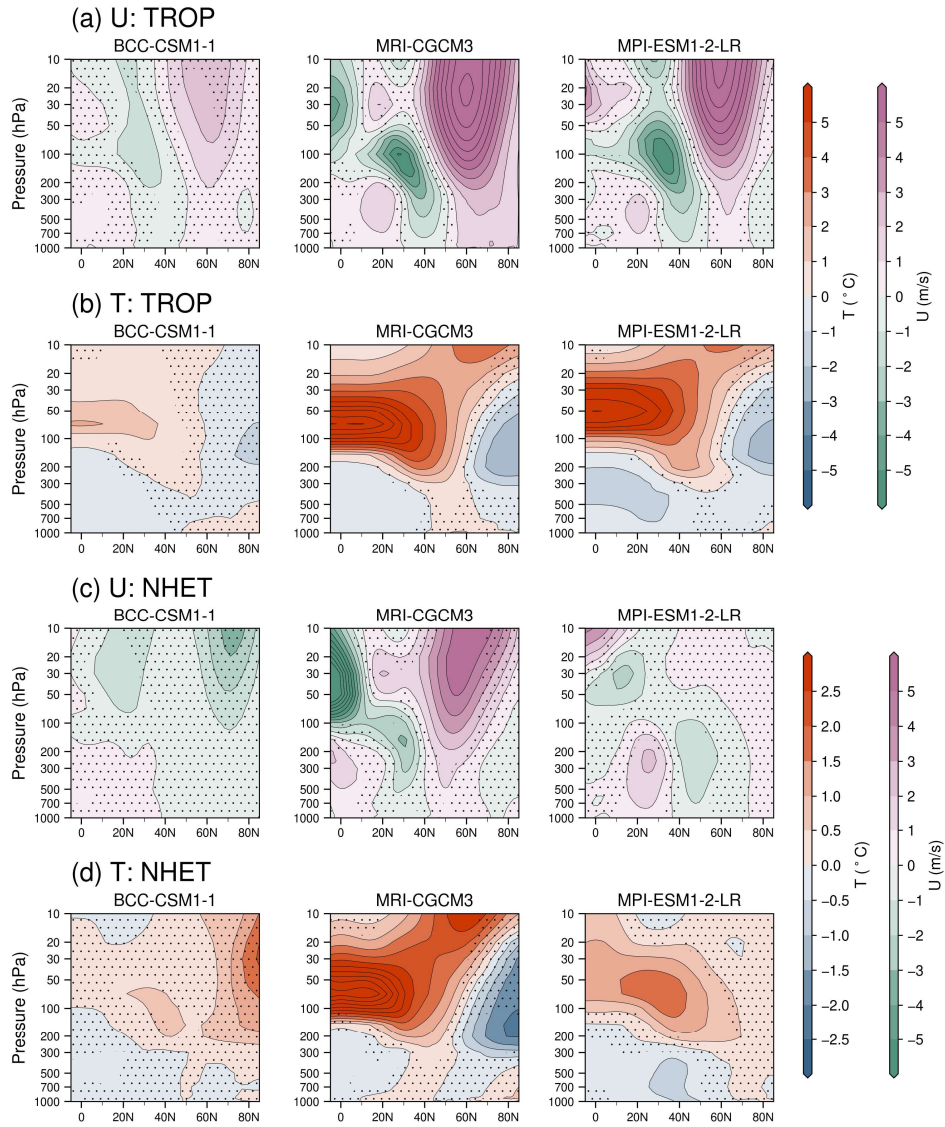
355 Figure 7. Northern Hemispheric zonal mean anomalies of (a) zonal wind ( U , unit: m/s) and (b) air temperature ( T , unit: ^{\circ}\text{C} ) from the stratosphere to the troposphere in three selected PMIP models with winter Eurasian warming responses during the first winter following TROP eruptions. (c-d) are the same as (a-b) but for NHET eruptions. Anomalies are computed relative to the average of five years before the eruptions. Black dots indicate regions where anomalies are not statistically significant at the 95% confidence level.
