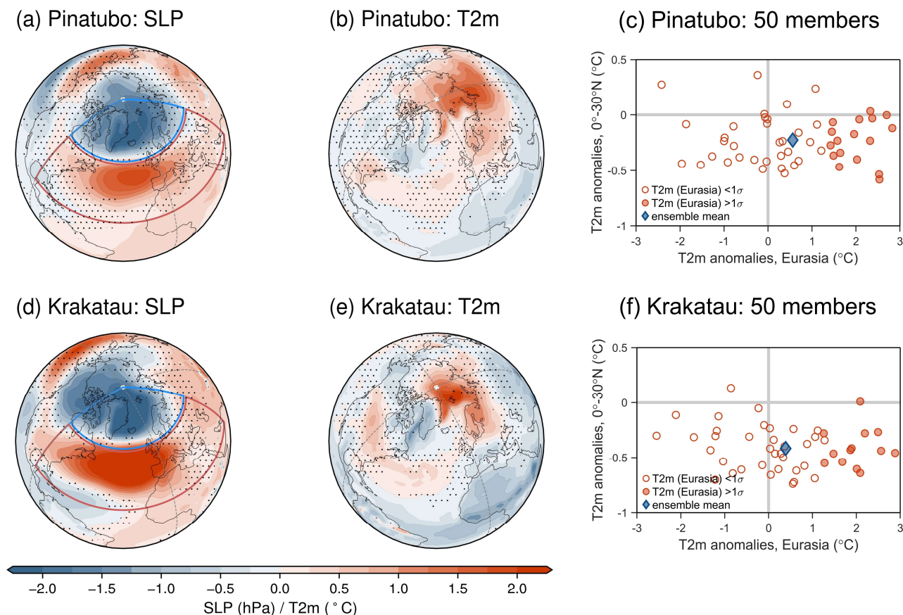
375 Figure 8. (a) Sea level pressure (SLP) and (b) near-surface air temperature (T2m) anomalies in the 50-member ensemble mean of the MPI-ESM1-2-LR historical simulation after the 1991 Pinatubo eruption. Black dots indicate regions where less than 30 members agree on the sign of the anomalies. (c) T2m anomalies over 0°–30°N and northern Eurasia (55°N–70°N, 10°E–120°E) relative to the mean of the historical simulation period (1850–2014), with red circles denoting individual members and the blue diamond denoting the ensemble mean. T2m 380 anomalies over northern Eurasia exceeding one standard deviation ( \sigma ) are filled with color. Panels (d–f) are the same as (a–c) but for the 1883 Krakatau eruption.
