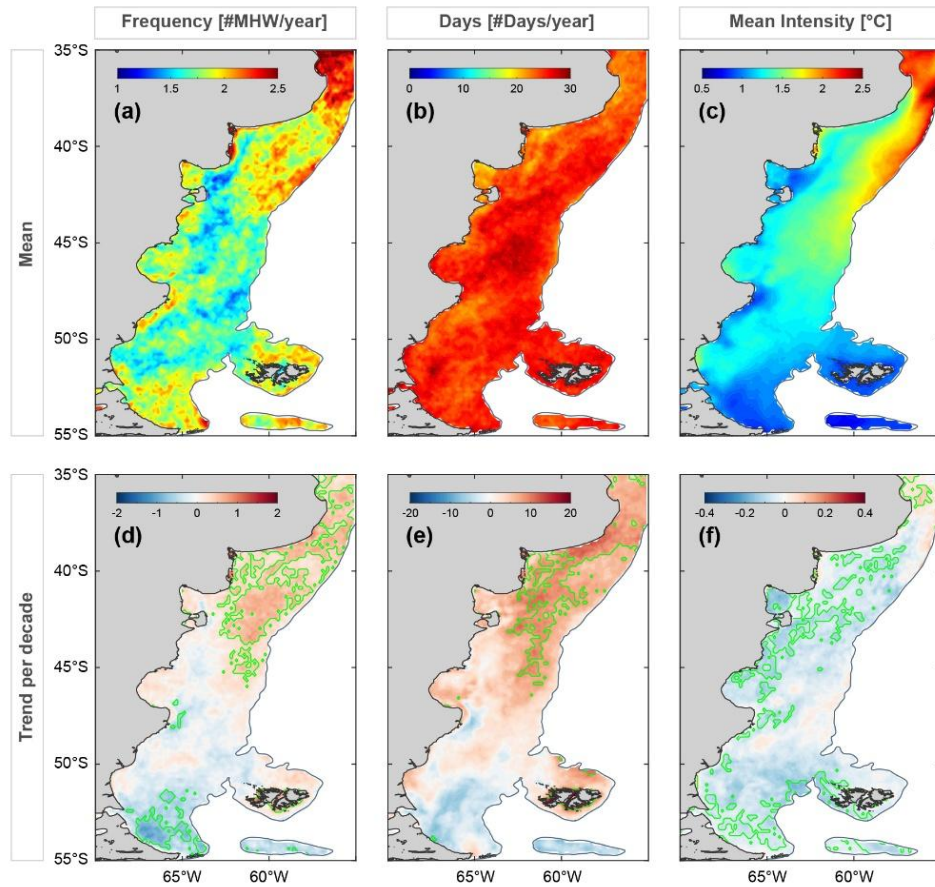
270 Figure 4: a) Mean frequency, b) number of cumulative days, and c) intensity of MHWs in the PS. Corresponding trends are shown in d), e), and f) (values decade -1 ). Areas in green indicate statistically significant trends ( p < 0.05 ).
