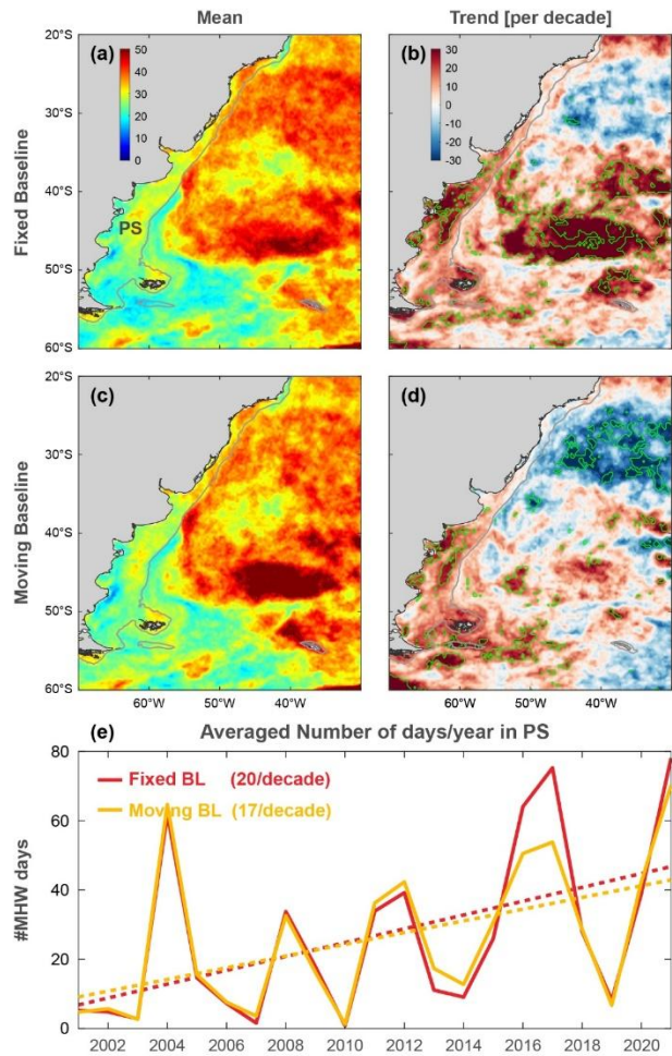
Figure 2: Comparison of two baseline methodologies (FB and MB) for the detection of MHWs in the PS. (a) Mean number of days per year of MHWs and (b) trend of the number of days by decade of MHWs using the fixed baseline approach. (c) Mean number of days by year of MHWs and (d) trend of number of days by decade of MHWs using the moving baseline approach. (e) Comparison of both methodologies on the interannual variability of the mean number of days in the PS. Delimited green areas stand for a statistically significant trend ( p < 0.05 ).
