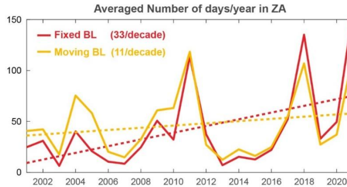
Figure B1: Comparison of both methodologies on the interannual variability of the mean number of days in the ZA.
