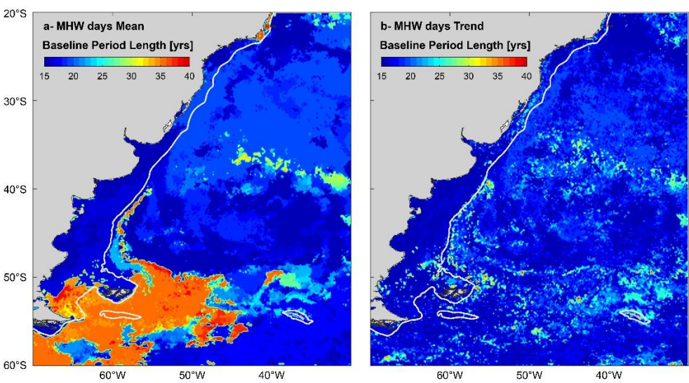
Figure B3. Length of the Baseline period [in years], when the 1982-2021 mean (a) and trend (b) MHWs days is maximum.
