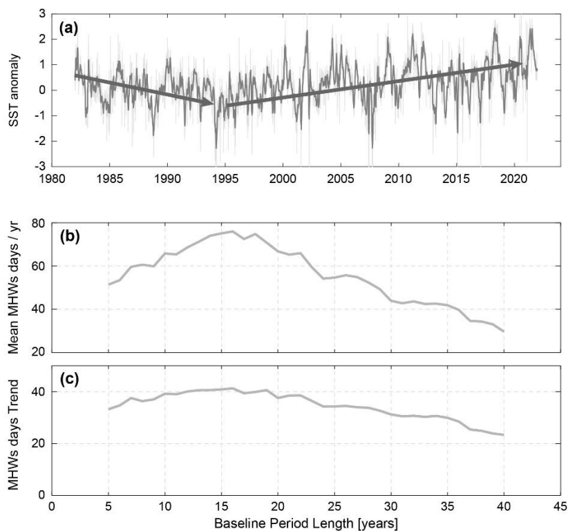
Figure B2: (a) SST anomaly (°C) in the Zapiola anticyclone. (b) Number of MHW days year -1 (averaged over 1982-2021) for different baseline period lengths (in years) ranging from 5 to 40 years (starting in 1982). (c) same as (b) for the trend in MHWs days [#days yr -1 decade -1 ].
