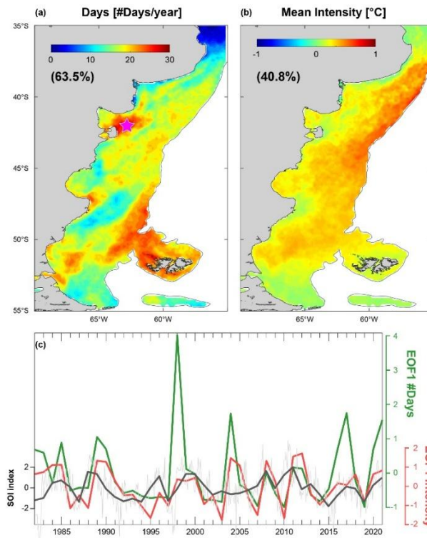
335 Figure 6: Spatial patterns of the first EOF modes of the interannual variability in (a) number of days, (b) mean intensity and (c) the corresponding time series of expansion coefficients overlaid on monthly (grey) and annual mean (black) SOI index. El Niño (La Niña) phases correspond to negative (positive) SOI indexes.
