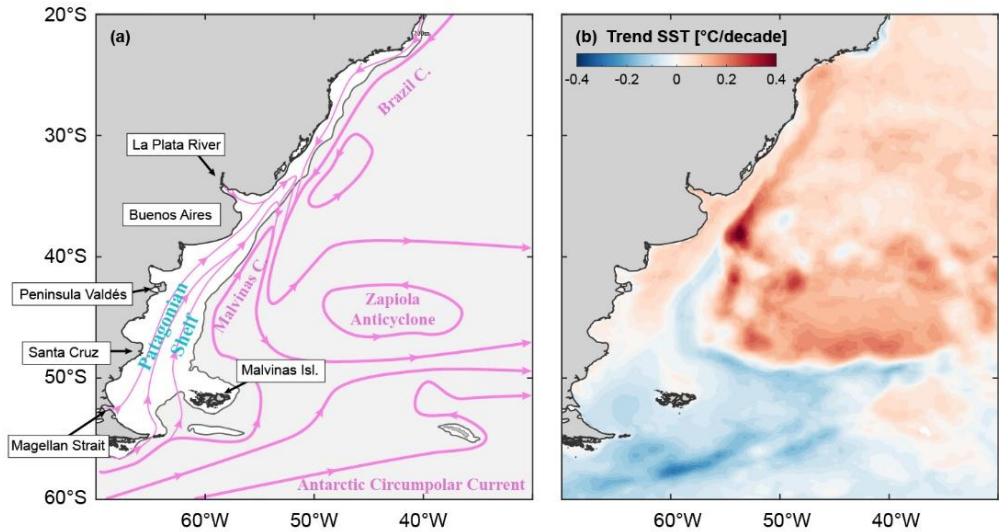
Figure 1: (a) General circulation patterns and oceanographic characteristics of the Southwestern Atlantic Ocean (SWA). The grey line, corresponding to the 200 m isobath, delimits the Patagonian Shelf (PS). (b) SST trend ( ^{\circ}\text{C decade}^{-1} ) in the region for the period 1980 to 2021.
