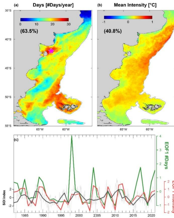
Figure 6: Spatial patterns of the first EOF modes of the interannual variability in (a) number of days, (b) mean intensity and (c) the corresponding time series of expansion coefficients overlaid on monthly (grey) and annual mean (black) SOI index. El Niño (la Niña) phases correspond to negative (positive) SOI indexes.
