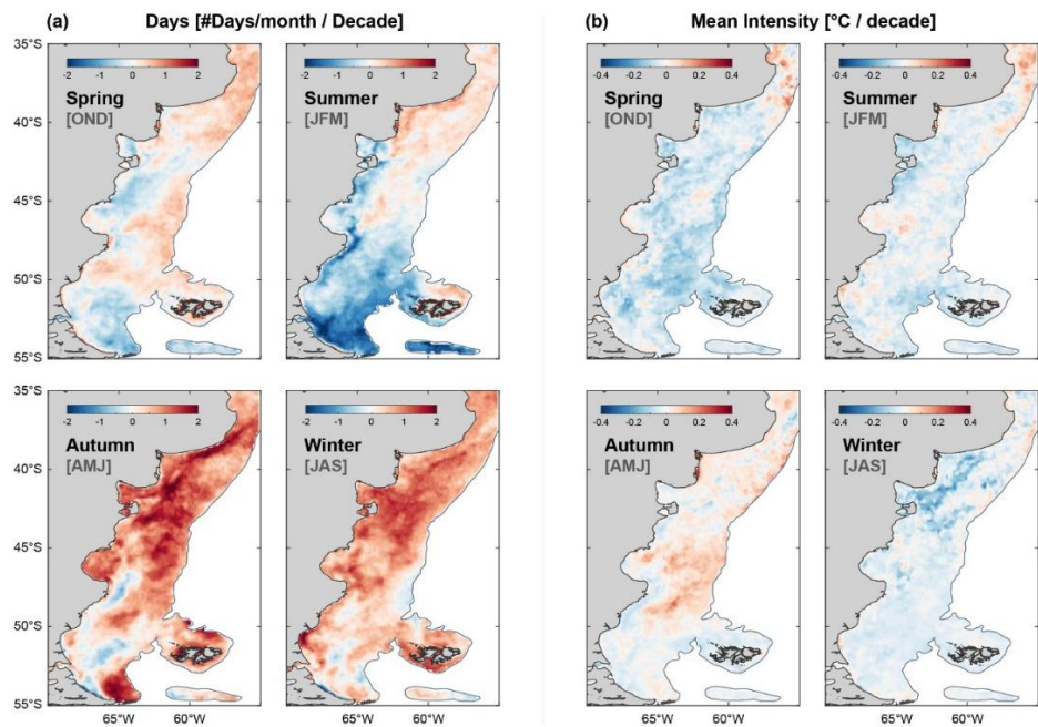
Figure D1. Seasonal Marine Heatwaves trends in number of days month -1 decade -1 and mean intensity (°C decade -1 ).
