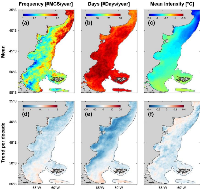
415 Figure C1. Marine Cold Spells in the Patagonian Continental Shelf. Mean frequency (a), number of days (b), intensity (c); trend per decade of frequency (d), number of days (e), intensity (f).
