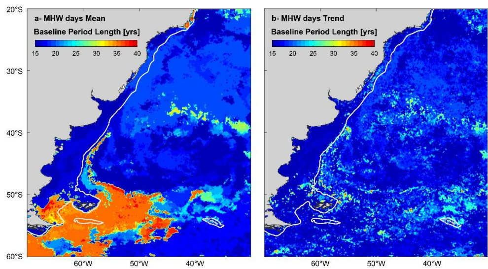
Figure B4. Length of the Baseline period [in years], when the 1982-2021 mean (a) and trend (b) MHWs days is maximum.
