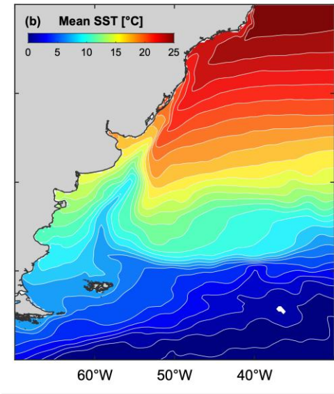
Figure A1: Mean sea surface temperature (SST, °C).
