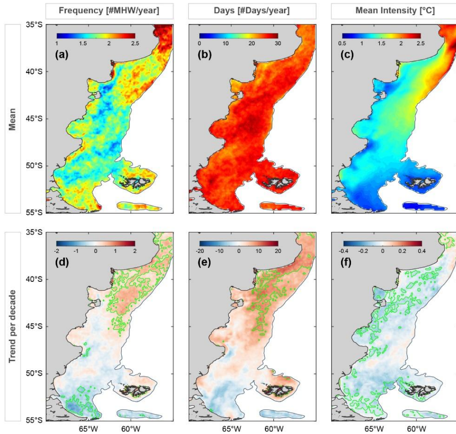
Figure 4: a) Mean frequency, b) number of cumulative days, and c) intensity of MHWs in the PS. Corresponding trends are shown in d), e), and f) (values decade -1 ). Areas in green indicate statistically significant trends ( p < 0.05 ).
