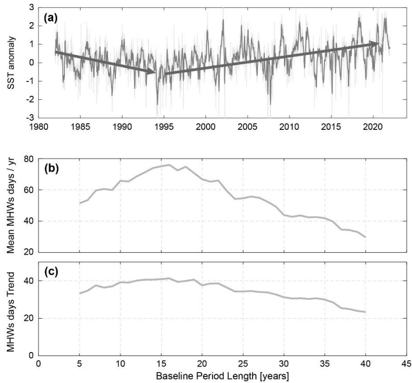
395 Figure B3: (a) SST anomaly (°C) in the Zapiola anticyclone. (b) Number of MHW days year -1 (averaged over 1982-2021) for different baseline period lengths (in years) ranging from 5 to 40 years (starting in 1982). (c) same as (b) for the trend in MHWs days [#days yr -1 decade -1 ].
