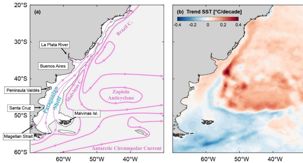
Figure 1: (a) General circulation patterns and oceanographic characteristics of the Southwestern Atlantic Ocean (SWA). The grey line, corresponding to the 200 m isobath, delimits the Patagonian Shelf (PS). (b) SST trend ( ^{\circ}\text{C decade}^{-1} ) in the region for the period 1980 to 2021.
