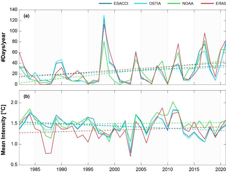
Figure 3: Dataset comparison for MHWs assessment in the PS. (a) Interannual variability in the number of MHWs days year -1 . (b) Mean annual MHW intensity. Dotted lines represent the linear fits to each corresponding dataset (see Table B2 for statistics).
