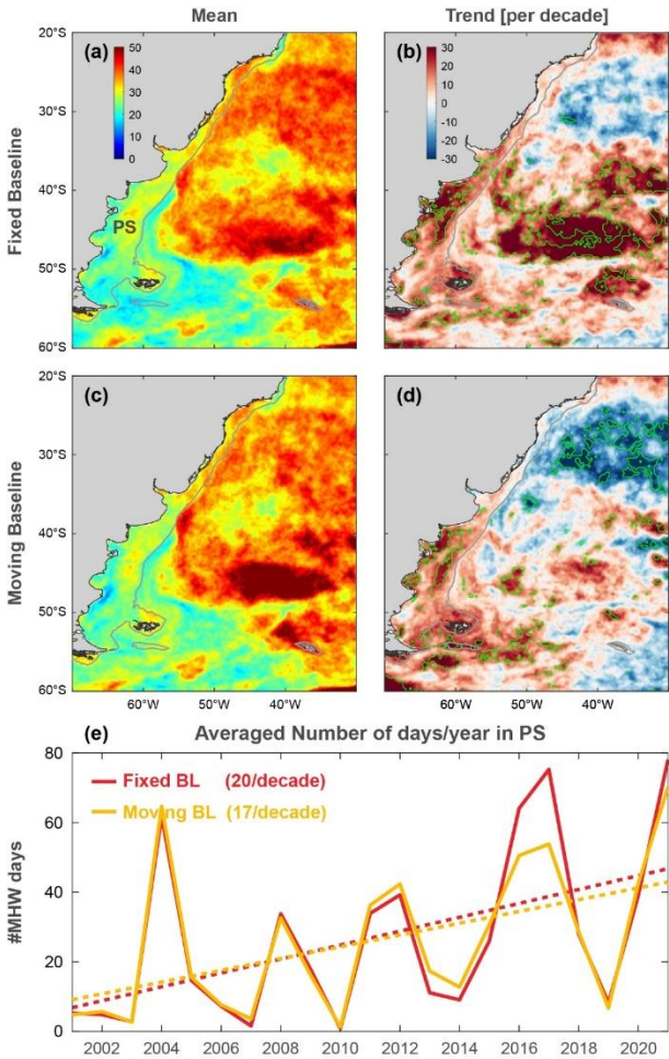
215 Figure 2: Comparison of two baseline methodologies (FB and MB) for the detection of MHWs in the PS. (a) Mean number of days per year of MHWs and (b) trend of the number of days by decade of MHWs using the fixed baseline approach. (c) Mean number of days by year of MHWs and (d) trend of number of days by decade of MHWs using the moving baseline approach. (e) Comparison of both methodologies on the interannual variability of the mean number of days in the PS. Delimited green areas stand for a statistically significant trend ( p < 0.05 ).
