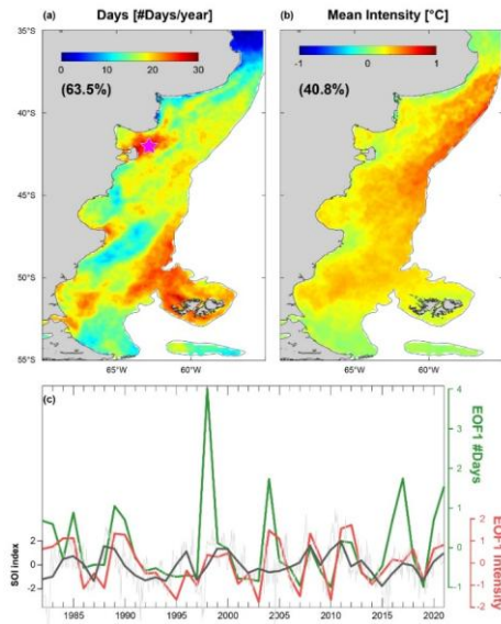
Figure 6: Spatial patterns of the first EOF modes of the interannual variability in (a) number of days, (b) mean intensity and (c) the corresponding time series of expansion coefficients overlaid on monthly (grey) and annual mean (black) SOI index. El Niño (la Niña) phases correspond to negative (positive) SOI indexes.
