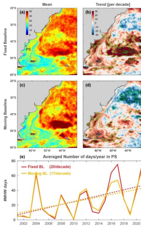
220 Figure 2: Comparison of two baseline methodologies (FB and MB) for the detection of MHWs in the PS. (a) Mean number of days per year of MHWs and (b) trend of the number of days by decade of MHWs using the fixed baseline approach. (c) Mean number of days by year of MHWs and (d) trend of number of days by decade of MHWs using the moving baseline approach. (e) Comparison of both methodologies on the interannual variability of the mean number of days in the PS. Delimited green areas stand for a statistically significant trend ( p < 0.05 ).
