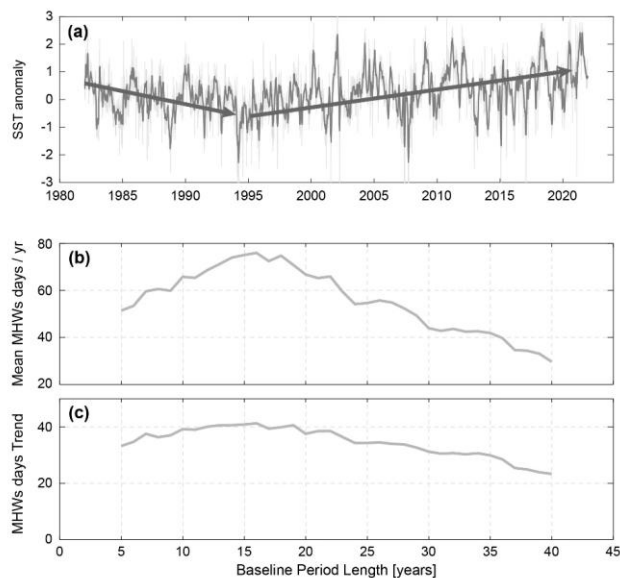
Figure B3: (a) SST anomaly (°C) in the Zapiola anticyclone. (b) Number of MHW days year -1 (averaged over 1982-2021) for different baseline period lengths (in years) ranging from 5 to 40 years (starting in 1982). (c) same as (b) for the trend in MHWs days [#days yr -1 decade -1 ].
