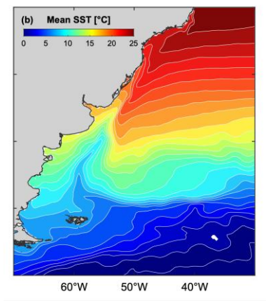
Figure A1: Mean sea surface temperature (SST, °C).
