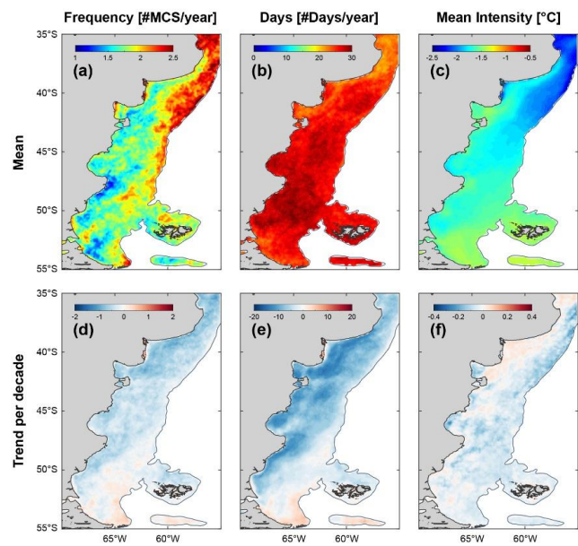
Figure C4C5. Marine Cold Spells in the Patagonian Continental Shelf. Mean frequency (a), number of days (b), intensity (c); trend per decade of frequency (d), number of days (e), intensity (f).
