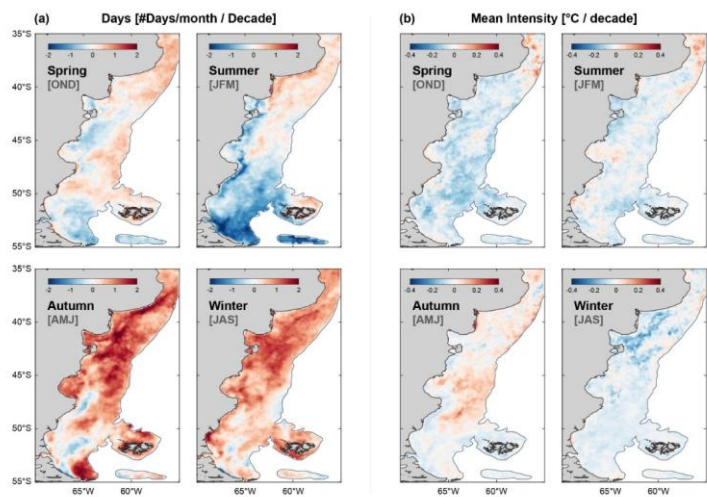
430 Figure D64. Seasonal Marine Heatwaves trends in number of days month -1 decade -1 and mean intensity (°C decade -1 ).
