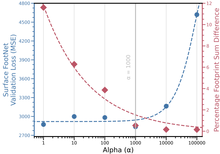
Figure 4. Trade-off between validation loss (mean squared error; MSE) and percentage footprint mass difference for different values of \alpha in the surface FootNet model.
