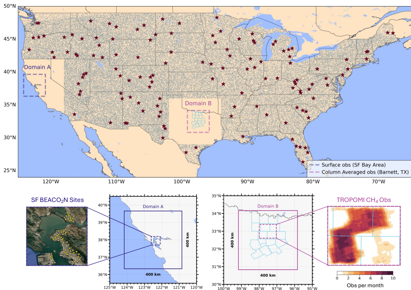
Figure 2. (Top panel) Receptors for training out-of-sample FootNet. Gray dots indicate individual receptors sampled uniformly across CONUS. Red stars show centers of 400×400 km 2 subdomains with enhanced temporal sampling. Domains A and B are withheld in the out-of-sample training configuration. Supplemental Figure S1 shows the full training data used for the in-sample FootNet model. Bottom row shows the observational networks used in both case studies. Background satellite imagery is taken from Google Maps.
