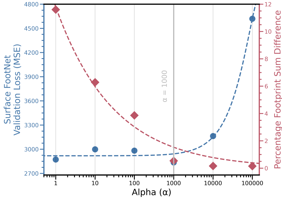
Figure 4. Trade-off between validation loss (mean squared error; MSE) and percentage footprint mass sum difference for different values of \alpha in the surface FootNet model.
