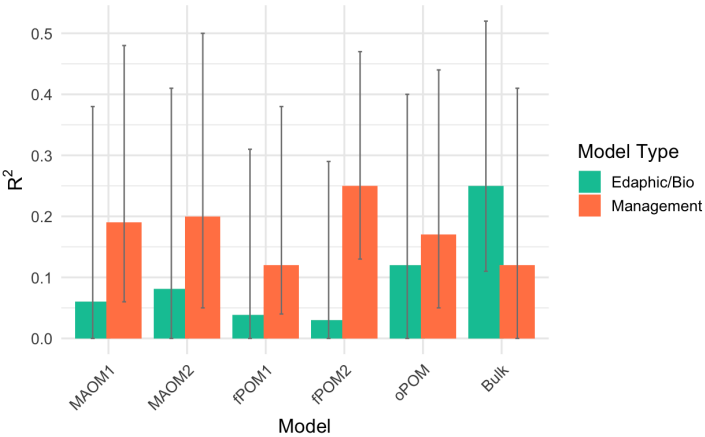
Figure 3: Marginal R 2 values for edaphic/biological variable groupings and management variables. 95% confidence intervals derived from parametric bootstrapping (1000 iterations; 'partR2' package in R). For all models, the edaphic/biological grouping includes soil physical PC1 (texture, CEC), soil iron PC1, and pH; for the MAOM2 model, this
