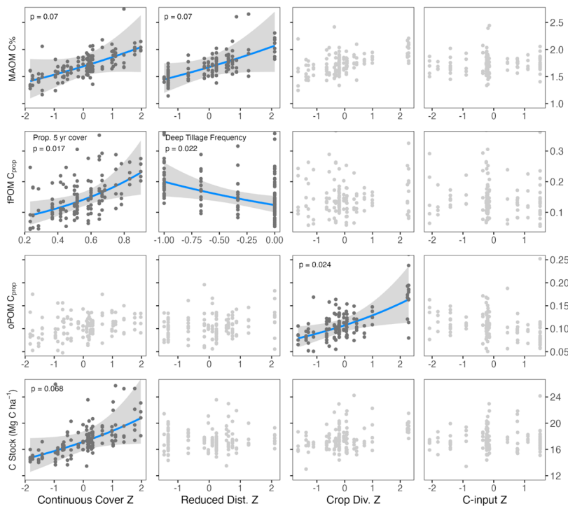
Figure 2: Modeled regressions for carbon fraction and stock models. Models hold all other variables constant at mean values. Significant relationships are darker with p-values listed. Unless otherwise indicated, x-axis uses z-scores for each management category. MAOM results visualize MAOM 2 model.
