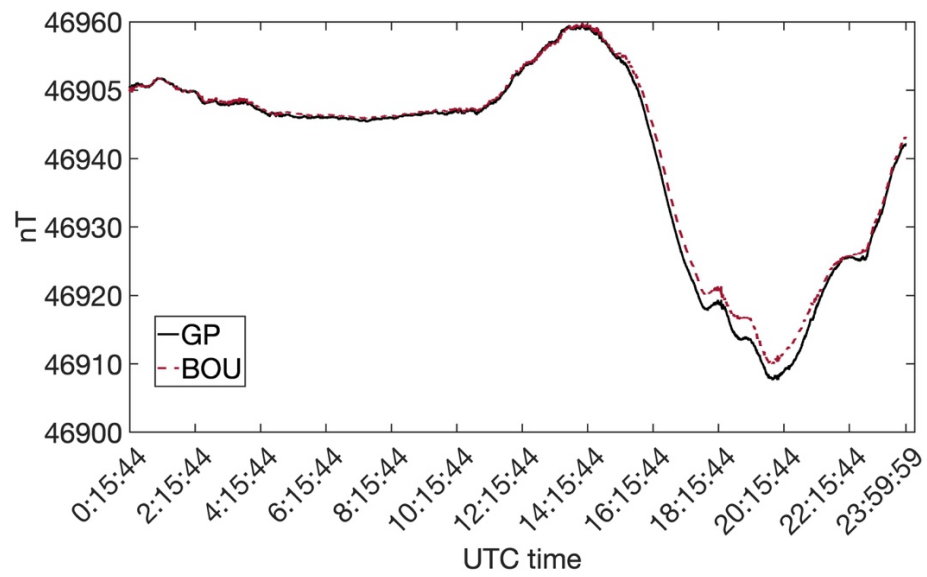
Figure 9f, with the magnetic field values shown in nT instead of microTesla.
