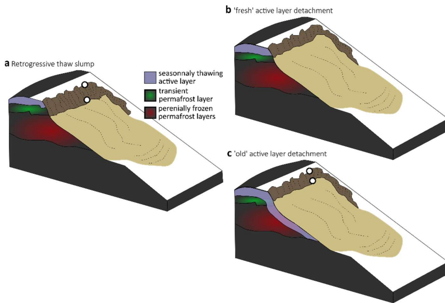
425 Figure 9: Conceptual model of materials exposed by hillslope thermokarst structures and mineral-organic carbon (OC) interactions in surface and deep samples. (a) an active retrogressive thaw slump, whose headwall exposes fresh material every summer; (b) a 'fresh' active layer detachment, i.e. in the days/months following its formation; (c) an "old" active layer detachment, i.e. several years after its formation and whose headwall has undergone freeze/thaw cycles for several years. The white dots on the outcrops (a) and (c) represent the sampling depths of the top and bottom samples.
