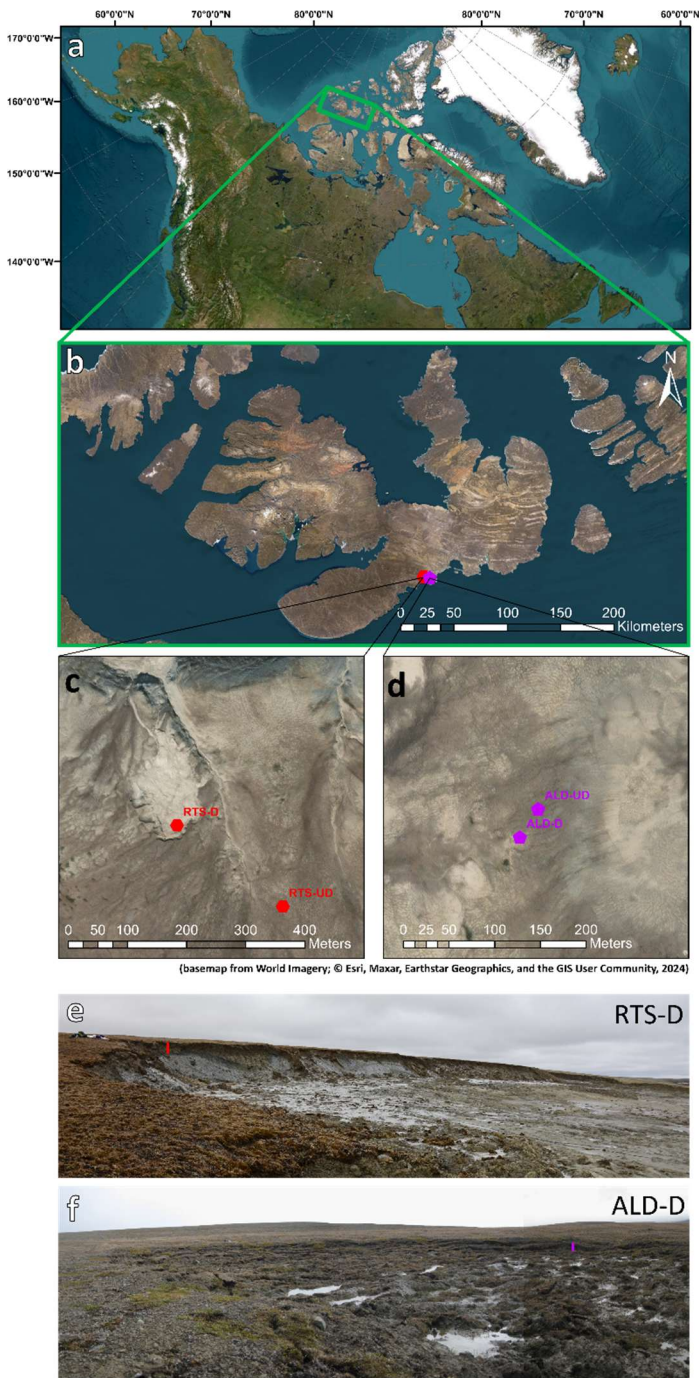
140 Figure 3: Study site and sampling location. (a) Location of the Melville Island; (b) Location of the Cape Bounty Arctic Watershed 145 Observatory (CBAWO), on the south-central coast of the Melville Island; (c-d) Locations of the sampled profiles. RTS = retrogressive thaw slump; ALD = active layer detachment; D = disturbed; UD = undisturbed; (e-f) Photographs and profile locations of the disturbed sites at the time of sampling for the RTS-D (e) and the ALD-D (f). Profile locations on panels (e) and (f) are represented by colored vertical rectangles. Map created in ArcMap® 10.8. Basemap source: World Imagery (Esri et al., 2024). Photos from panels e-f: M. Lafrenière, J. Heslop.
