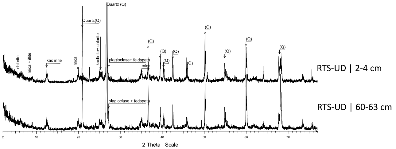
555 Figure C. 2: Diffractograms for Cape Bounty thaw slump in the undisturbed profile (RTS-UD).
