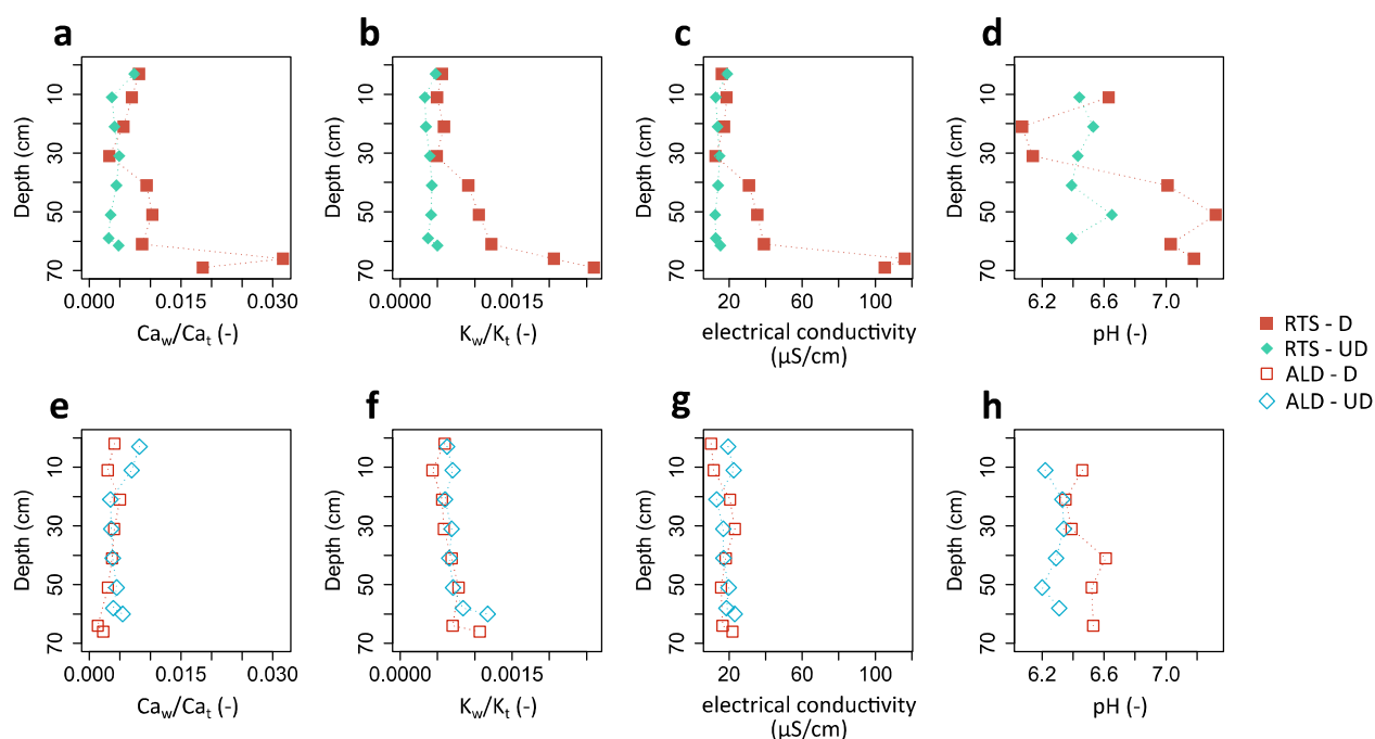
260 Figure 5: Results of water extraction measurements for (a,e) the ratio between water extracted (w) and total (t) concentrations in calcium ( Ca_w/Ca_t ), (b,f) the ratio between water extracted (w) and total (t) concentrations in potassium ( K_w/K_t ), (c,g) electrical conductivity and (d,h) pH. RTS = retrogressive thaw slump; ALD = active layer detachment; D = disturbed; UD = undisturbed.
