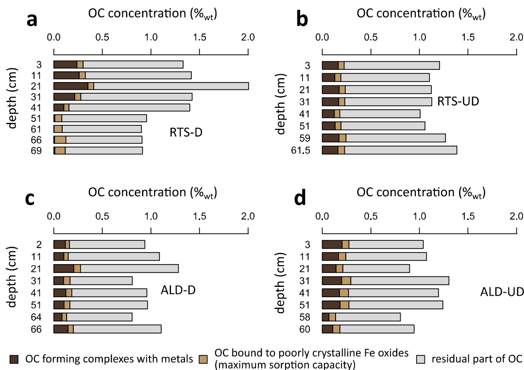
320 Figure 7: Evolution with depth of pyrophosphate-extracted carbon ( C_p ) and maximum proportion of organic carbon (OC) bound to poorly crystalline Fe oxides ( C_{amorph} ) in (a) sediments exposed by the retrogressive thaw slump (RTS-D); (b) the corresponding undisturbed profile (RTS-UD); (c) sediments exposed by the active layer detachment (ALD-D); (d) the corresponding undisturbed profile (ALD-UD). The values of OC bound to crystalline Fe oxides correspond to a calculation with a maximum sorption capacity of 0.22 \text{ g}_{OC}/\text{g}_{Fe} as ferrihydrite ( Fe_o-Fe_p ). %wt = mass of OC as a percentage of the total mass of dry soil, i.e., weight percent.
