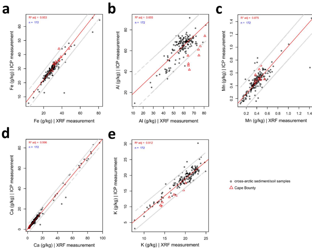
535 Figure A. 1: Total concentrations in Fe (a), Al (b), Mn (c), Ca (d) and K (e) measured by inductively coupled plasma optical-emission spectrometry (ICP-OES) as a function of those measured by the portable X-ray fluorescence (pXRF). Cross-arctic measurements include data from the yedoma domain (Monhonval et al., 2021b) and include samples from Khardang Island (n = 1), Kurungnakh Island (n = 2), Sobo sise Island (n = 58), Bykovsky peninsula (n = 2), Buor Khaya peninsula (n = 44), Stolbovoy Island (n = 1), Bol'shoy lyakhovsky Island (n = 3), Oyogos Yar coast (n = 1), Kytalyk (n = 4), Duvanny Yar (n = 5), Yukechi (n = 2), Kitluk (n = 2), Baldwin peninsula (n = 1), Colville (n = 8) and Itkilik (n = 10). Other samples originate from Zackenberg (n = 4) (Opfergelt et al., 2018), Peel Plateau (n = 3) (Thomas et al., 2023), Batagay (n = 14) (Thomas et al., 2024) and from Cape Bounty (n = 8; this study). 95% prediction intervals are presented in grey. 540
