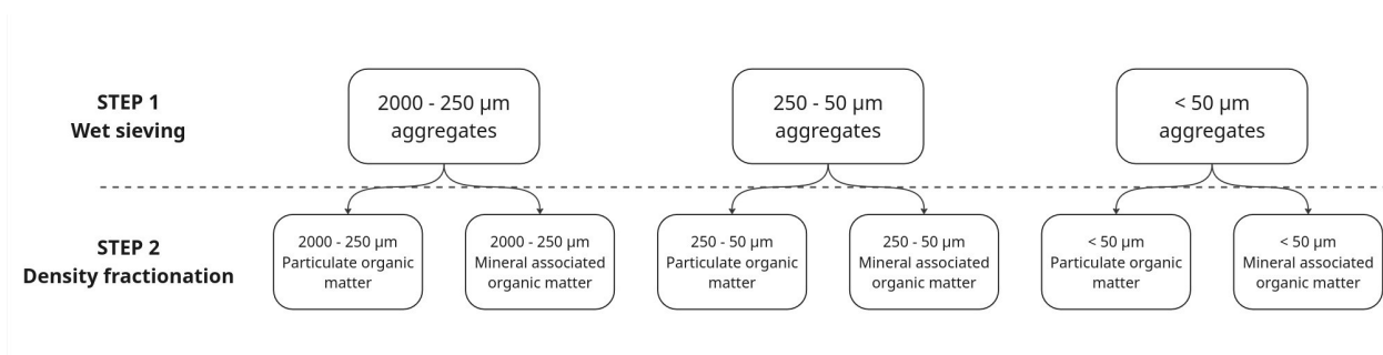
Figure 4: Two-stage aggregate and density fractionation protocol (adapted from Burgeon et al., 2021).
