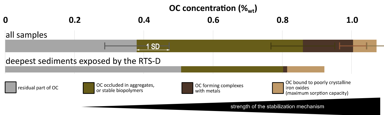
510 Figure 10: Individual organic carbon (OC) pools at Cape Bounty. Average concentrations and standard deviations (SD) of the physically and chemically extracted OC pools on all samples (n=8) compared to the deepest sediments exposed by the retrogressive thaw slump (RTS-D). The color-coding of the OC targeted pools matches those of the selective extractions shown in Fig. 2.
