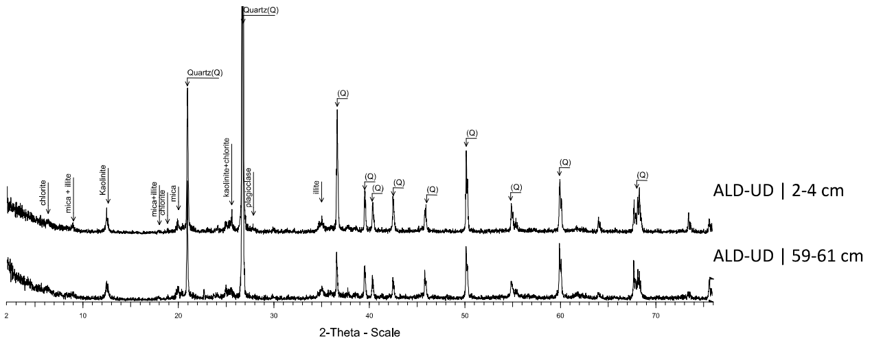
560 Figure C. 4: Diffractograms for Cape Bounty active layer detachment in the undisturbed profile (ALD-UD).
