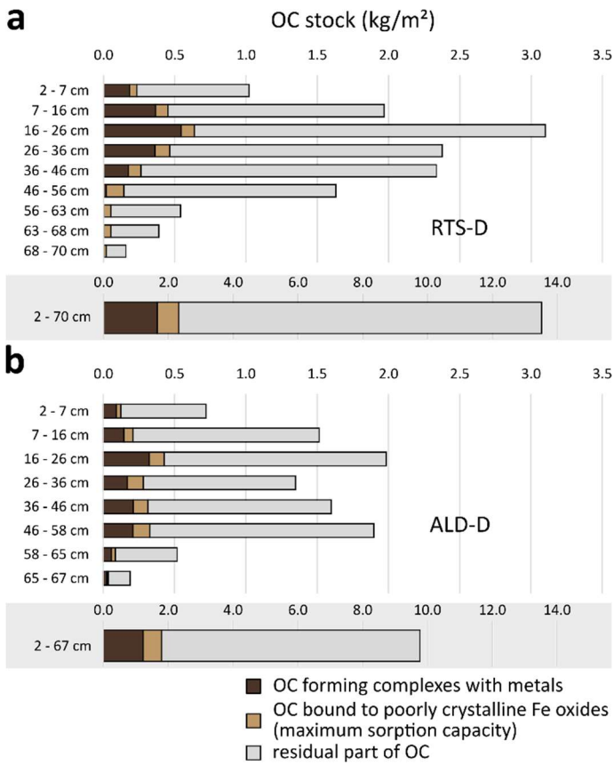
610 | Figure D. 8: Evolution with depth of the stock of pyrophosphate-extracted carbon ( C_p ) and maximum proportion of organic carbon (OC) bound to poorly crystalline Fe oxides ( C_{amorph} ) in (a) sediments exposed by the retrogressive thaw slump (RTS-D); (b) sediments exposed by the active layer detachment (ALD-D); Stocks are estimated by assuming an excess ice content of 50% for depths \geq 60 cm (Lamhonwah et al., 2016) and dry bulk densities of 1.53 g/cm 3 for depths of 0–7 cm, 1.55 g/cm 3 for depths of 7–26 cm, 1.67 g/cm 3 for depths of 26–46 cm, and 1.71 g/cm 3 for depths greater than 46 cm (Stanton, 2023). OC concentrations as in Figure 7 Fig-7 . The bars with the gray background represent the integral over the entire depth.
