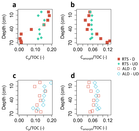
Figure D. 6: Evolution with depth of the proportion of pyrophosphate-extracted carbon relative to the total ( C_p/\text{TOC} ) and maximum proportion of organic carbon (OC) bound to poorly crystalline Fe oxides, relative to the total ( C_{\text{amorph}}/\text{TOC} ) for (a-b) sediments exposed by the retrogressive thaw slump (RTS-D) and the corresponding undisturbed profile (RTS-UD); (c-d) sediments exposed by the active layer detachment (ALD-D) and the corresponding undisturbed profile (ALD-UD). The values of OC bound to crystalline Fe oxides correspond to a calculation with a maximum sorption capacity of 0.22 \text{ gOC/gFe} as ferrihydrite ( \text{Fe}_o\text{-Fe}_p ). Color code as in Fig. 5.
