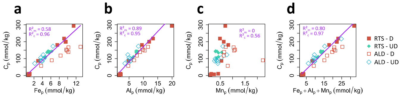
565 Figure D. 1: Robust linear regression plots between carbon extracted by pyrophosphate ( C_p ) and (a) Fe extracted by pyrophosphate ( Fe_p ); RTS = retrogressive thaw slump; ALD = active layer detachment; D = disturbed; UD = undisturbed. Color code as in Fig. 5. The variable ‘profile’ (RTS-D, RTS-UD, ALD D, ALD UD) have been included as a random factor, with random intercept and slope. The marginal R^2 ( R^2_m ), represents the population-level trend (variance explained by fixed effects). The conditional R^2 ( R^2_c ) have been included to account for both fixed and random effects and reflects total model performance.
