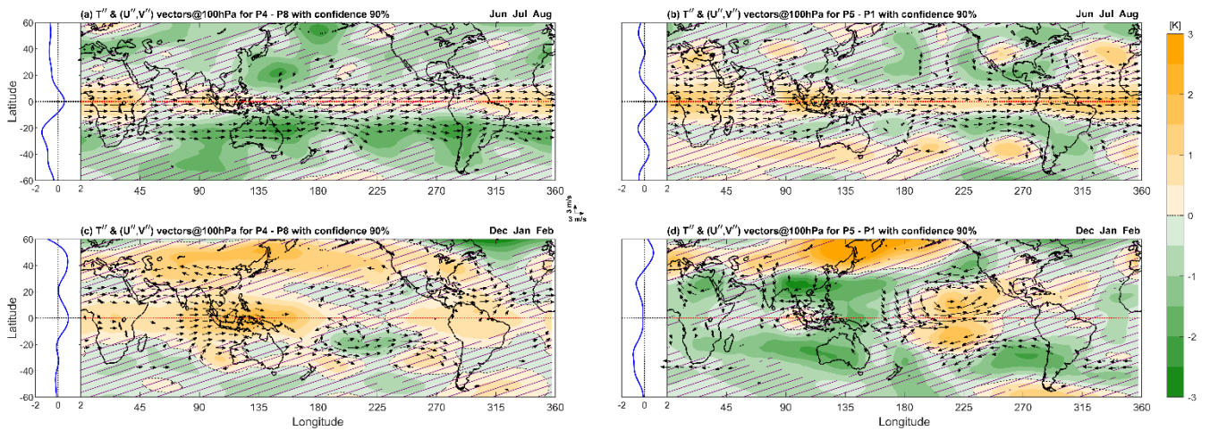
375 Figure 6. As in Fig. 5, but for temperature T'' (color bar) and wind vectors ( U'' , V'' ) at 100 hPa. The zonal mean meridional profile of QBO temperature anomaly is shown to the left of each panel.
