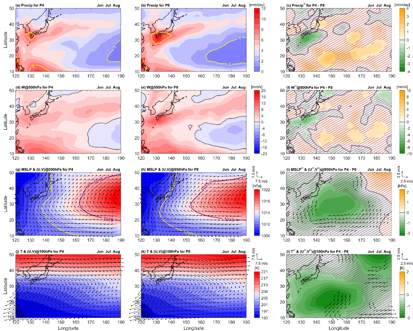
440 Figure 7. QBO regional teleconnection manifestation in the Northwest Pacific (10°-50°N, 120°-190°E) during boreal summer (JJA), showing composite climatologies for (left) QBO W at 50 hPa (P4), (middle) QBO E at 50 hPa (P8), and (right) QBO W – E at 50 hPa (P4 –
