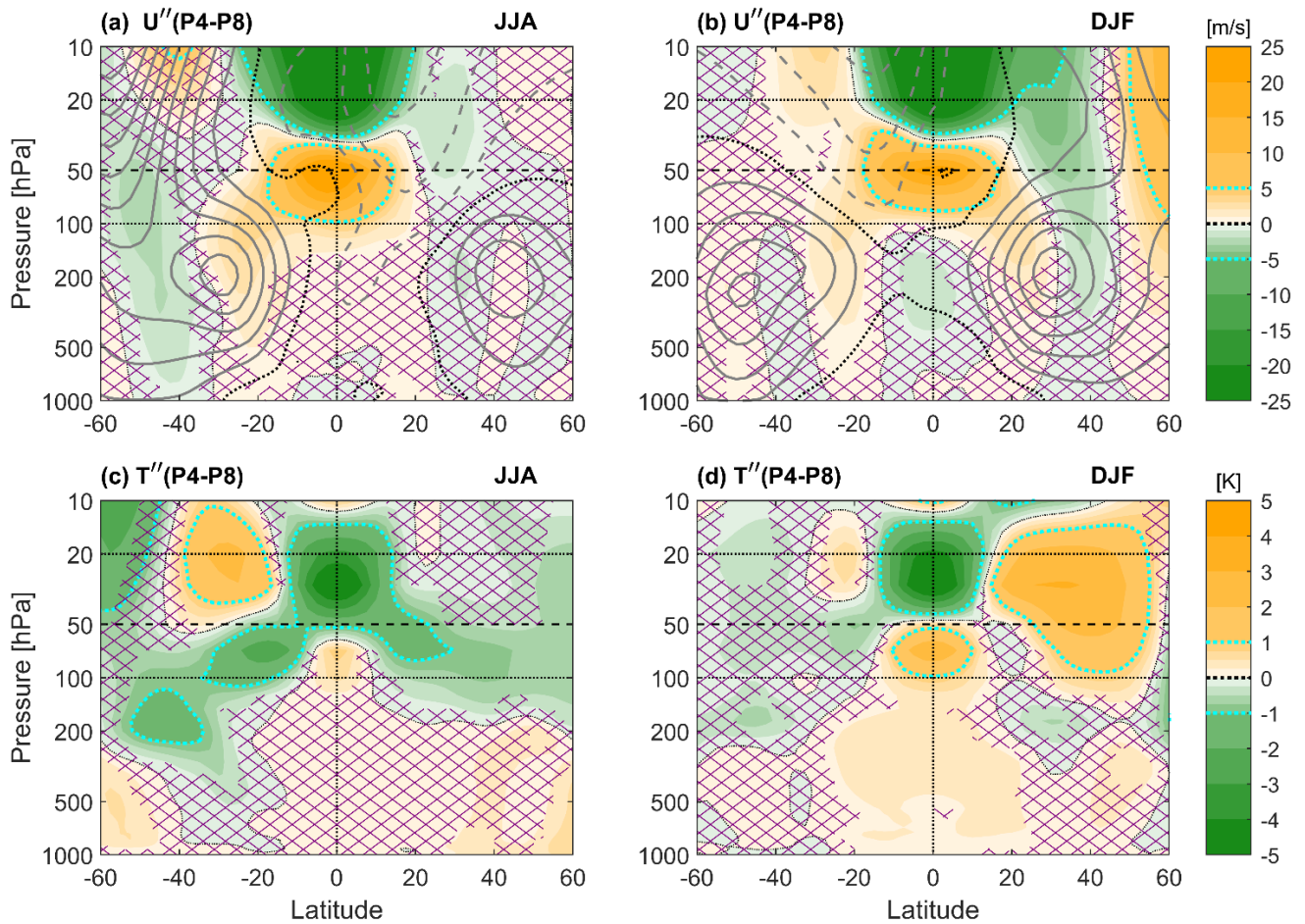
275 Figure 3. Meridional sections of the composite difference in U'' and T'' anomalies for opposing QBO phase pairs, QBO W – E at 50 hPa (P4 –P8), during DJF and JJA. Top, a–b) U'' wind anomalies. Bottom, c–d) T'' anomalies. From left to right, columns represent JJA, and DJF. The violet cross hatching indicates regions of statistical significance less than 90%. The cyan dotted line separate regions of fine and coarse contour. Horizontal lines indicate the 20 hPa (dotted), 50 hPa (dashed), and 100 hPa (dotted) levels. The climatological cycle of the U-wind for the period 1970–2020 is also shown as gray contour lines over the U'' wind anomaly panels for the respective seasons. The solid (dashed) contour lines represent the positive (negative) value, and the black dotted line is the position of the zero-wind line.
