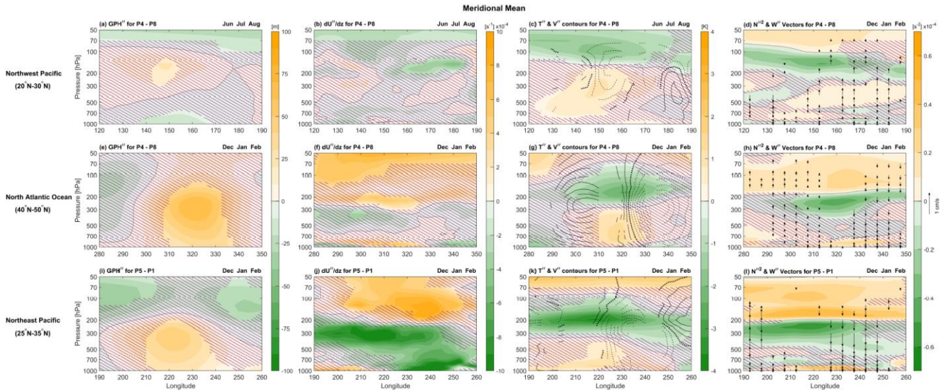
510 Figure 10. Longitude-pressure sections of composite differences between opposite QBO phases for selected latitudinal means shown in Fig 7, 8, and 9. The top row shows the latitudinal mean between 20°N and 30°N over the Northwest Pacific (120°E - 190°E) during JJA, the middle row shows the mean between 40°N and 50°N over the North Atlantic Ocean (280°E - 350°E) during DJF, and bottom row shows the mean between 25°N and 35°N over Northeast Pacific (190°E and 260°E) during DJF. The first, second, third, and fourth column of each row represent the composite difference of GPH'', vertical shear of zonal wind ( dU''/dz ), T'' (color bar) with V'' wind (contour lines at 0.5 m/s), and N''^2 with W'' wind vectors, respectively. The top two rows use QBO W - E at 50 hPa (P4 - P8), and the third uses 70 hPa indices (P5 - P1). Violet cross-hatching indicates regions of statistical significance less than 90%. The V'' contours on the 3 rd column and W'' wind arrows on the 4 th column are plotted only if either component's statistical significance exceeds the 90%. 515
