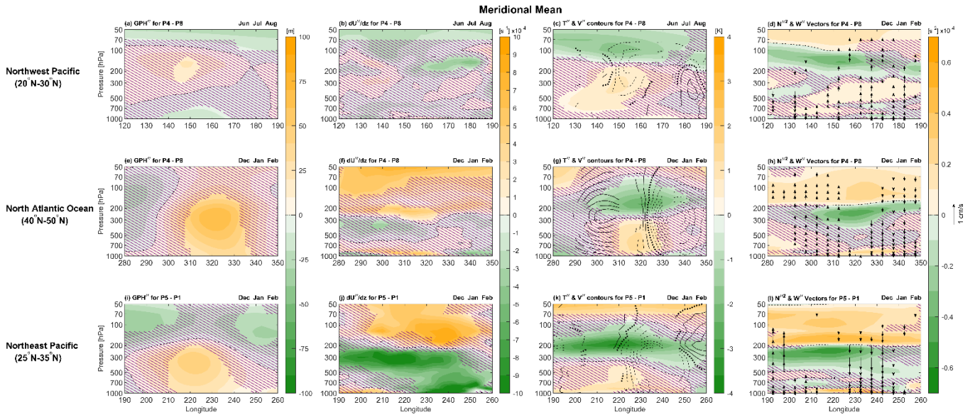
515 Figure 10. Longitude-pressure sections of composite differences between opposite QBO phases for selected latitudinal means shown in Fig. 7, 8, and 9. The top row shows the latitudinal mean between 20°N and 30°N over the Northwest Pacific (120°E - 190°E) during JJA, the middle row shows the mean between 40°N and 50°N over the North Atlantic Ocean (280°E - 350°E) during DJF, and bottom row shows the mean between 25°N and 35°N over Northeast Pacific (190° E and 260° E) during DJF. The first, second, third, and fourth column of each row represent the composite difference of GPH'', vertical shear of zonal wind ( dU''/dz ), T'' (color bar) V'' wind (contour lines at 0.5 m/s), and N''^2 with W'' wind vectors, respectively. The top two rows use QBO W - E at 50 hPa (P4 - P8), and the third uses 70 hPa indices (P5 - P1). Violet cross-hatching indicates regions of statistical significance less than 90%. The V'' contours on the 3 rd column and W'' wind arrows on the 4 th column are plotted only if either component's statistical significance exceeds the 90%.
