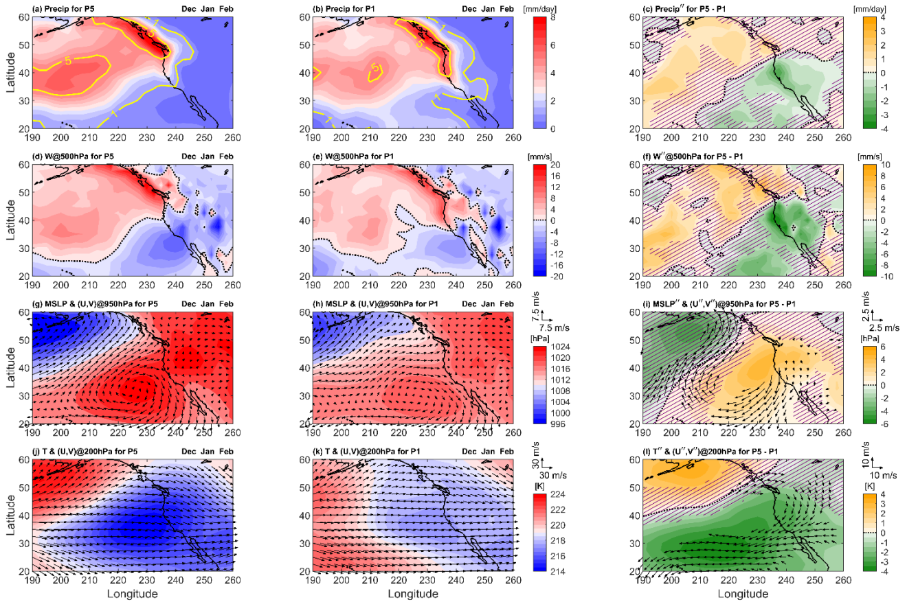
Figure 9. As in Fig. 7, but focused over the Northeast Pacific region ( 20^{\circ} - 60^{\circ} N, 190^{\circ} - 260^{\circ} E) during DJF, for QBO W and E at 70 hPa (P5 and P1).
