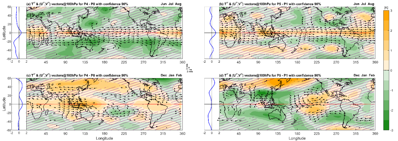
Figure 6. As in Fig. 5, but for temperature T' (color bar) and wind vectors ( U' , V' ) at 100 hPa. The zonal mean meridional profile of QBO temperature anomaly is shown to the left of each panel.
