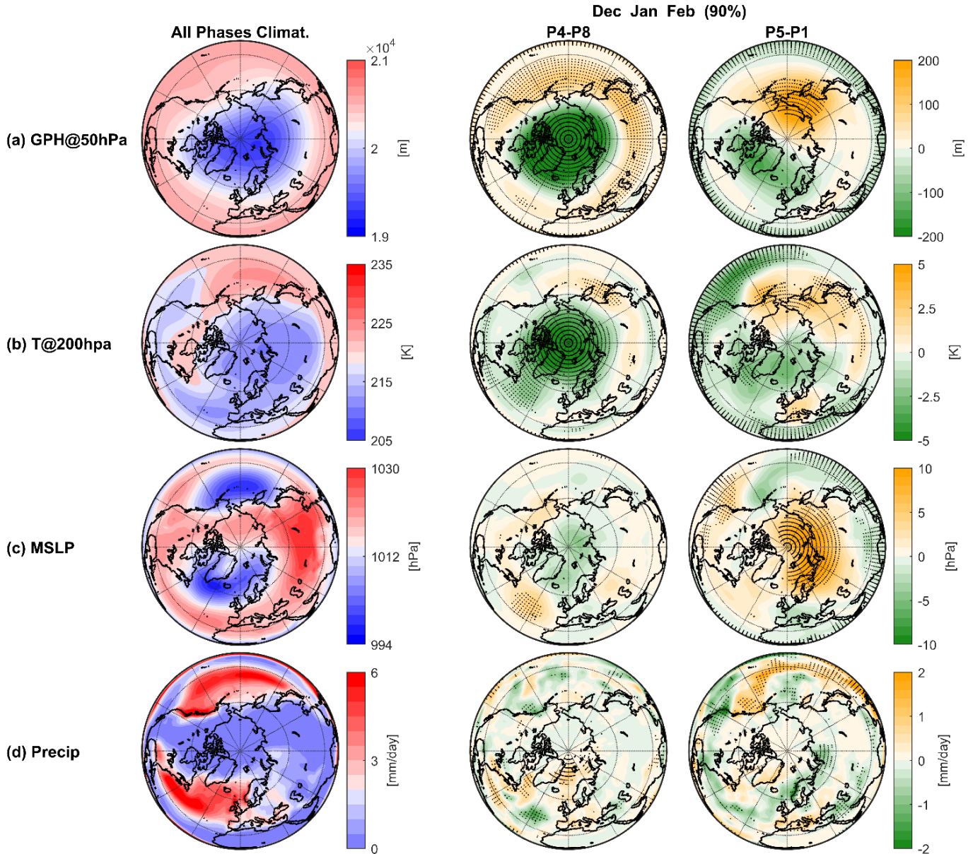
610 Figure 11. NH orthographic polar projections (10°N–90°N) of a) 50 hPa GPH, b) T at 200 hPa, c) MSLP, and d) precipitation, showing the climatology and anomalies of composite differences between QBO opposite phases during DJF and neutral ENSO. The first, second, and third, columns of each row represent the climatological mean, QBO W – E at 50 hPa (P4 – P8), and QBO W – E at 70 hPa (P5 – P1), respectively. Black dots on the both composite difference plots highlight regions where statistical significance exceeds 90%.
