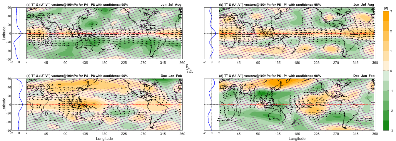
405 Figure 6. As in Fig. 5, but for temperature T'' (color bar) and wind vectors ( U'' , V'' ) at 100 hPa. The zonal mean meridional profile of QBO temperature anomaly is shown to the left of each panel.
