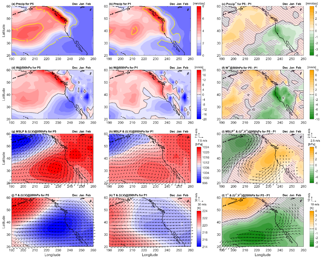
535 Figure 9. As in Fig. 7, but focused over the Northeast Pacific region (20°-60°N, 190°-260°E) during DJF, for QBO W and E at 70 hPa (P5 and P1).
