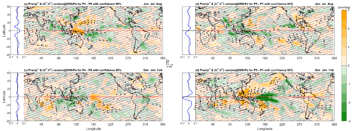
355 Figure 5. Longitude-latitude sections of QBO composite differences in precipitation (color bar) and 950 hPa horizontal winds (vector length shown in center inset) anomalies for QBO opposite phase pairs, for (a-b) JJA and (c-d) DJF. The left column represents QBO W – E at 50 hPa (P4 – P8), while the right column represents QBO W – E at 70 hPa (P5 – P1). The latitudinal profile of zonal mean precipitation is shown to the left of each panel. Wind anomalies ( U'' , V'' ) are plotted if either component’s statistical significance exceeds 90%. Violet cross-hatching indicates regions of statistical significance less than 90%.
