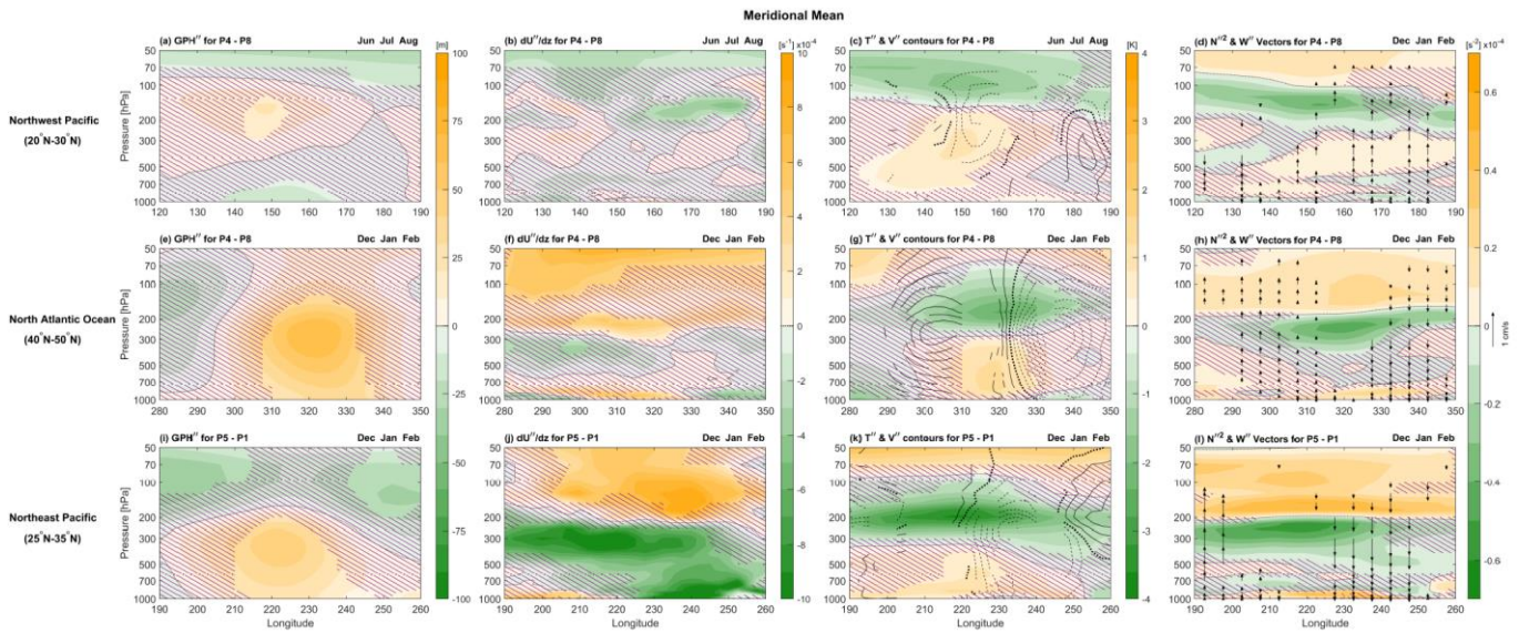
Figure 10. Longitude-pressure sections of composite differences between opposite QBO phases for selected latitudinal means shown in Fig. 7, 8, and 9. The top row shows the latitudinal mean between 20°N and 30°N over the Northwest Pacific (120°E - 190°E) during JJA, the middle row shows the mean between 40°N and 50°N over the North Atlantic Ocean (280°E - 350°E) during DJF, and bottom row shows the mean between 25°N and 35°N over Northeast Pacific (190°E and 260°E) during DJF. The first, second, third, and fourth column of each row represent the composite difference of GPH, vertical shear of zonal wind ( dU/dz ), T' (color bar) with V' wind (contour lines at 0.5 m/s), and N'' with W' wind vectors, respectively. The top two rows use QBO W - E at 50 hPa (P4 - P8), and the third uses 70 hPa indices (P5 - P1). Violet cross-hatching indicates regions of statistical significance less than 90%. The V' contours on the 3 rd column and W' wind arrows on the 4 th column are plotted only if either component's statistical significance exceeds the 90%.
