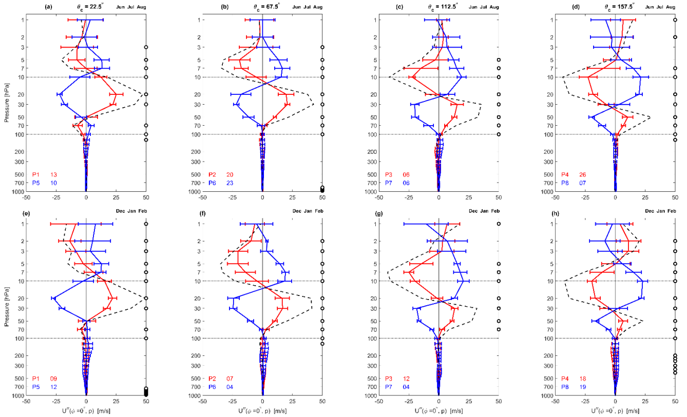
220 Figure 1. Average vertical profiles of zonal mean zonal wind U'' anomalies for each of the eight phases P1 to P4 (red) and P5 to P8 (blue), along with composite differences between these QBO opposite phases (black dashed line) for JJA (a-d) and DJF (e-h). The whiskers denote \pm one standard deviation for each composite phase, and an open circle is plotted on the right y-axis if the composite difference at that level exceeds 90% statistical significance. The total number of samples for each phase is written at the bottom left corner in each panel.
