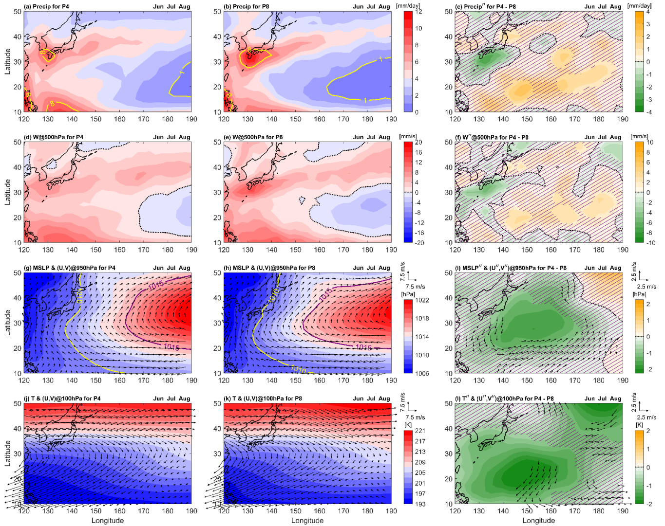
480 Figure 7. QBO regional teleconnection manifestation in the Northwest Pacific (10°-50°N, 120°-190°E) during boreal summer (JJA), showing composite climatologies for (left) QBO W at 50 hPa (P4), (middle) QBO E at 50 hPa (P8), and (right) QBO W - E at 50 hPa (P4 - P8), for (a-c) precipitation, (d-f) mid tropospheric W-wind at 500 hPa, (g-i) MSLP with (U, V) wind at 950 hPa, and (j-l) 100 hPa temperature with (U, V) wind. The violet cross hatching on the composite difference plots indicates regions of statistical significance less than 90%. Wind anomalies ( U'' , V'' ) are plotted only if either component's statistical significance exceeds 90%.
