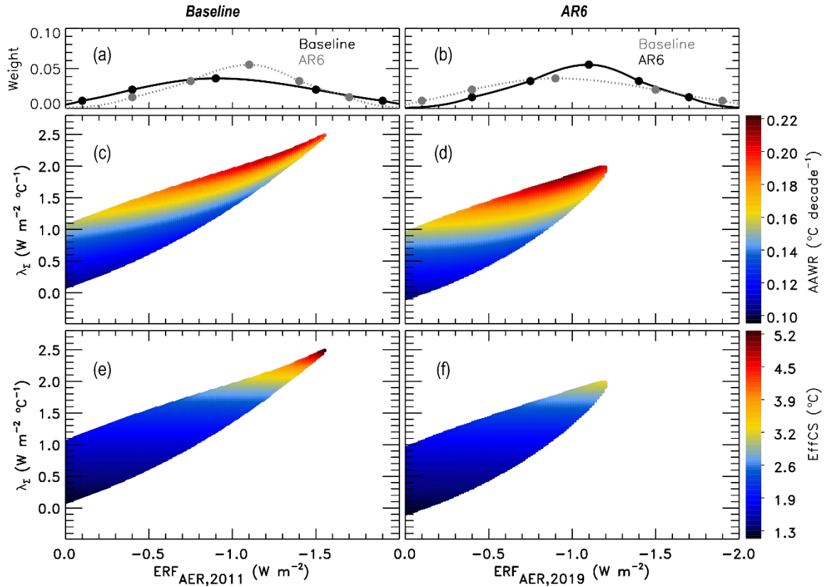
325 Figure 1: Aerosol weighting method and EM-GC computed values of AAWR and EffCS for combinations of ERF_{AER} and \lambda_{\Sigma} . (Left): Simulations using the Baseline framework. (Right): Simulations using the AR6 framework. (a–b) Asymmetrical Gaussians used to weight aerosol scenarios for probabilistic forecasts, as described in Sect. 2.2.2. Points marked on the Gaussians represent specific ERF values used as the central values, as well as 1\sigma and 2\sigma boundaries of each Gaussian (Table S3). The Gaussians are overlaid for 330 visual comparison. The Gaussians shown with the solid black line are used to weight the EM-GC output in each column. (c–d) EM-GC computed values of AAWR for the \lambda_{\Sigma} - ERF_{AER} ensemble. Colors denote the specific values of AAWR as indicated by the color bar on the right, and are only shown for the combinations of ERF_{AER} and \lambda_{\Sigma} for which a good fit to the HadCRUT5 historical climate record was found. (e–f) EM-GC computed values of EffCS for the \lambda_{\Sigma} - ERF_{AER} ensemble.
