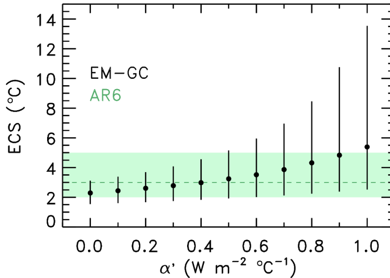
360 Figure 2: Equilibrium Climate Sensitivity (ECS) as the function of the pattern effect ( \alpha' , see text). Black vertical bars and circles correspond to the EM-GC 5–95% range, and 50% probability, respectively. The green shaded area and horizontal dashed line represent the AR6 very likely range, and central estimate of ECS respectively, from Table 7.13 of Forster et al. (2021). All results shown in this figure are based on simulations that use inputs from the AR6 framework.
