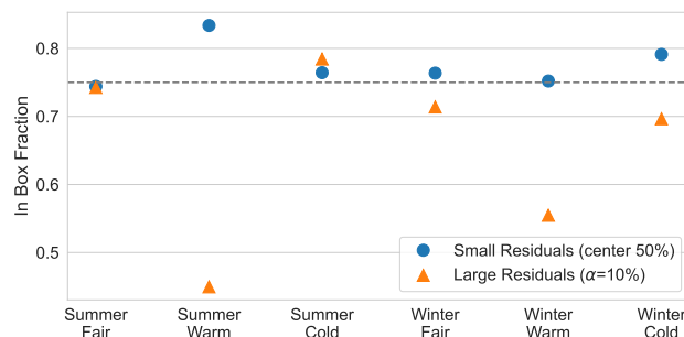
Figure 6. Fraction of ABL data found within the PRIM (75% coverage, dashed line) box for small (25–75 th percentiles) and large magnitude (< 5 th and > 95 th ) [\text{CO}_2] residuals separated by season and airmass. Data below the dashed line indicate that residuals are less likely associated with typical environmental conditions for that expert-designated case.
