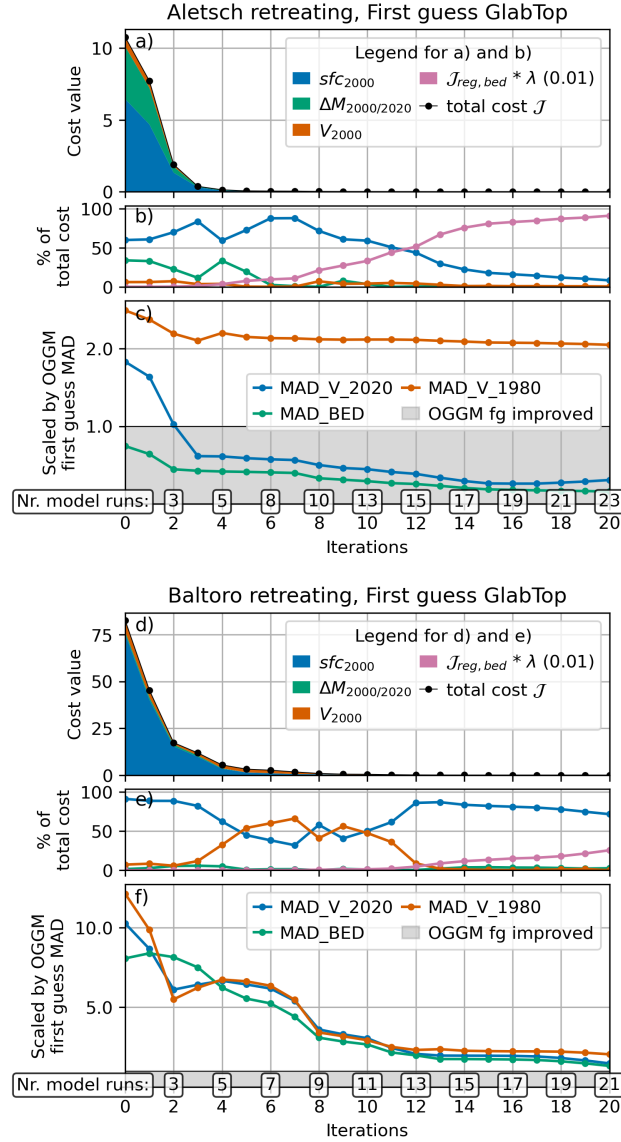
Figure 7. Same as Figure 4, for Aletsch (a, b and c) and Baltoro (d, e and f) retreating using GlabTop first guess.
