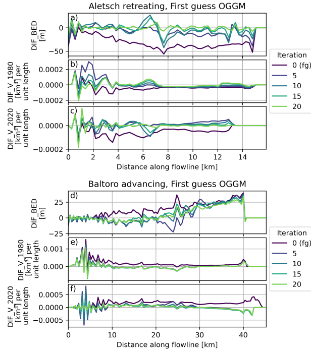
Figure 6. Differences between the synthetic truth and AGILE guess after 10 and 20 iterations along the flowline for Aletsch retreating (a to c) and Baltoro advancing (d to f), starting from the OGGM first guess (0 Iteration) with a \lambda value of 0.01. Panels a and d show the differences in bed height, panels b and e shows the differences in volume for 1980, and panels c and f show the differences in volume for 2020. All differences are displayed for every grid point along the flowline.
