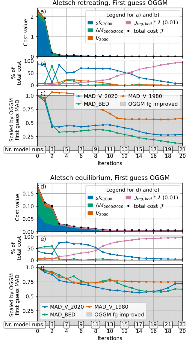
Figure 4. Evolution of the cost function and performance metrics for Aletsch retreating (a to c) and equilibrium (d to f), starting from the OGGM first guess, with a \lambda value of 0.01. Panels a and d show the evolution of the cost function over minimization iterations, with individual cost terms represented in different colors. The relative contribution of the cost terms to the total cost is shown in panels b and e. Panels c and f illustrate the evolution of performance metrics over the same iterations. The numbers in boxes along the x-axis indicate the total number of forward model runs required for each corresponding iteration.
