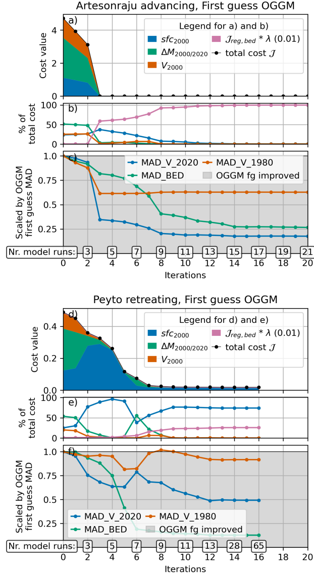
Figure 5. Same as Figure 4, for Artesonraju advancing (a, b and c) and Peyto retreating (d, e and f) starting from the OGGM first guess.
