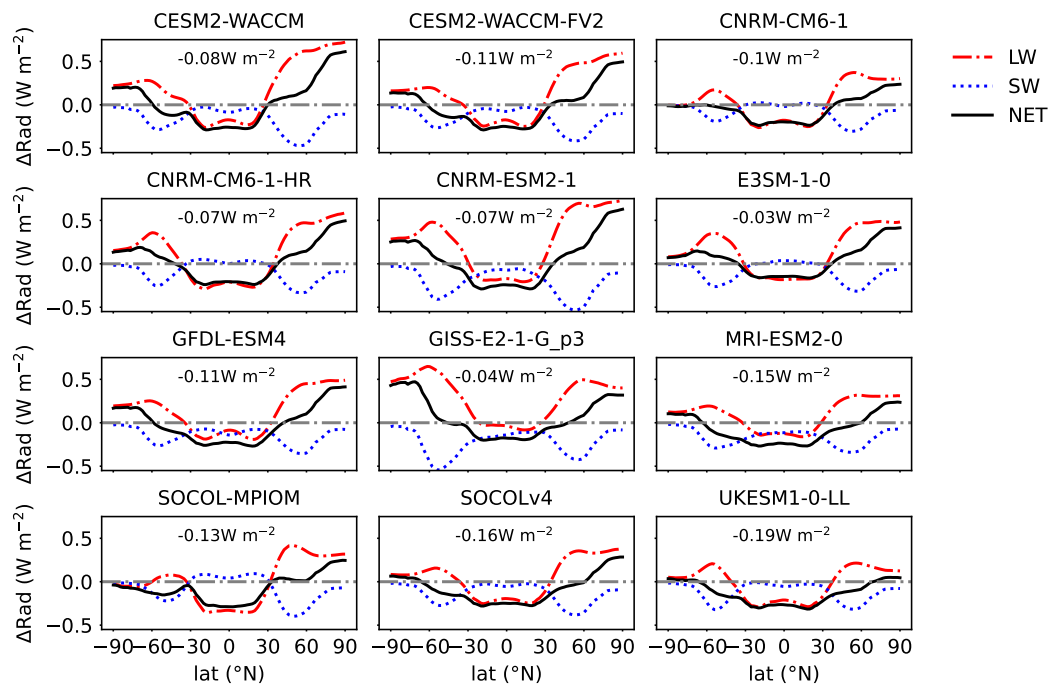
Figure 8. Annual-mean zonal-mean response of radiative fluxes at the tropopause to ozone from chem models for the 4×CO 2 experiment. The longwave, shortwave and net radiative flux response are denoted with red (dash-dotted), blue (dotted) and black lines, respectively. The value of the global mean net flux change is shown as number in each subplot.
