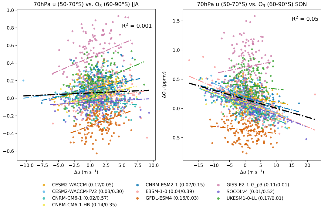
Figure B2. 150-year-long seasonal-mean ozone response in 60-90°S to zonal wind ( u ) change in 50-70°S at 70hPa in JJA and SON for 1pctCO 2 . Fitting lines retrieved from linear regression are plotted as dash-dotted lines with the corresponding color for each model. The thick black line is fitted using data from all models with the corresponding R^2 denoted in the upper right corner of the plot. R^2 values for each model are denoted in the legend for JJA and SON respectively.
