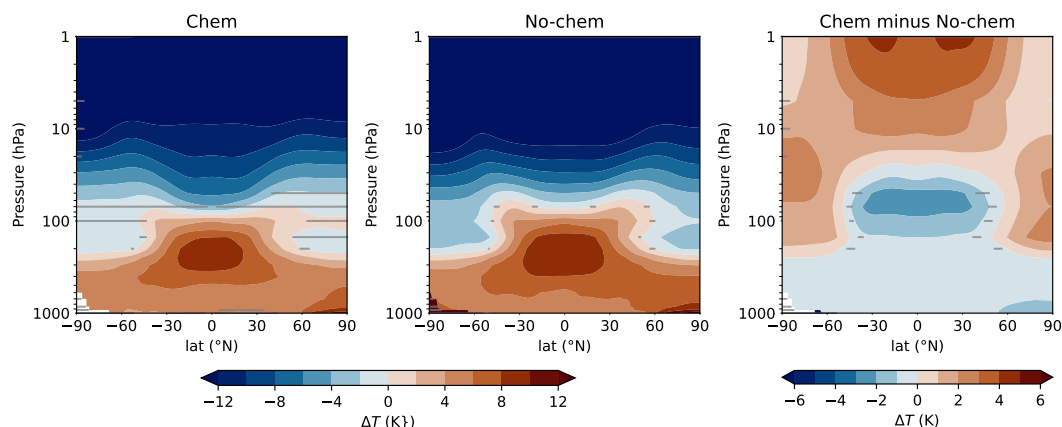
Figure 10. Similar to Figure 9, but average of 100-year long annual mean air temperature response to 4\times\text{CO}_2 of six -seven pairs of chem and no-chem models.
