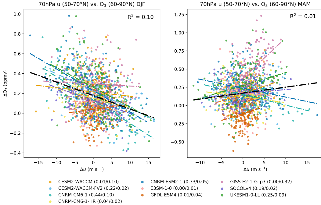
Figure 3. 150-year-long seasonal-mean ozone response in 60-90°N to zonal wind ( u ) change in 50-70°N at 70hPa in MAM and DJF and MAM for 1pctCO 2 . Fitting lines retrieved from linear regression are plotted as dash-dotted lines with the corresponding color for each model. The thick black line is fitted using data from all models with the corresponding R 2 denoted in the upper right corner of the plot. R 2 values for each model are denoted in the legend for DJF and MAM respectively.
