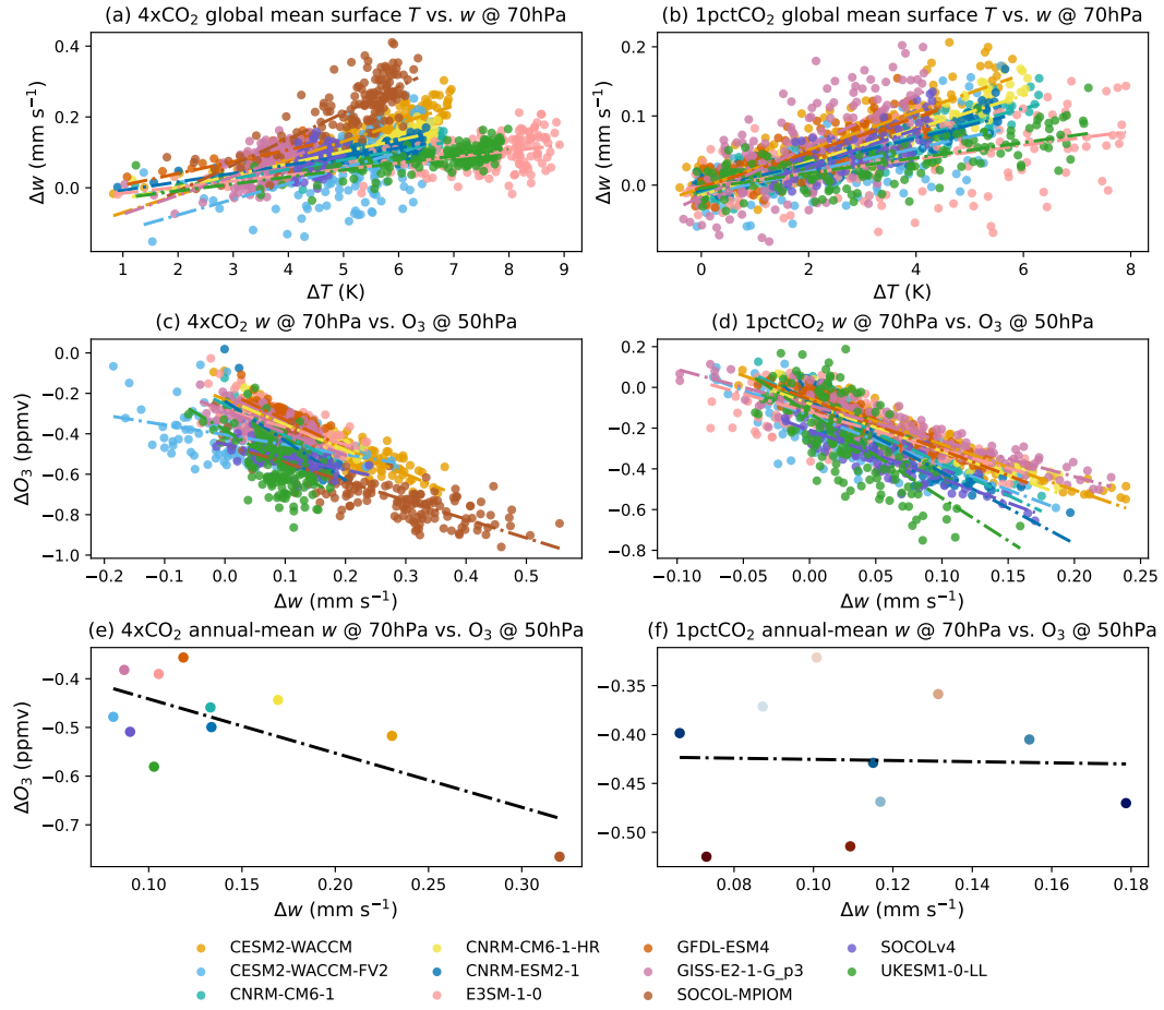
Figure 4. (a)-(b): Annual-mean tropical ( 20^{\circ}\text{S} - 20^{\circ}\text{N} ) upwelling (w) response to global mean surface temperature for the 4\times\text{CO}_2 and 1pctCO 2 experiments for individual year. (c)-(d): Same as (a)-(b), but contrasting upwelling changes with the ozone response. (e)-(f): Same as (c)-(d), but averaged over the last 100 years for 4\times\text{CO}_2 and for all the 150 years for 1pctCO 2 experiment. Fitting lines retrieved from a linear regression are plotted with the corresponding color of each model.
