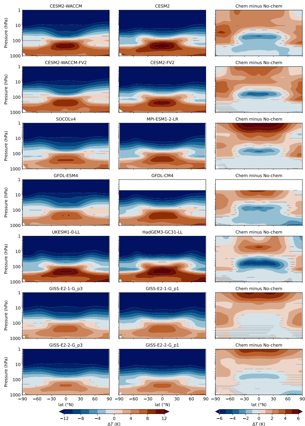
Figure 9. Comparison of the 100-year long annual-mean air temperature response to 4\times\text{CO}_2 between six seven pairs of chem and no-chem CMIP6 models. The left column shows the response from chem models, the middle column shows the response from no-chem models and the right column shows the difference between chem and no-chem models.
