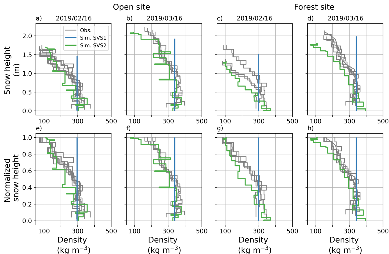
Figure 4. Simulated (with SVS1 in blue and SVS2 in green) and observed vertical snow density profiles in (a, b, e, f) the open site and (c, d, g, h) the forest site at two different dates during the 2018/19 winter season at Snow Crested Butte. The first row shows raw vertical profiles whereas the second row shows normalized profiles where the thickness of the layers in each observed and simulated profile is normalized by total snow height.
