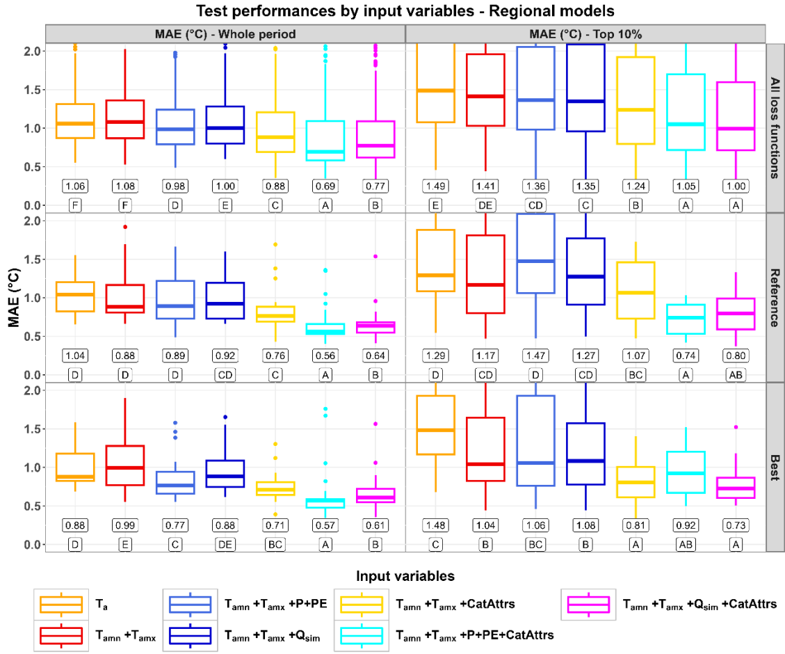
375 Figure 4: Distributions of the test performances (MAE, in °C) of the regionally trained models over the whole test period (left column) and the test subperiod corresponding to the highest 10% observed values (right column). Top row shows the distribution over all the loss functions ( 18 \times 21 = 378 points per distribution). The middle row shows the performances for the reference loss function (MSE with standardization, 21 points per distribution). The bottom row shows the performances with the best loss function over all sets of input variables (MAE with standardization for the whole period and MSE without standardization for the top 10%, 21 points per distribution). Numerical values under the boxes represent the median value for each distribution. Letters under the numerical values rank the distributions, and are defined such as distributions that share at least one letter are not significantly different according to the binomial test. 380
