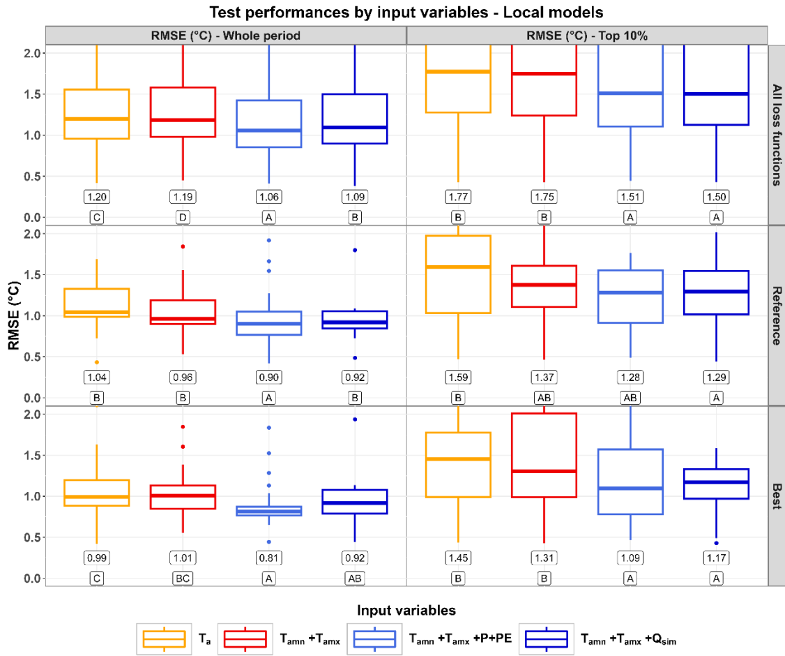
535 Figure C2: Distributions of the test performances (RMSE, in °C) of the local models over the whole test period (left column) and the 540 test subperiod corresponding to the highest 10% observed values (right column). This figure is similar to Fig. 3 but with RMSE as a criterion to evaluate the test performances. The top row shows the distribution over all the loss functions ( 18 \times 21 = 378 points per distribution). The middle row shows the performances for the reference loss function (MSE with standardization, 21 points per distribution). The bottom row shows the performances for the best loss function over all sets of input variables (MAE without standardization for the whole period and M4E with standardization for the top 10%, 21 points per distribution). Numerical values under the boxes represent the median value for each distribution. Letters under the numerical values rank the distributions, and are defined such as distributions that share at least one letter are not significantly different according to the binomial test.
