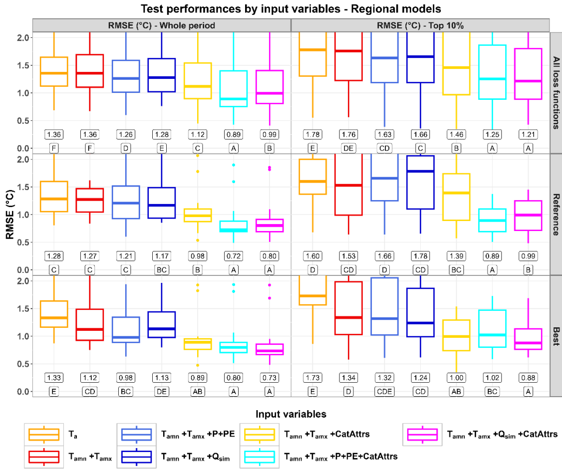
545 Figure C3: Distributions of the test performances (RMSE, in °C) of the regionally trained models over the whole test period (left column) and the test subperiod corresponding to the highest 10% observed values (right column). This figure is similar to Fig. 4 but with RMSE as a criterion to evaluate the test performances. Top row shows the distribution over all the loss functions ( 18 \times 21 = 378 points per distribution). The middle row shows the performances for the reference loss function (MSE with standardization, 21 points per distribution). The bottom row shows the performances with the best loss function over all sets of input variables (MSE without standardization for both cases). Numerical values under the boxes represent the median value for each distribution. Letters under the numerical values rank the distributions, and are defined such as distributions that share at least one letter are not 550 significantly different according to the binomial test.
