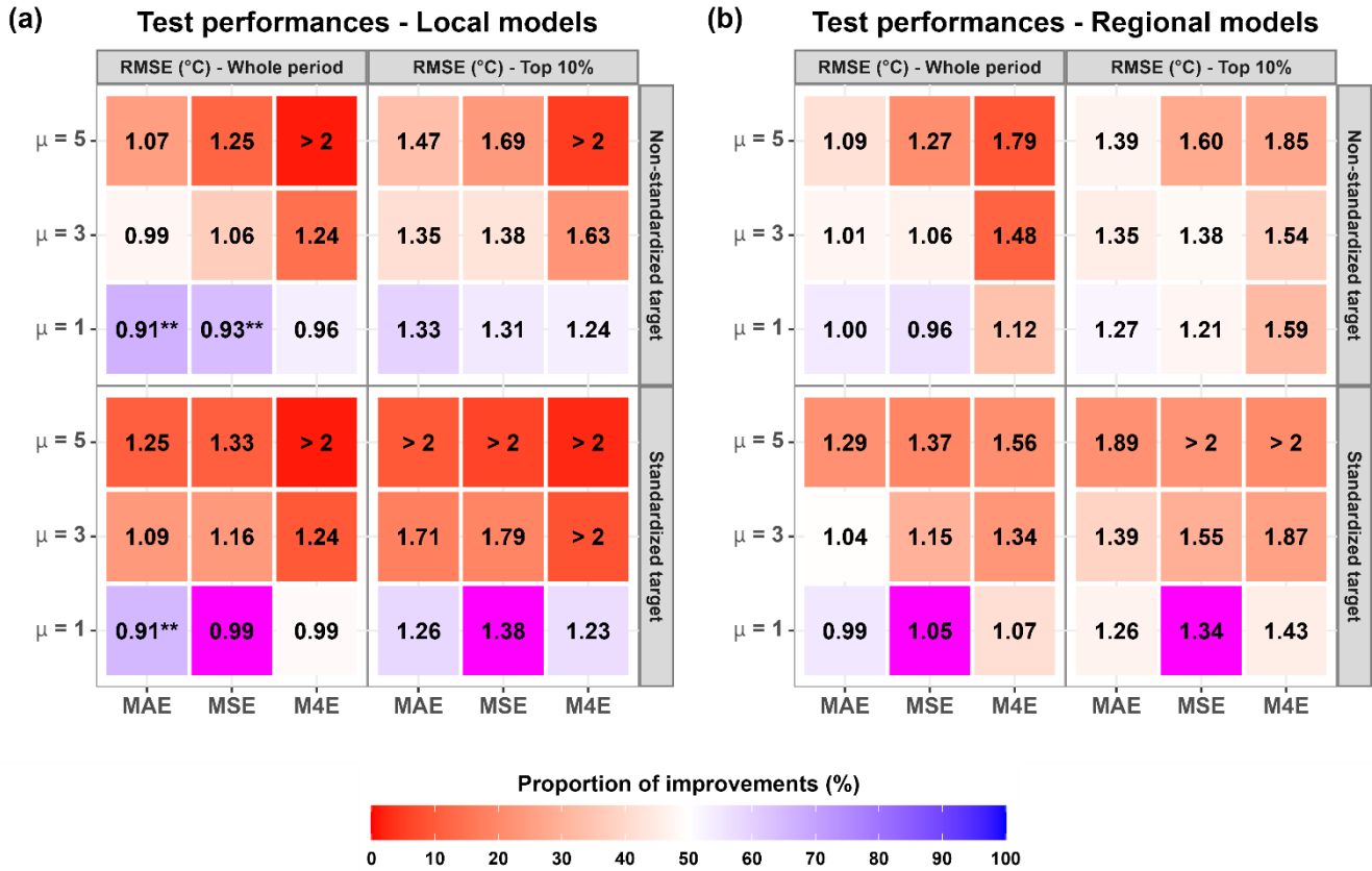
530 Figure C1: Median test performances (RMSE, in °C) of the local models (a) and the regional models (b) according to the loss function used for training. This figure is similar to Fig. 2 but with RMSE as a criterion to evaluate test performances. Colours indicate the proportion of cases for which the use of the loss function yielded better results than the reference loss function (MSE with standardization, shown in magenta). Asterisks indicate that the custom loss function is significantly better than the reference loss function according to the binomial test: * for a significance threshold of 5%, ** for a threshold of 1%, and *** for a threshold of 0.1%.
