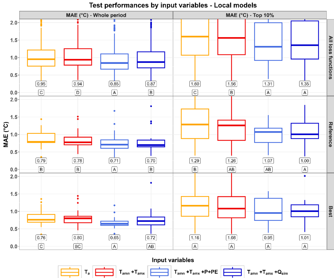
350 Figure 3: Distributions of the test performances (MAE, in °C) of the local models over the whole test period (left column) and the test subperiod corresponding to the highest 10% observed values (right column). The top row shows the distribution over all the loss functions ( 18 \times 21 = 378 points per distribution). The middle row shows the performances for the reference loss function (MSE with standardization, 21 points per distribution). The bottom row shows the performances for the best loss function over all sets of input
