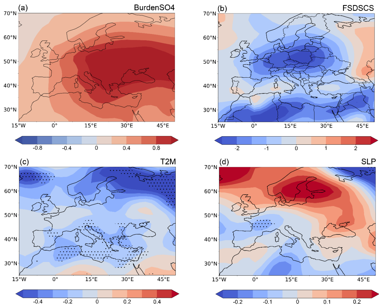
651 Figure 3. Spatial patterns of the 1901-1955 linear trends of the JJA average (a) column sulphate aerosol burden 652 ( 10^{-5} \text{ kg m}^{-2} (55 \text{ years})^{-1} ), (b) surface clear-sky downward shortwave radiation ( \text{W m}^{-2} (55 \text{ years})^{-1} ), (c) 2-m air 653 temperature ( \text{K} (55 \text{ years})^{-1} ), and (d) sea level pressure ( \text{hPa} (55 \text{ years})^{-1} ) associated with increased European 654 sulphate aerosols (difference between the ALL and fixEU ensemble means). The black dots in (c) and (d) mark 655 the grid points for which the trend exceeds the 90% significance level according to the two-tailed Student's t-test.
