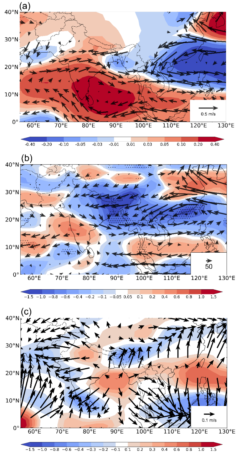
Figure 2. Spatial patterns of the 1901-1955 linear trends of the JJA average (a) 850-hPa winds ( \text{m s}^{-1} (55 \text{ years})^{-1} ) and 925-hPa streamfunction (colors, 10^6 \text{ m}^2 \text{ s}^{-1} (55 \text{ years})^{-1} ), (b) 1000-300 hPa vertically integrated moisture transport (vectors, \text{Kg m}^{-1} \text{ s}^{-1} ) and its divergence (shades, \text{mm d}^{-1} (55 \text{ years})^{-1} ), (c) 150-hPa divergent circulation ( \text{m s}^{-1} (55 \text{ years})^{-1} ) and its divergence (shades; 10^{-6} \text{ s}^{-1} (55 \text{ years})^{-1} ) associated with increased European sulphate aerosols (difference between the ALL and fixEU ensemble means). The black dots in (b) mark the grid points for which the trend exceeds the 90% significance level according to the two-tailed Student's t-test.
