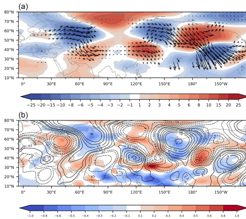
Figure 4. Spatial patterns of the 1901-1955 linear trends of the JJA average (a) 300-hPa wave activity flux (vectors; 10^{-4} \text{ m}^2 \text{ s}^{-2} (55 \text{ years})^{-1} ) and streamfunction (shades; 10^5 \text{ m}^2 \text{ s}^{-1} (55 \text{ years})^{-1} ), and (b) 300-hPa meridional wind (contours; \text{m s}^{-1} (55 \text{ years})^{-1} ) and 500-hPa vertical velocity (shades; 10^{-2} \text{ Pa s}^{-1} (55 \text{ years})^{-1} ) associated with increased European sulphate aerosols (difference between the ALL and fixEU ensemble means).
