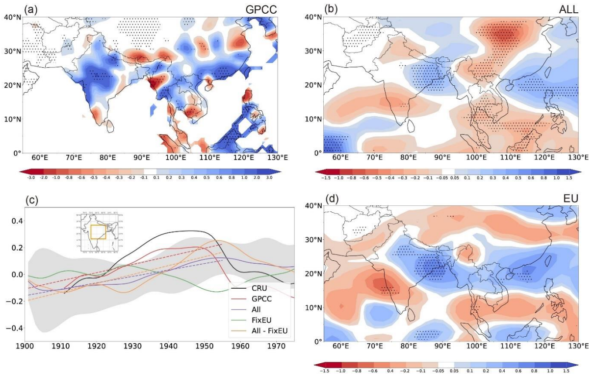
Figure 1. (a)-(b): Spatial patterns of the 1901-1955 linear trends of JJA precipitation ( \text{mm day}^{-1} (55 \text{ years})^{-1} ) for (a) GPCC, (b) the all-forcing ensemble (ALL), and (d) the difference between ALL and the all-forcing experiment with fixed preindustrial aerosol emissions over Europe (fixEU), representing the impact of EU aerosols. The black dots mark the grid points for which the trend exceeds the 90% significance level according to the two-tailed Student's t-test. (c): Time series of area-averaged JJA precipitation anomalies ( \text{mm day}^{-1} ; deviations from the 1901-2000 climatology) over central-northern India (land-only points within 75^{\circ} – 87^{\circ}\text{E} , 16^{\circ} – 27^{\circ}\text{N} ; area shown in inset map) smoothed with 11-year running means to highlight low-frequency (multi-decadal) fluctuations. The black and red lines represent observations (CRU and GPCC, respectively), while the purple, green and orange lines represent the ensemble means of ALL, fixEU, and their difference (EU). The grey shading represents the standard deviation of the eight-member ALL ensemble around the mean. The 1901-1955 least-squares linear trends of the simulated time series are shown as dashed lines in the corresponding colours. Note that the interval for the simulated changes is half of that used for the observations.
