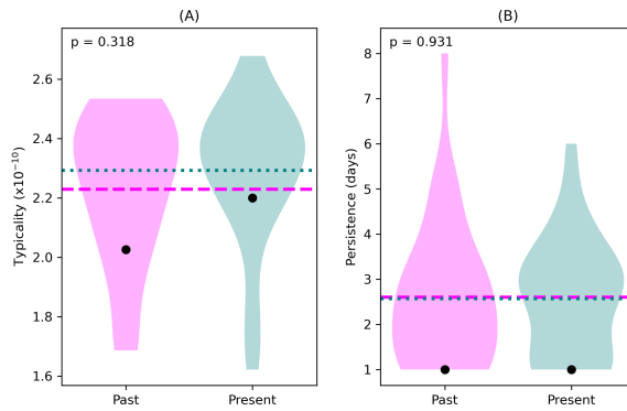
Figure 3: The changes in typicality (A) and persistence (B) for spring between the past (1950–1979) and present (1994–2023) periods. Black dots indicate the typicality and persistence of the event. The violins show the distribution of the t_{analogue} and p_{analogue} values, whose means are represented by dashed lines for the past period and dotted lines for the present period. The p-value indicates the statistical significance of the difference between these means.
