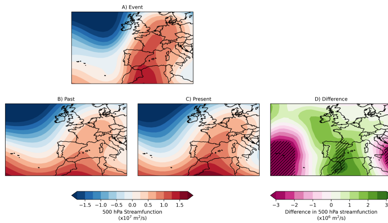
Figure 5: The difference in 500 hPa streamfunction between analogue composites from the present (1994–2023) and past (1950–1979) periods. Hatched areas show regions where the difference is significant on a 95% confidence level.
