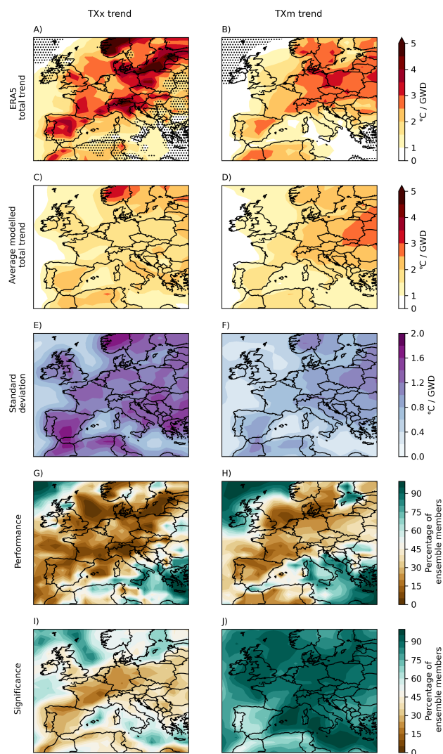
295 Figure 7: The ERA5 total temperature trends in the maximum (TXx) and the mean (TXm) of the daily maximum spring temperatures up to 2014, the mean trends found by the 105 model ensemble members from the HadGEM3 and MIROC6 models, the standard deviation of the modelled trends, the percentage of the ensemble members that find a trend as high as the ERA5 trend or higher, and the percentage of the ensemble members that find a trend that is statistically significant on a 95% confidence level.
