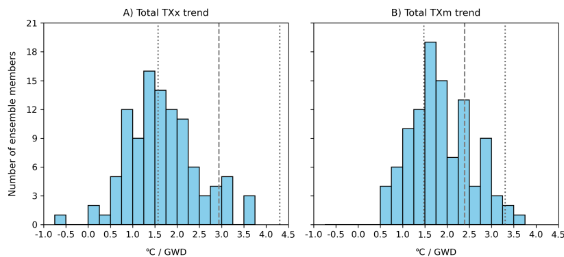
Figure 8: The distribution of the trends in the maximum (TXx) and the mean (TXm) of the daily maximum spring temperatures, averaged for Western Europe, as found by 105 ensemble members from the HadGEM3 and MIROC6 models. The dashed grey lines represent the trends found in ERA5, with dotted lines showing their 95% confidence interval.
