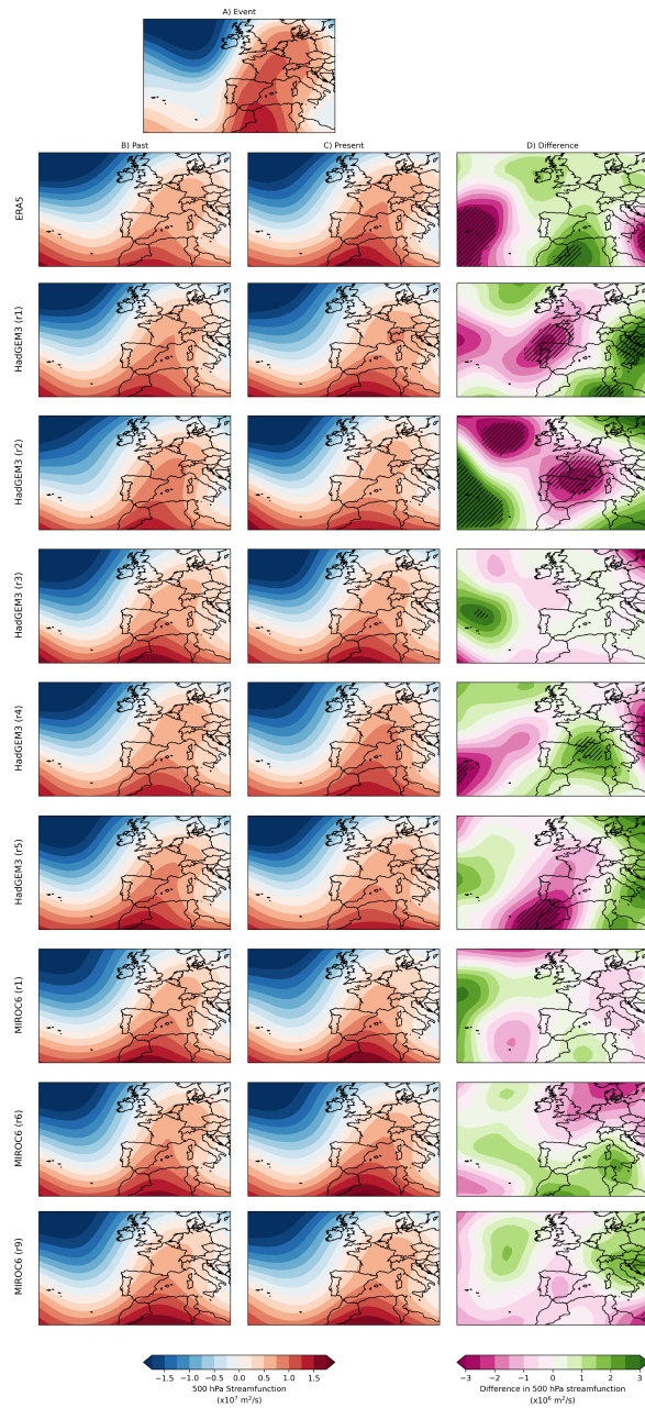
Figure 9: The difference in 500 hPa streamfunction between analogue composites from the past (1950–1979) and present (1985–2014) periods, for ERA5 and the different model ensembles. Hatched areas show regions where the difference is significant on a 95% confidence level.
