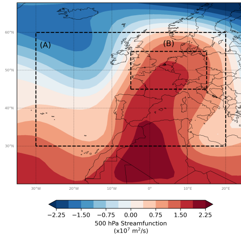
Figure 1: The 500 hPa streamfunction for the Southerly Flow event on 29 June 2019. Box (A) shows the domain used to select analogues. Box (B) shows the area over which trends for Western Europe are averaged.
