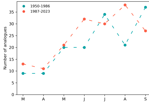
270 Figure 6: The distribution of analogues within the fifth percentile of Euclidean distances over different months, for two time periods.
