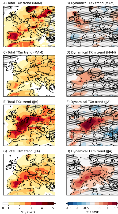
Figure 2: The total trends in the maximum (TXx) and the mean (TXm) of the daily maximum temperatures in a season, for spring and summer, and the dynamical contributions to these trends. Trends are calculated using the ERA5 dataset and are expressed in the amount of warming, in degrees Celsius, per global warming degree (GWD). Dotted areas represent regions where the trend is not significant on a 95% confidence level.
