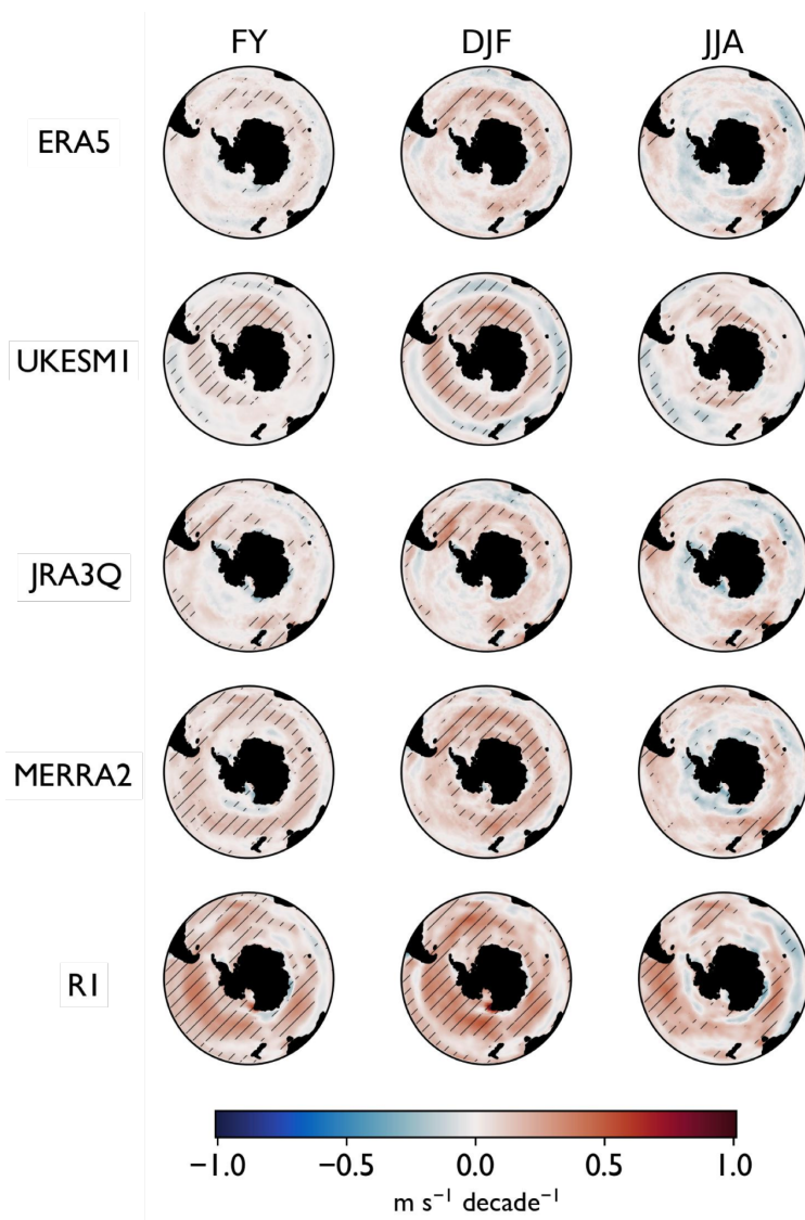
Fig. 3: Decadal trends in 10-m wind speed (1980-2019). Hatching shows trends significant at the 95% confidence level. See also Table 5.
