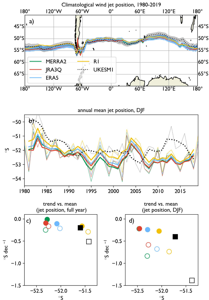
3 Fig. 4: Summary statistics for the wind jet. The wind jet is calculated as the location of the maximum of 4 the u -component of the 10-m wind speed between 30°S and 70°S (see Methods). a): the climatological 5 mean annual jet position, with one standard deviation of the annual mean shown for ERA5 and UKESMI. 6 b): The zonal mean of the austral summer jet position. Thick lines indicate smoothing by a 3-point 7 running mean filter. c-d): Trends in the annual (c) and summer (d) jet position mean vs. climatological 8 means. Colours from panel a) are repeated throughout the figure. See also Sup. Tables ST3 and ST4.
