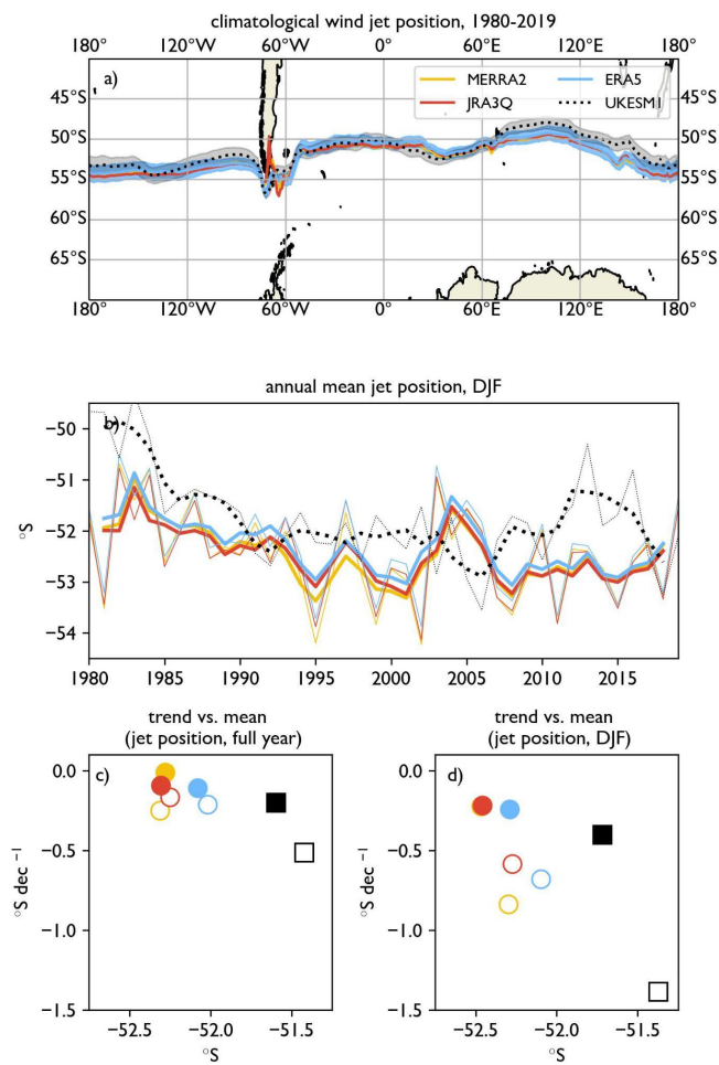
2 3 Fig. 4: Summary statistics for the wind jet. The wind jet is calculated as the location of the maximum of 4 the u -component of the 10-m wind speed between 30°S and 70°S (see Methods). a): the climatological 5 mean annual jet position, with one standard deviation of the annual mean shown for ERA5 and UKESM1. 6 b): The zonal mean of the austral summer jet position. Thick lines indicate smoothing by a 3-point 7 running mean filter. c-d): Trends in the annual (c) and summer (d) jet position mean vs. climatological 8 means. Colours from panel a) are repeated throughout the figure. See also Sup. Tables ST3 and ST4.
