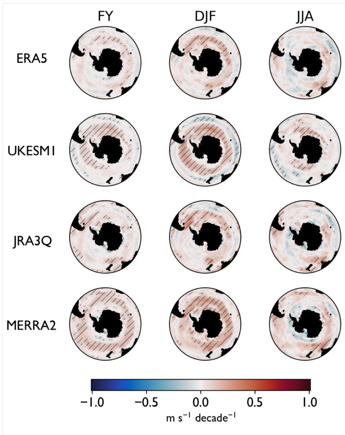
2 3 Fig. 3: Decadal trends in 10-m wind speed (1980-2019). Hatching shows trends significant at the 95% 4 confidence level. See also Table 5. 5 6
