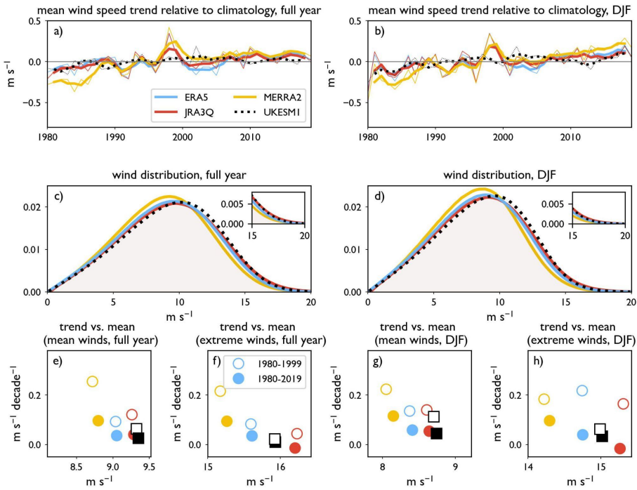
2 3 4 Fig. 2: Summary statistics for wind distributions in four reanalysis products and UKESM1. a-b): mean 5 10-m wind speed trends relative to climatology for a) full year and b) DJF only. Thick lines have been 6 smoothed by a three-point running filter. c-d): windspeed frequency distribution (100 bins, 0-20 m s^{-1} ) 7 for c) full year and d) DJF, with high tails shown in inset. e-h) Trends in mean and extreme winds for full 8 year and DJF vs. climatological means, with colours the same as in panel a). Filled symbols represent 9 1980-2019, while open symbols represent 1980-1999; circles represent reanalyses while squares 10 represent UKESM1. Colours from panel a) are repeated throughout the figure. Summary statistics shown 11 in panels e)-h) are also given in Tables 4 and 5. All figure statistics are calculated for daily winds at 12 1^{\circ} \times 1^{\circ} resolution, 40^{\circ}S - 60^{\circ}S .
