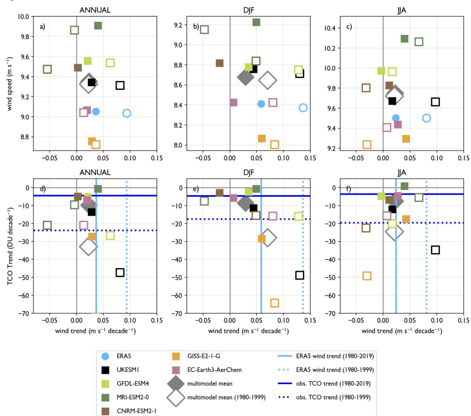
2 3 Fig. 6: 10-m wind speed, decadal wind speed trend, and decadal TCO trend (70°S- 90°S) for CMIP 4 models with interactive chemistry. For each model, one ensemble member is used (see Table 2). Wind 5 speeds and trends are calculated from daily winds at 1°x1° resolution, 40°S- 60°S. Note the caveats 6 regarding TCO trends in GISS-E2-I-G discussed in section 3.4. 7 8
