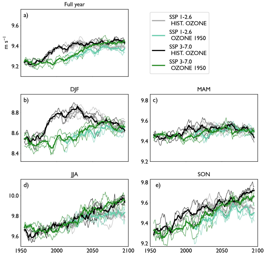
Fig. 7: 10-m wind speed evolution from 1950 to 2100 in the OZONE-1950 and OZONE-HIST experiments. a) Full year, b-e): seasonally subdivided means. All means are calculated for daily winds at 1^\circ \times 1^\circ resolution, 40^\circ\text{S} - 60^\circ\text{S} . For each experiment, three ensemble members are shown, with the ensemble mean shown in bold. All lines are smoothed with a 10-year running filter. See also Table 6.
