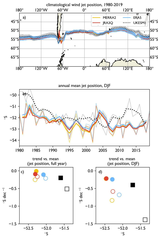
3 Fig. 4: Summary statistics for the wind jet. The wind jet is calculated as the location of the maximum of 4 the u -component of the 10-m wind speed between 30°S and 70°S (see Methods). a): the climatological 5 mean annual jet position, with one standard deviation of the annual mean shown for ERA5 and UKESM1. 6 b): The zonal mean of the austral summer jet position. Thick lines indicate smoothing by a 3-point 7 running mean filter. c-d): Trends in the annual (c) and summer (d) jet position mean vs. climatological 8 means. Colours from panel a) are repeated throughout the figure. See also Sup. Tables ST3 and ST4.
