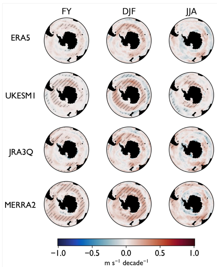
2 3 Fig. 3: Decadal trends in 10-m wind speed (1980-2019). Hatching shows trends significant at the 95% 4 confidence level. See also Table 5. 5 6
