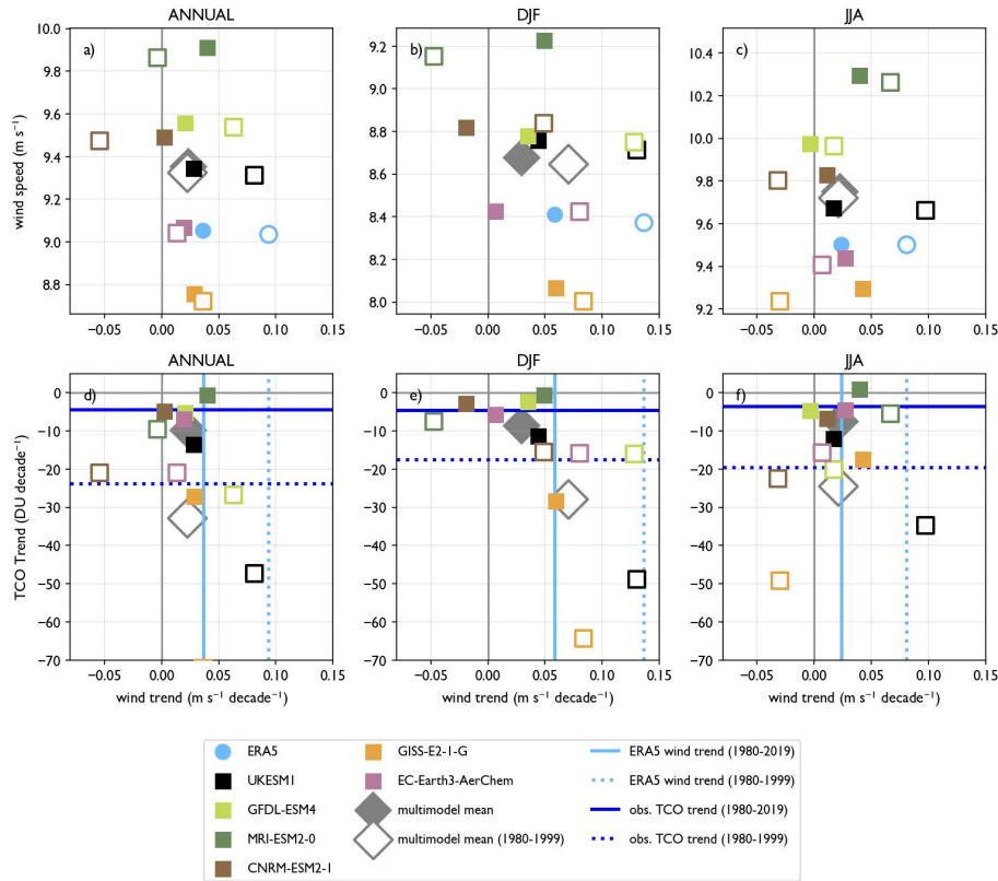
3 Fig. 6: 10-m wind speed, decadal wind speed trend, and decadal TCO trend (70°S- 90°S) for CMIP 4 models with interactive chemistry. For each model, one ensemble member is used (see Table 2). Wind 5 speeds and trends are calculated from daily winds at 1°x1° resolution, 40°S- 60°S. Note the caveats 6 regarding TCO trends in GISS-E2-I-G discussed in section 3.4.
