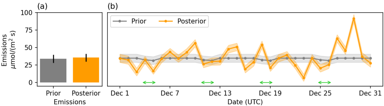
420 Figure 5: (a) Comparison of time- and domain-averaged emissions between prior and posterior estimates for December 2021 in Seoul, and (b) time series of domain-averaged daily (daytime average) prior and posterior CO 2 emissions, including emission uncertainties. Green arrows indicate weekends.
