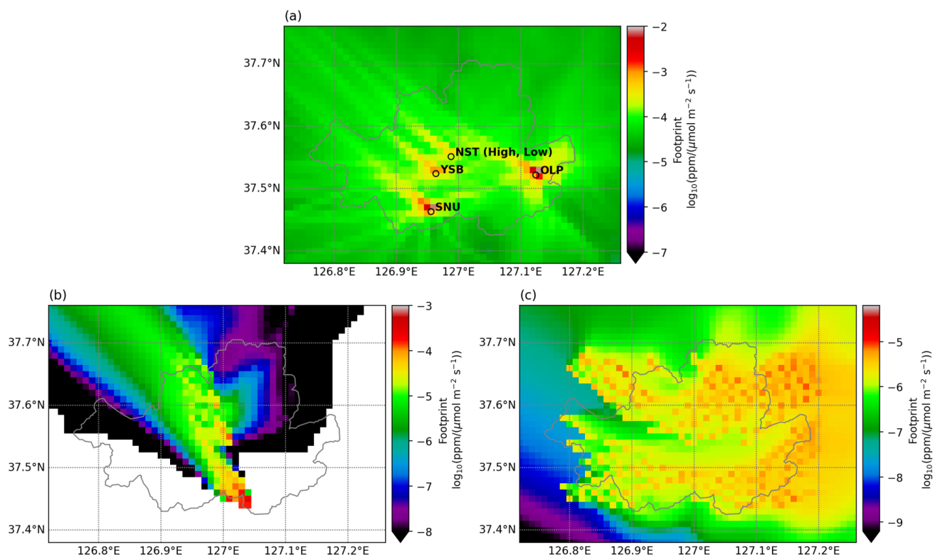
Figure 3: Footprint averages on a \log_{10} scale to upwind source regions of (a) daytime-only ground observations (10:00–16:00 KST) during December 2021, (b) OCO-2 satellite data on December 4, 2021, at 13:00 KST, and (c) OCO-3 satellite data on December 5, 2021, at 11:00 KST across the Seoul domain. Note that the footprint ranges differ in panels (a), (b), and (c) for visualization purposes.
