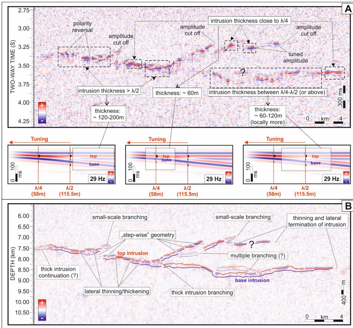
Figure 17: Seismic interpretation of igneous intrusion imaged by profile PL-1200 (cf. Fig. 8). (A) PreSTM seismic profile with detailed interpretation of reflection amplitude and an estimation of intrusion thickness based on seismic tuning and vertical resolution criteria obtained from the wedge model analysis (Fig. 13). Three wedge models, calculated using zero-phase Ricker wavelet with 29 Hz dominant frequency, demonstrate various seismic responses depending on different sill thicknesses; (B) Part of PreSDM PL-1200 profile that illustrates interpreted top and base of the intrusion and its inferred geometry.
