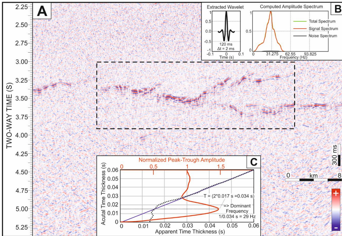
380 Figure 8: Seismic tuning analysis for polygon 3. (A) Enlarged part of PL-1200 seismic profile that illustrates detailed seismic expression of inferred igneous intrusion within the crystalline basement of the Baltic Basin (cf. Fig. 4). Black dotted rectangle indicates seismic wavelet extraction window for tuning analysis. (B) Extracted wavelet parameters with the computed amplitude spectrum. (C) Results of the seismic tuning analysis (tuning thickness chart) for the statistical wavelet extracted within a defined window, see text for additional explanation.
