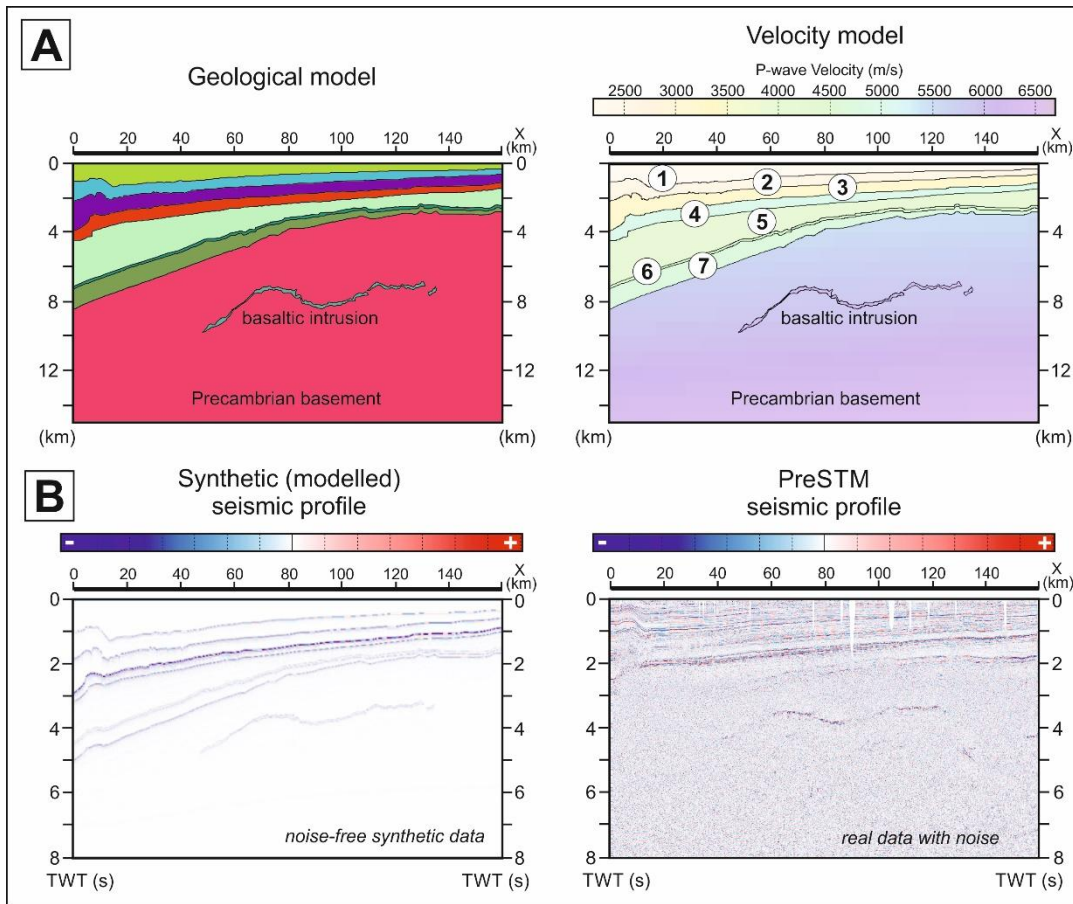
465 Figure 11: 2D seismic modeling for profile PL-5400 - basalt scenario. (A) Left - geological model based on interpreted PL-5400 profile; right - P-wave velocity model: (1) Cretaceous and Cenozoic: velocity 2200 m/s, density 2.1 g/cm 3 , (2) Jurassic: velocity 2500 m/s, density 2.2 g/cm 3 , (3) Triassic: velocity 3200 m/s, density 2.23 g/cm 3 , (4) Permian (Zechstein evaporites): velocity 5000 m/s, density 2.5 g/cm 3 , (5) Silurian: velocity 4000 m/s, density 2.35 g/cm 3 , (6) Ordovician: velocity 4300 m/s, density 2.4 g/cm 3 , (7) Cambrian: velocity 4750 m/s, density 2.5 g/cm 3 , Precambrian basement: vertical velocity gradient 5500–6500 m/s, density gradient 2.58–2.81 g/cm 3 , basaltic intrusion: velocity 6240 m/s and density 2.76 g/cm 3 (after Murase and McBirney, 1973; Brown and Kim, 470 2020); (B) Comparison of synthetic profile and real PreSTM seismic profile.
