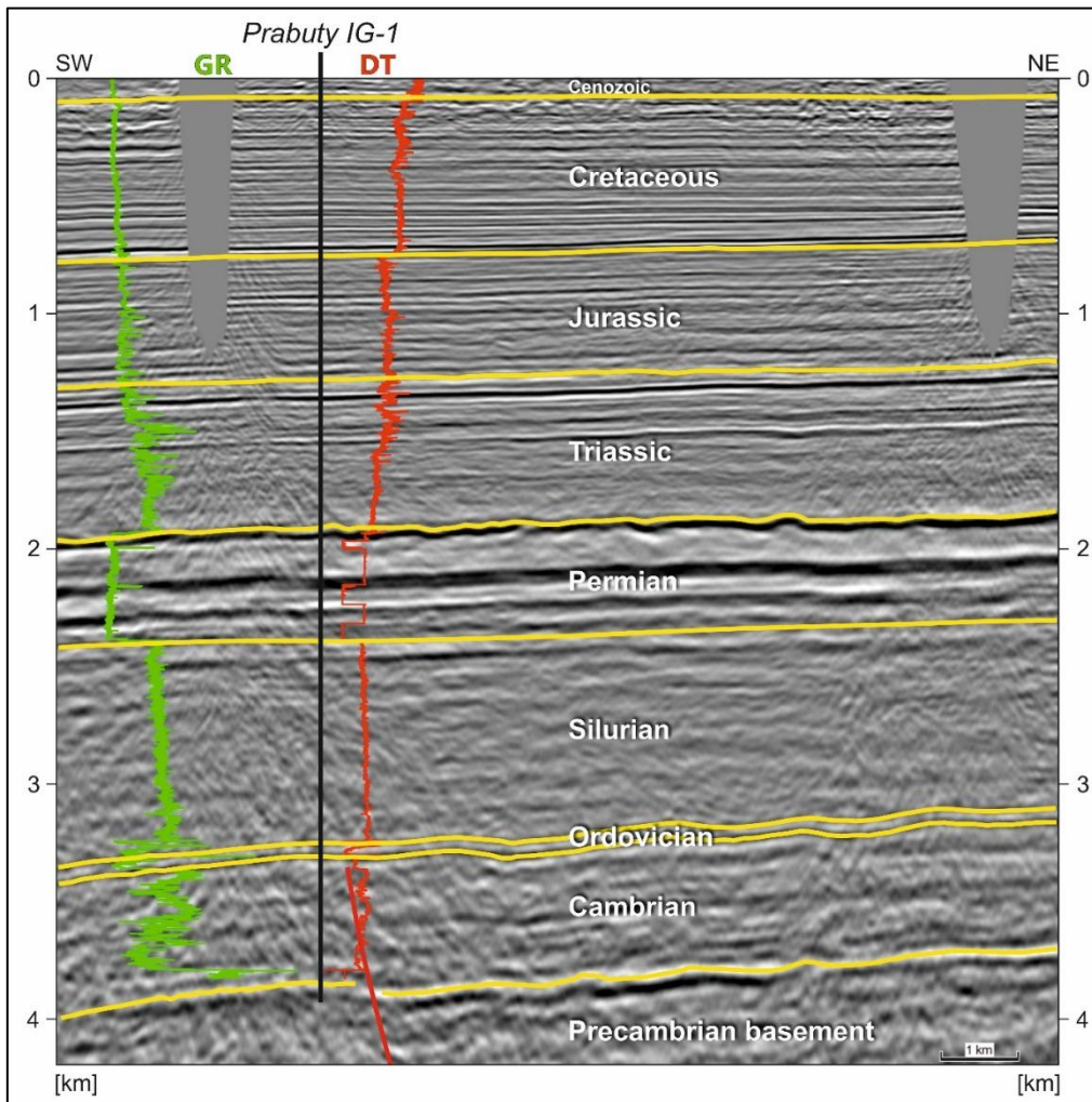
425 Figure 9: Correlation of deep calibration well Prabuty IG-1 with PSDM version of PL-5400 profile. GR: natural gamma ray log, DT: sonic log.
