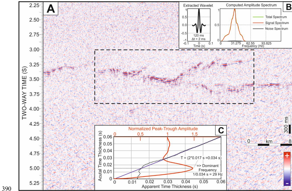
Figure 8: Seismic tuning analysis for polygon 3. (A) Enlarged part of PL-1200 seismic profile that illustrates detailed seismic expression of inferred igneous intrusion within the crystalline basement of the Baltic Basin (cf. Fig. 4). Black dotted rectangle indicates seismic wavelet extraction window for tuning analysis. (B) Extracted wavelet parameters with the computed amplitude spectrum. (C) Results of the seismic tuning analysis (tuning thickness chart) for the statistical wavelet extracted within a defined window, see text for additional explanation.
