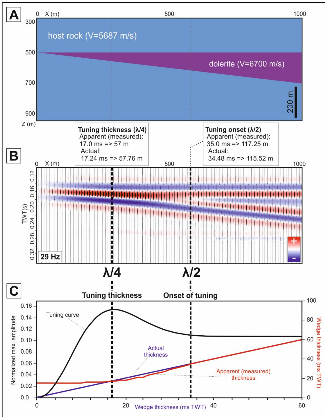
510 Figure 13: Wedge model used to evaluate role of tuning and vertical resolution of seismic imaging of dolerite intrusion. (A) wedge thickness ranges from 0 to 200 m, and the total length of the model is 1000 m, velocity and density values of the host rock have been 5687 m/s and 2.73 g/cm 3 , respectively, and for dolerite wedge 6700 m/s and 2.87 g/cm 3 , respectively (cf. Fig. 12). (B) Theoretical seismic profile obtained by using a zero-phase Ricker wavelet of 29 Hz (cf. Fig. 6, Fig. 7 and Fig. 8). (C) Graph of the tuning curve versus apparent and actual wedge thickness. Predicted amplitude displays maximum response at an estimated thickness of 57-58 m.
