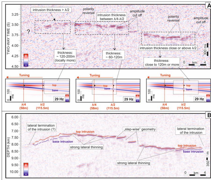
Figure 145: Seismic interpretation of igneous intrusion imaged by profile PL-5400, part 1 (cf. Fig. 6). (A) PreSTM seismic profile with detailed interpretation of reflection amplitude and an estimation of intrusion thickness based on seismic tuning and vertical resolution criteria obtained from the wedge model analysis (Fig. 13). Three wedge models, calculated using zero-phase Ricker wavelet with 29 Hz dominant frequency, demonstrate various seismic responses depending on different sill thicknesses; (B) Part of PreSDM PL-5400 profile that illustrates interpreted top and base of the intrusion and its inferred geometry.
