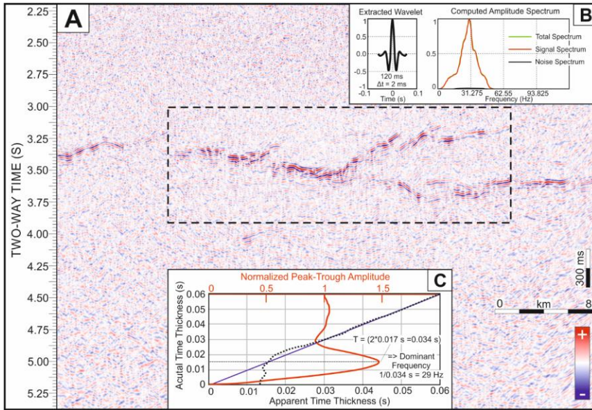
385 Figure 8: Seismic tuning analysis for polygon 3. (A) Enlarged part of PL-1200 seismic profile that illustrates detailed seismic expression of inferred igneous intrusion within the crystalline basement of the Baltic Basin (cf. Fig. 4). Black dotted rectangle indicates seismic wavelet extraction window for tuning analysis. (B) Extracted wavelet parameters with the computed amplitude spectrum. (C) Results of the seismic tuning analysis (tuning thickness chart) for the statistical wavelet extracted within a defined window, see text for additional explanation.
