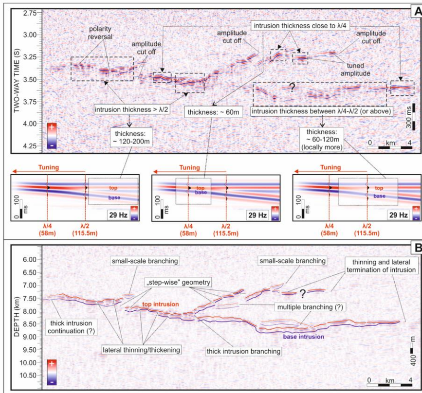
640 | Figure 167: Seismic interpretation of igneous intrusion imaged by profile PL-1200 (cf. Fig. 8). (A) PreSTM seismic profile with detailed interpretation of reflection amplitude and an estimation of intrusion thickness based on seismic tuning and vertical resolution criteria obtained from the wedge model analysis (Fig. 13). Three wedge models, calculated using zero-phase Ricker wavelet with 29 Hz dominant frequency, demonstrate various seismic responses depending on different sill thicknesses; (B) Part of 645 PreSDM PL-1200 profile that illustrates interpreted top and base of the intrusion and its inferred geometry.
