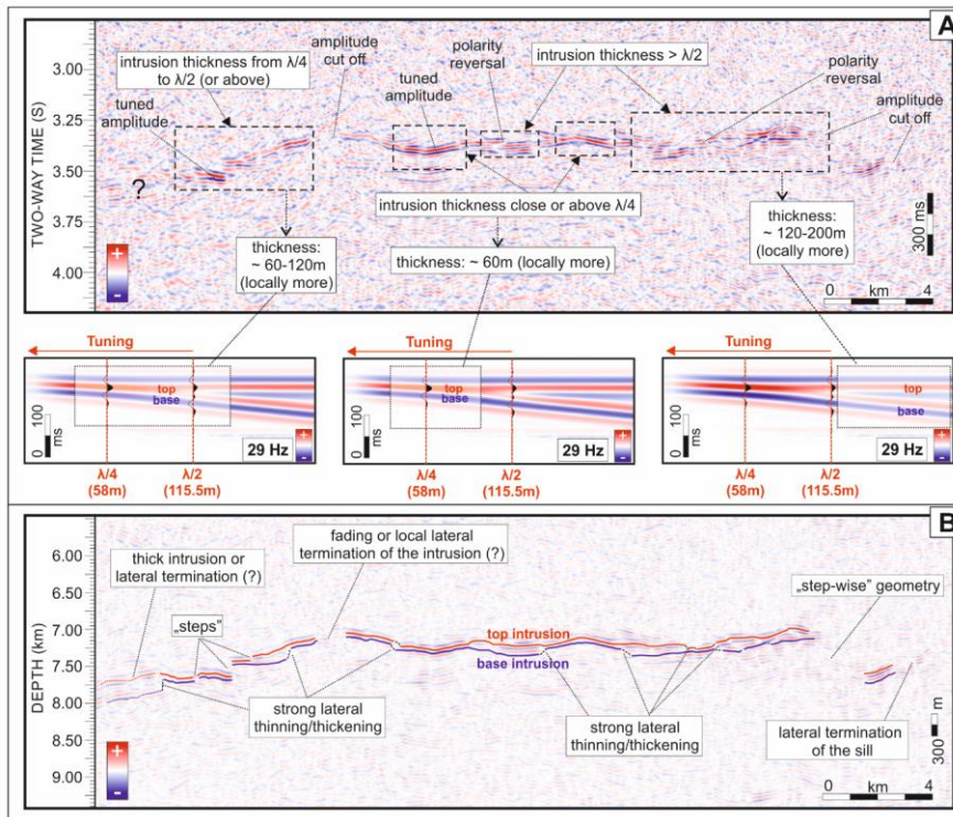
605 Figure 156: Seismic interpretation of igneous intrusion imaged by profile PL-5400, part 2 (cf. Fig. 7). (A) PreSTM seismic profile with detailed interpretation of reflection amplitude and an estimation of intrusion thickness based on seismic tuning and vertical resolution criteria obtained from the wedge model analysis (Fig. 13). Three wedge models, calculated using zero-phase Ricker wavelet with 29 Hz dominant frequency, demonstrate various seismic responses depending on different sill thicknesses; (B) Part of PreSDM PL-5400 profile that illustrates interpreted top and base of the intrusion and its inferred geometry.
