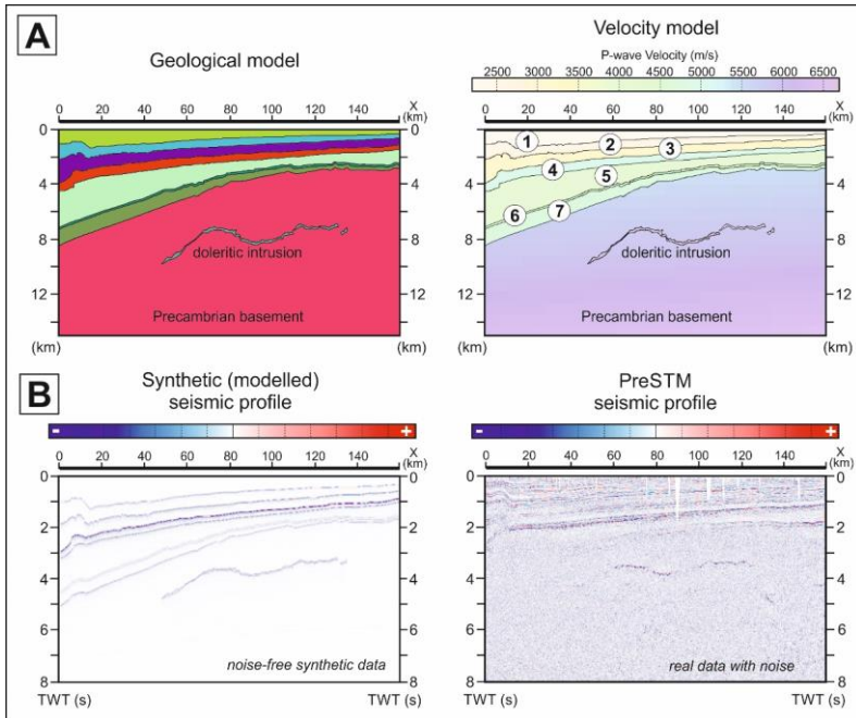
465 Figure 12: 2D seismic modeling for profile PL-5400 - dolerite scenario. (A) Left - geological model based on interpreted PL-5400 profile; right - P-wave velocity model: (1) Cretaceous and Cenozoic: velocity 2200 m/s, density 2.1 g/cm 3 , (2) Jurassic: velocity 2500 m/s, density 2.2 g/cm 3 , (3) Triassic: velocity 3200 m/s, density 2.23 g/cm 3 , (4) Permian (Zechstein evaporites): velocity 5000 m/s, density 2.5 g/cm 3 , (5) Silurian: velocity 4000 m/s, density 2.35 g/cm 3 , (6) Ordovician: velocity 4300 m/s, density 2.4 g/cm 3 , (7) Cambrian: velocity 4750 m/s, density 2.5 g/cm 3 , Precambrian basement: vertical velocity gradient 5500–6500 m/s, density gradient 2.58–2.81 g/cm 3 , doleritic intrusion: velocity 6700 m/s and density: 2.87 g/cm 3 (Brown and Kim, 2020); (B) Comparison of synthetic profile and real PreSTM seismic profile. 470
