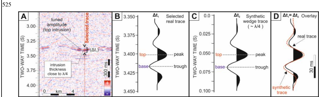
530 Figure 14: Comparison between observed and synthetic seismic responses of the inferred intrusion. (A) Location of the selected trace on seismic profile PL-5400, part 2 (trace interpreted as corresponding to an intrusion thickness close to the maximum tuning thickness ( \approx \lambda/4 ), based on the analysed tuning response; see polygon 2 in Fig. 7). (B) Real seismic trace displayed in variable-area wiggle format, extracted from the intrusion interval, where the main peak and trough correspond to reflections from the intrusion top and base, respectively. (C) Synthetic trace extracted from the wedge model for a thickness of \sim 58 m (close to the estimated tuning thickness, \lambda/4 ; see Fig. 13), using a zero-phase 29 Hz Ricker wavelet. (D) Overlay of real (black) and synthetic (red dashed) traces. All traces are displayed using identical two-way time windows (100 ms) and consistent amplitude scaling.
