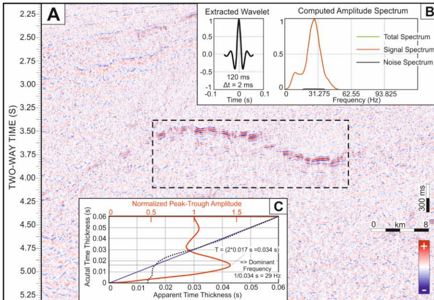
360 Figure 6: Seismic tuning analysis for polygon 1. (A) Enlarged part of PL-5400 seismic profile that illustrates detailed seismic expression of inferred igneous intrusion within the crystalline basement of the Baltic Basin (cf. Fig. 3). Black dotted rectangle indicates seismic wavelet extraction window for tuning analysis. (B) Extracted wavelet parameters with the computed amplitude spectrum. (C) Results of the seismic tuning analysis (tuning thickness chart) for the statistical wavelet extracted within a defined window, see text for additional explanation.
