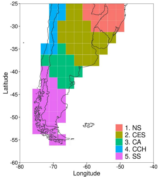
Figure 1: Regionalisation of SSA based on the co-occurrence of hot days during the warm seasons of 1979–2023. Grid points are 140 coloured and numbered from 1 to 5, according to the region they belong: C1—northern of SSA (NS), C2—central-eastern of SSA (CES), C3—central Argentina and northern Argentinian Patagonia (CA), C4—central Chile (CCH), C5—Argentinian Patagonia and southern Chile, southern SSA (SS).
