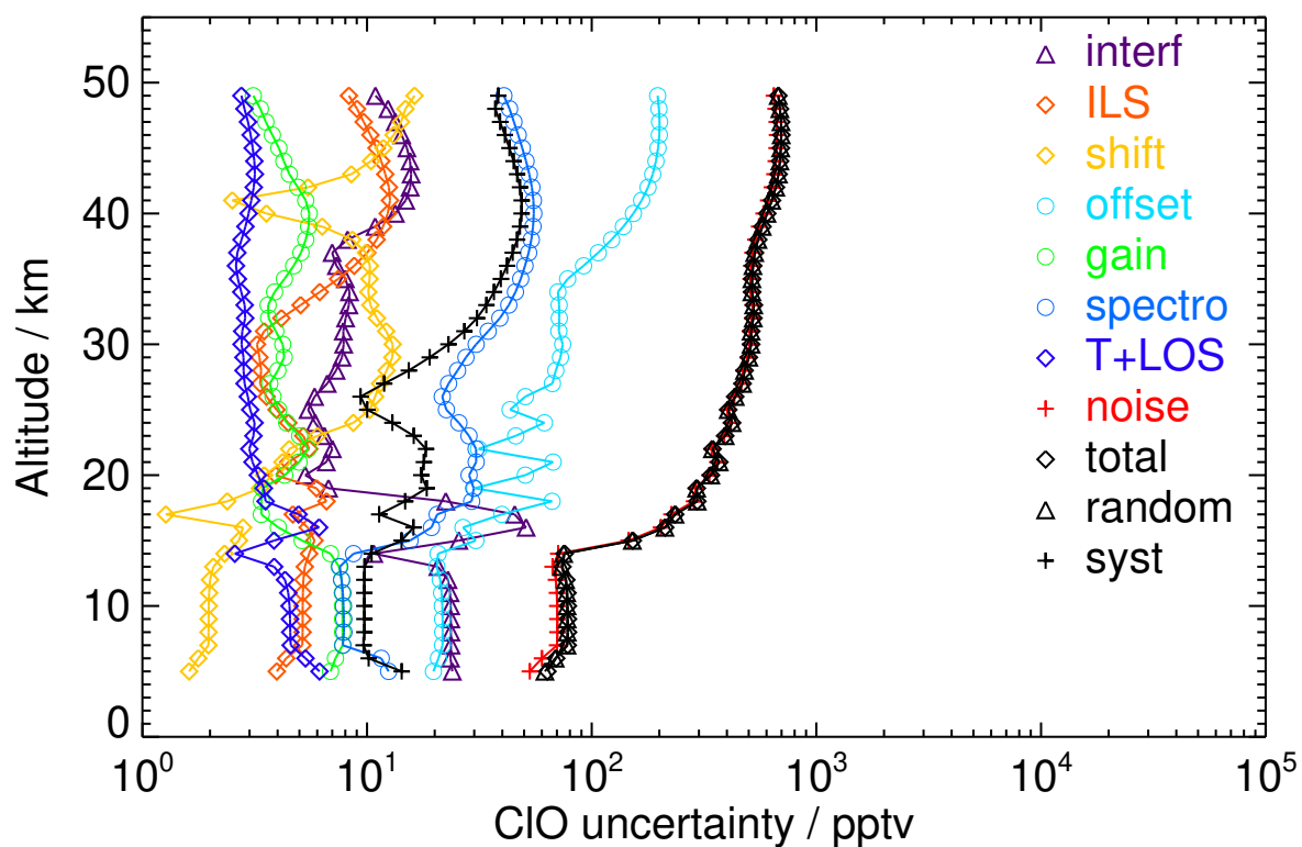
Figure S33. V8H_CLO_62 Southern polar autumn day
