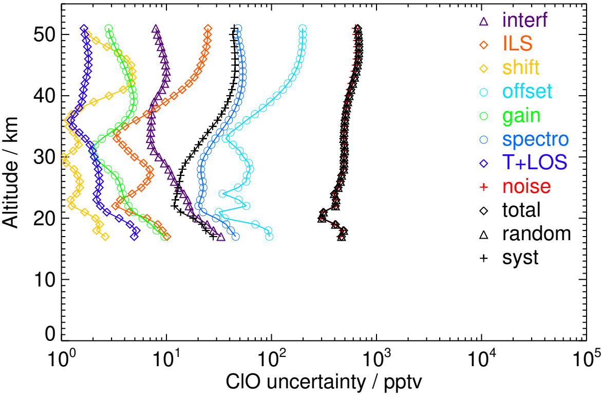
Figure S100. V8R_CLO_562 Southern polar summer night
