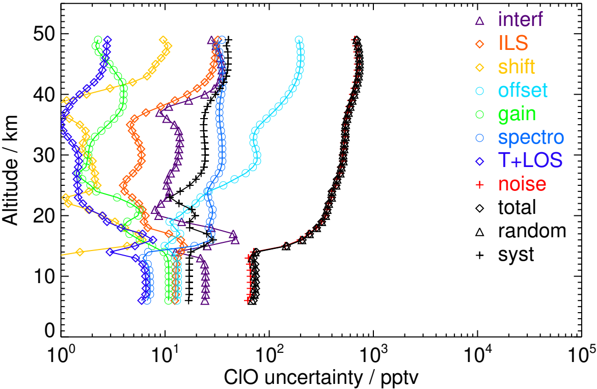
Figure S60. V8R_CLO_262 Southern midlatitude autumn night
