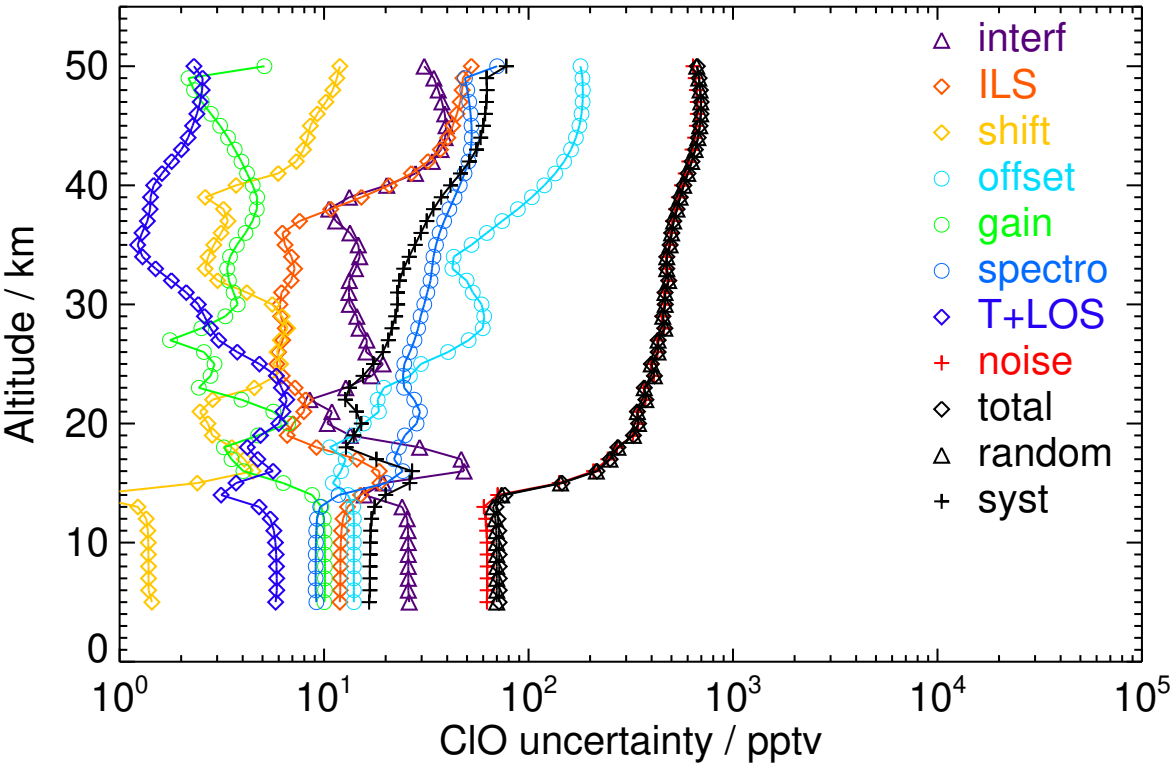
Figure S64. V8R_CLO_262 Southern polar spring night
