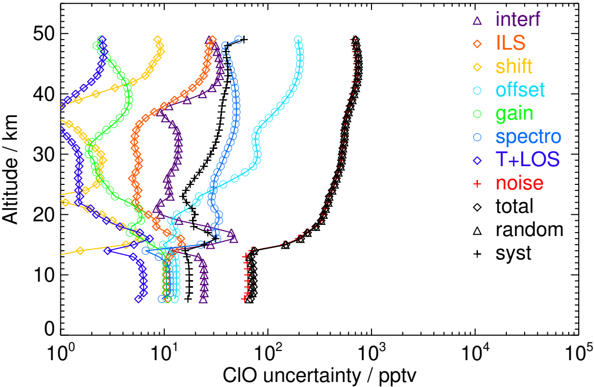
Figure S59. V8R_CLO_262 Southern midlatitude autumn day
