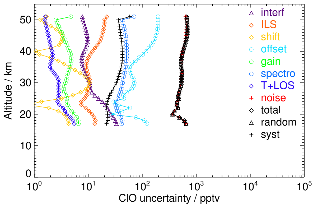
Figure S85. V8R_CLO_562 Tropics day
