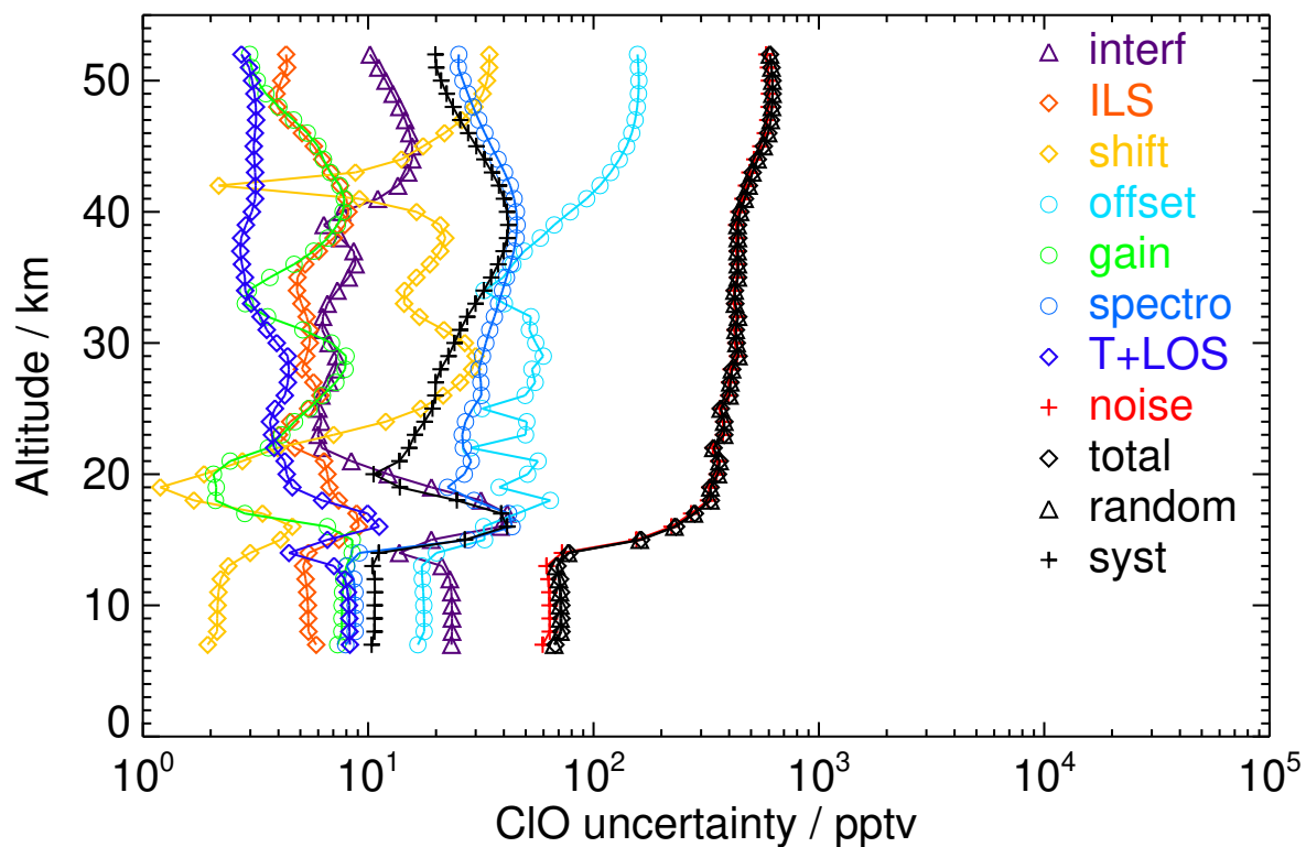
Figure S17. V8H_CLO_62 Tropics day
