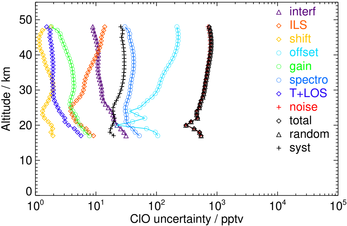
Figure S76. V8R_CLO_562 Northern polar autumn night
