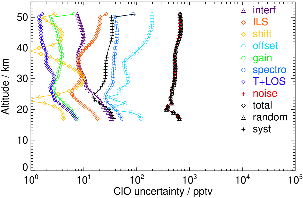
Figure S86. V8R_CLO_562 Tropics night
