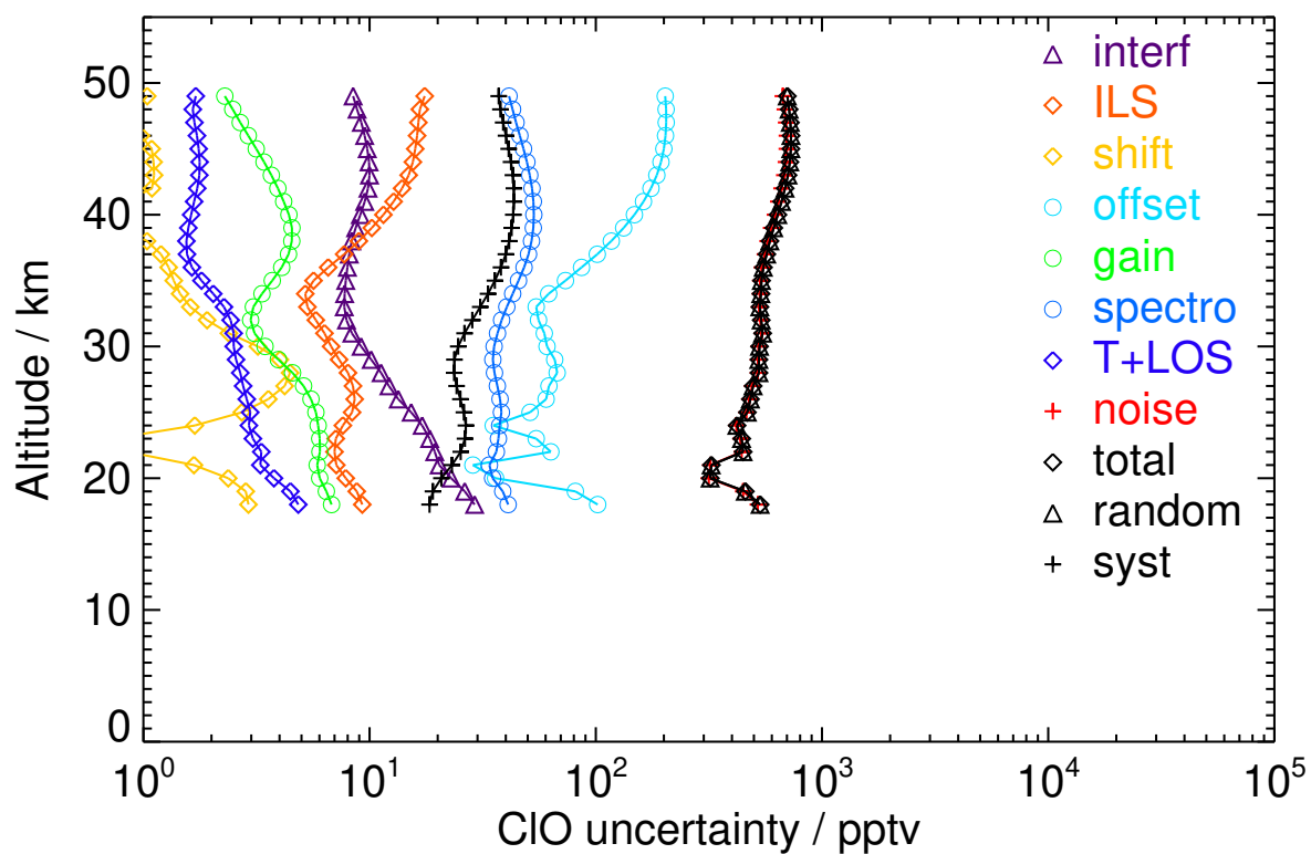
Figure S93. V8R_CLO_562 Southern midlatitude autumn day
