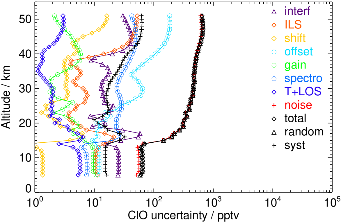
Figure S66. V8R_CLO_262 Southern polar summer night
