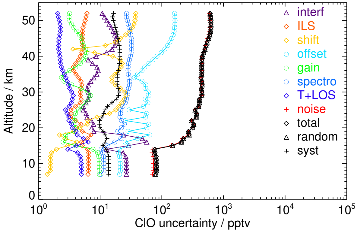
Figure S12. V8H_CLO_62 Northern midlatitude spring night
