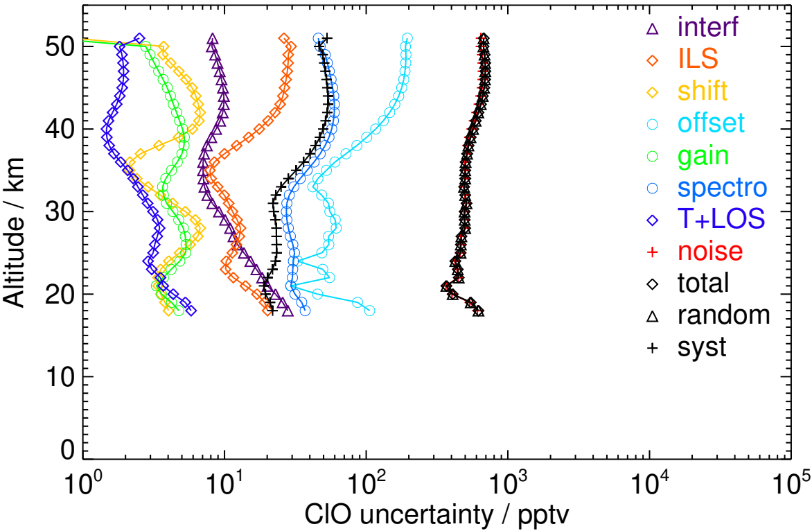
Figure S98. V8R_CLO_562 Southern polar spring night
