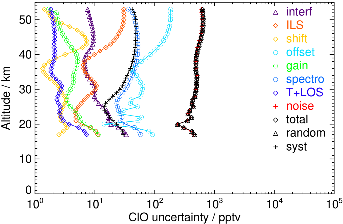
Figure S73. V8R_CLO_562 Northern polar summer day
