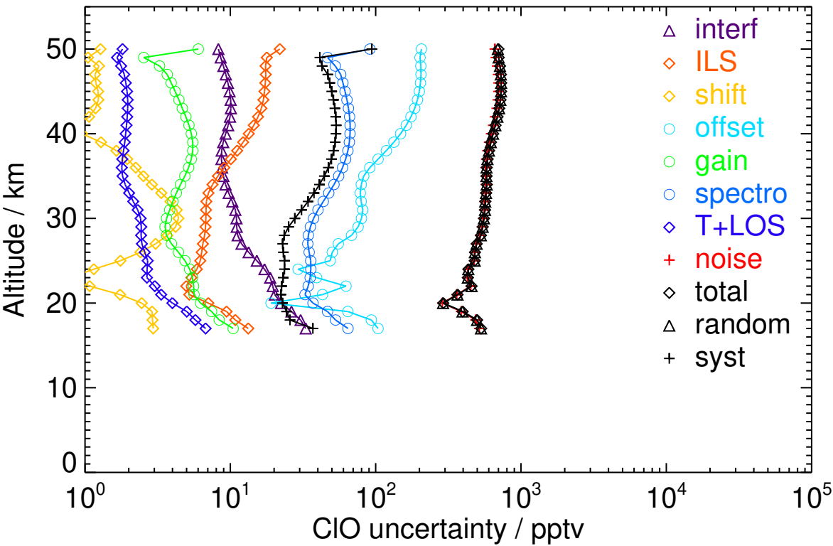
Figure S83. V8R_CLO_562 Northern midlatitude autumn day
