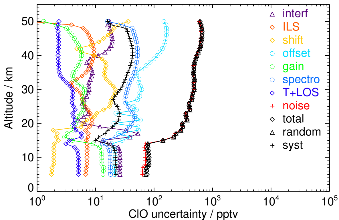
Figure S9. V8H_CLO_62 Northern midlatitude winter day
