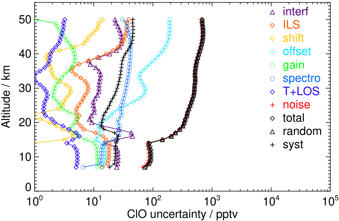
Figure S46. V8R_CLO_262 Northern midlatitude spring night
