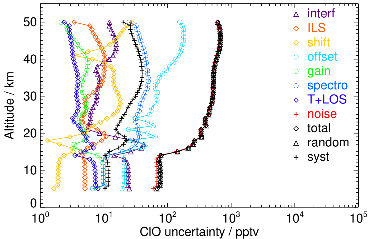
Figure S19. V8H_CLO_62 Southern midlatitude winter day
