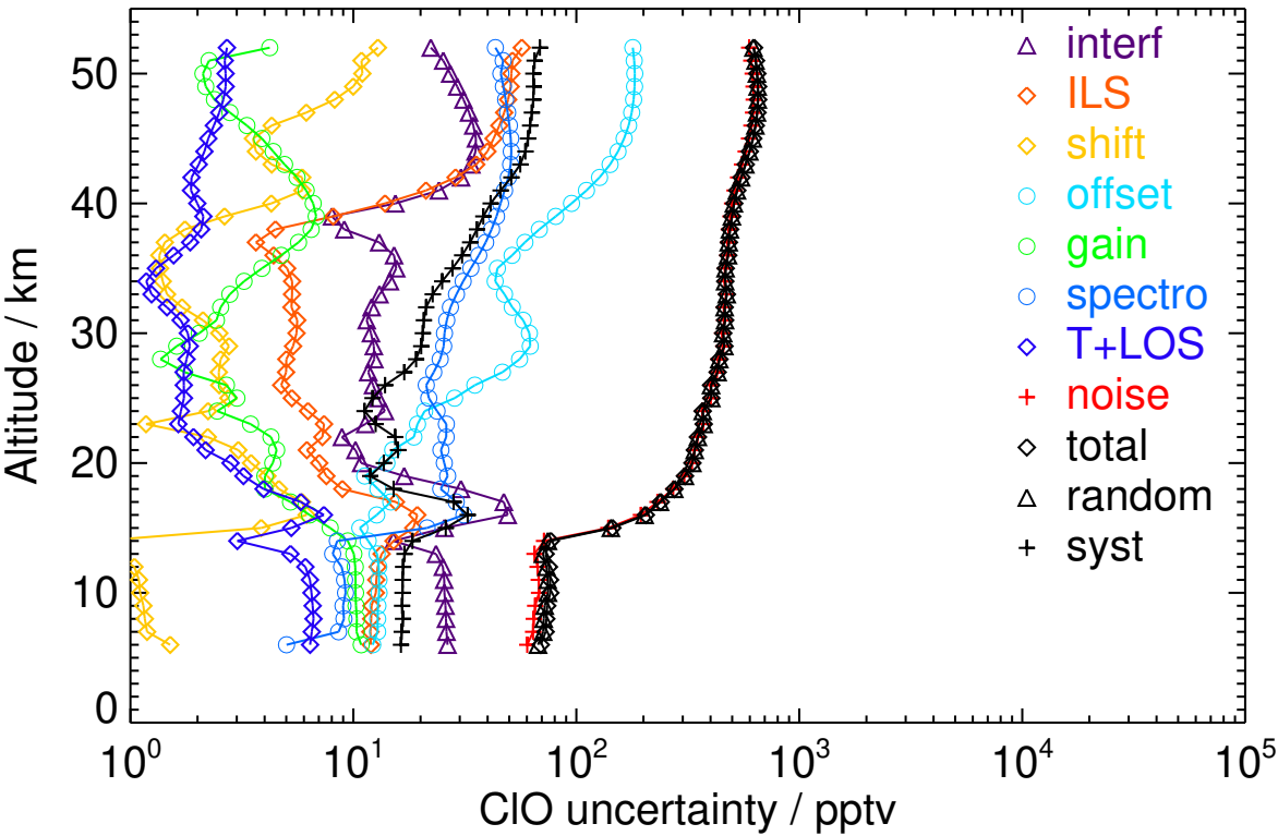
Figure S58. V8R_CLO_262 Southern midlatitude summer night
