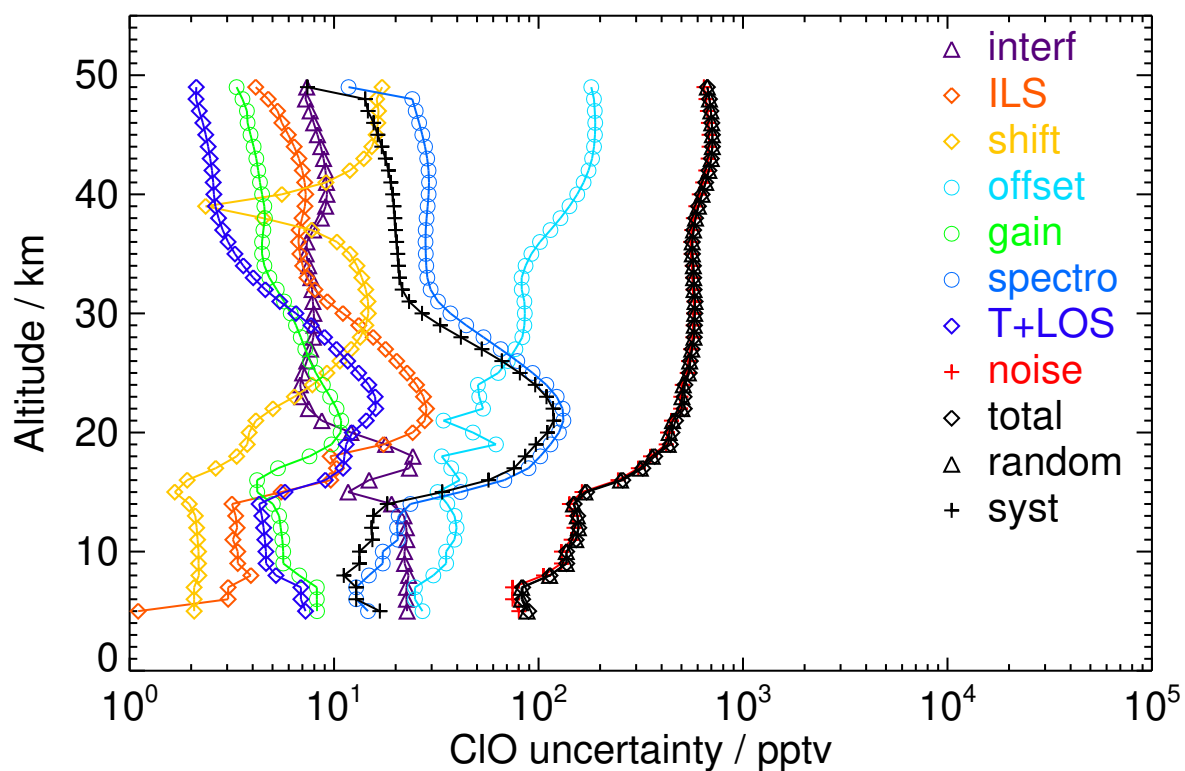
Figure S27. V8H_CLO_62 Southern polar winter day
