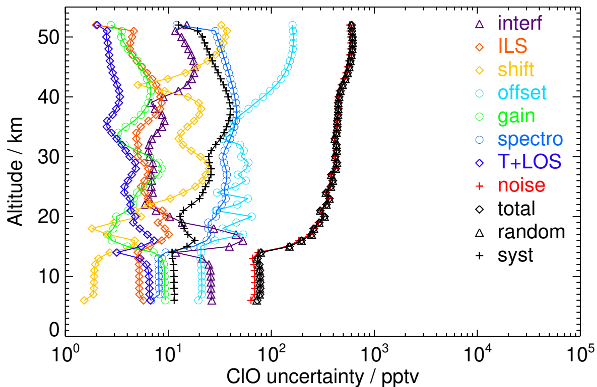
Figure S21. V8H_CLO_62 Southern midlatitude spring day
