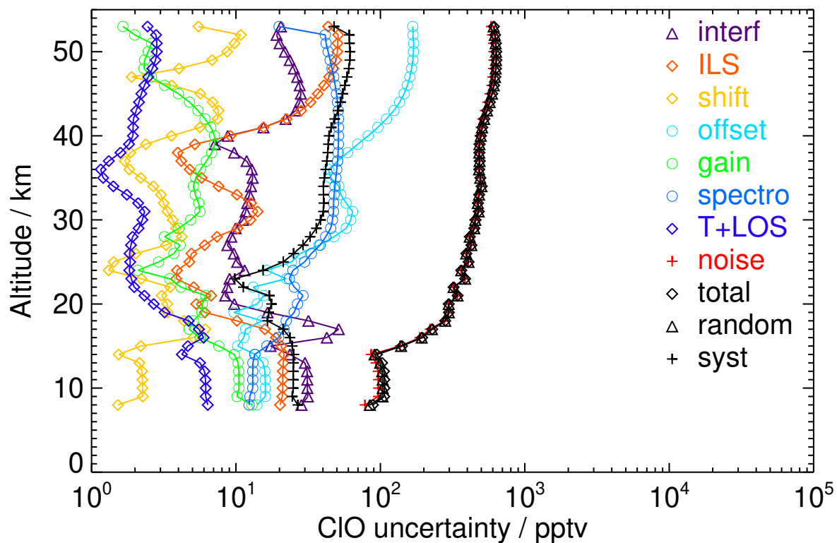
Figure S39. V8R_CLO_262 Northern polar summer day
