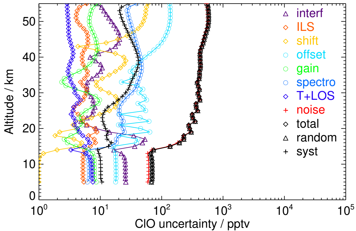
Figure S31. V8H_CLO_62 Southern polar summer day
