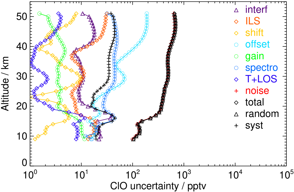
Figure S51. V8R_CLO_262 Tropics day
