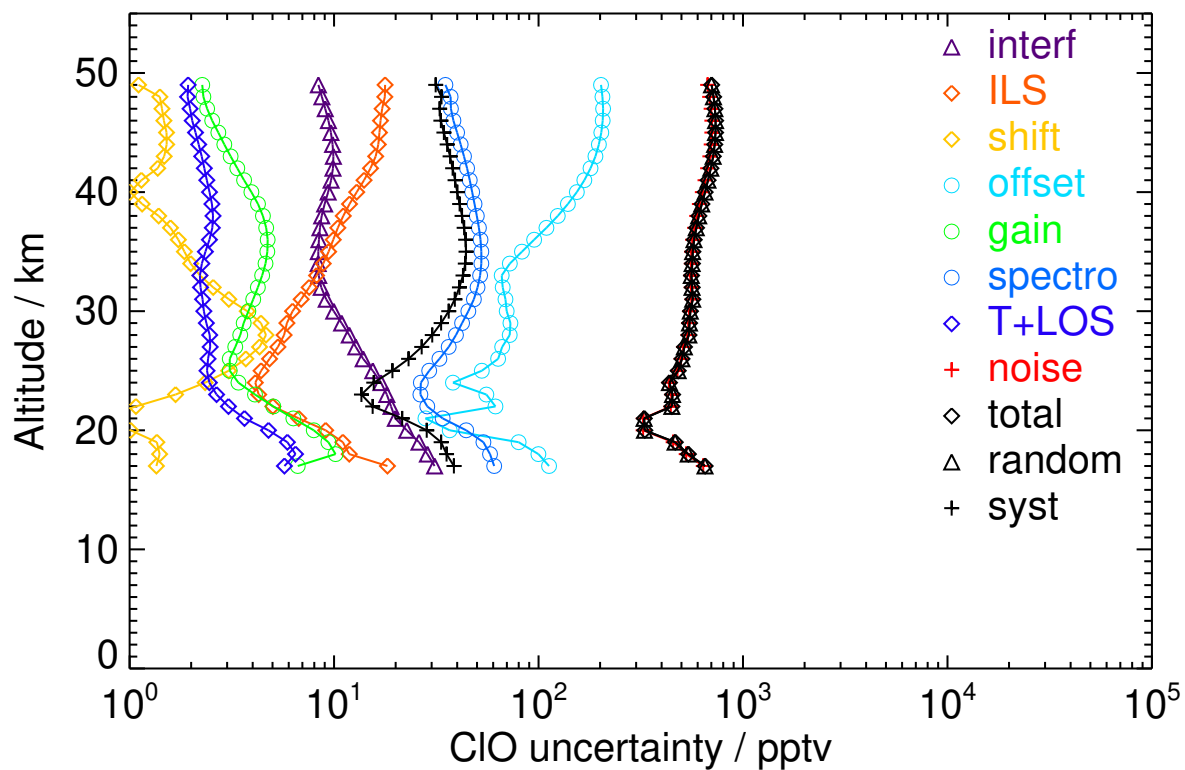
Figure S87. V8R_CLO_562 Southern midlatitude winter day
