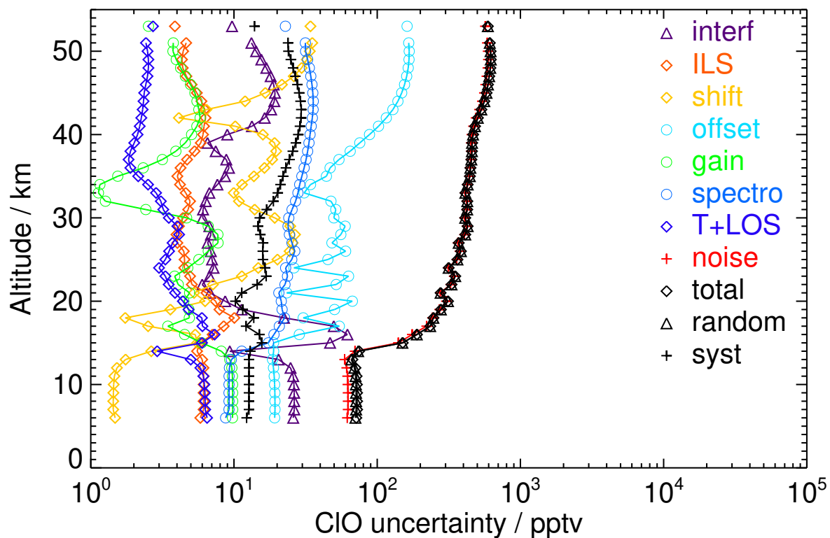
Figure S22. V8H_CLO_62 Southern midlatitude spring night
