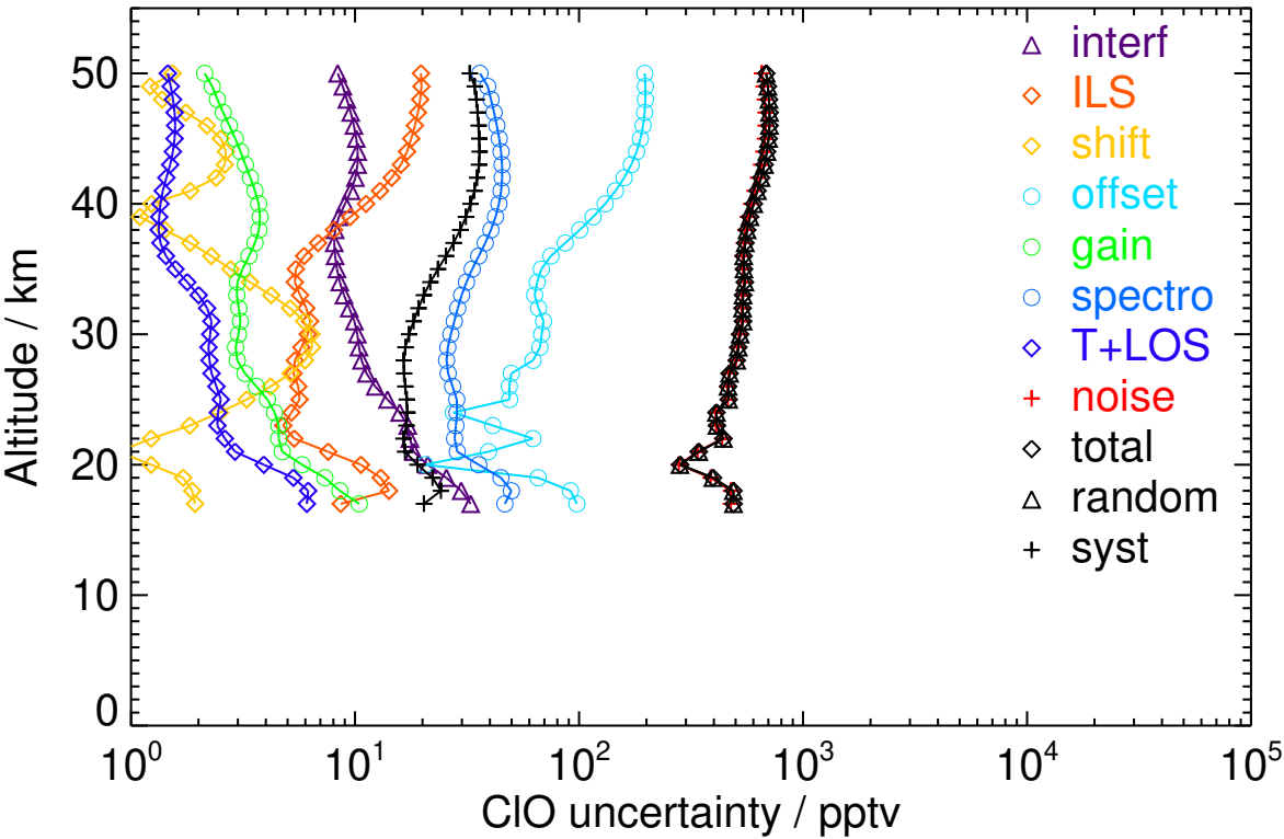
Figure S90. V8R_CLO_562 Southern midlatitude spring night
