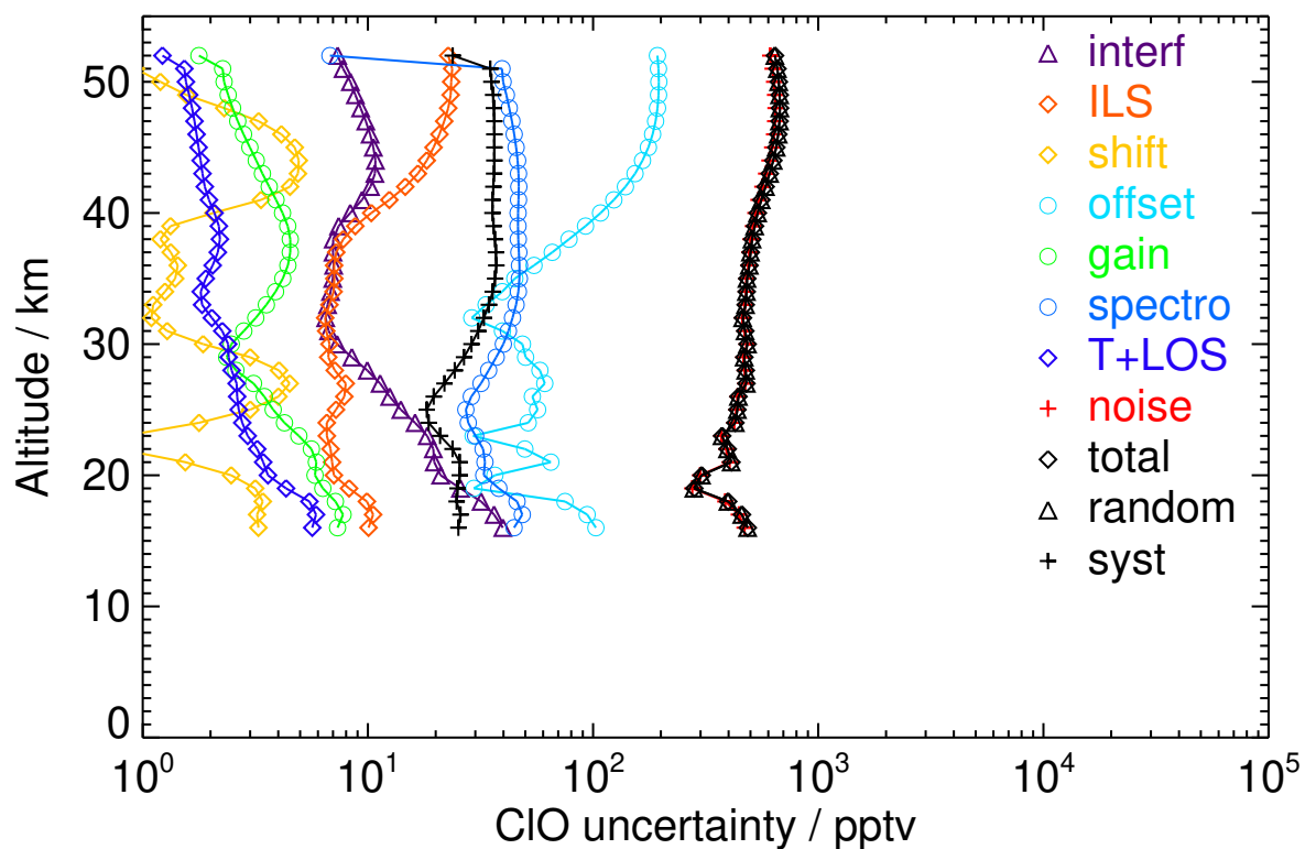
Figure S91. V8R_CLO_562 Southern midlatitude summer day
