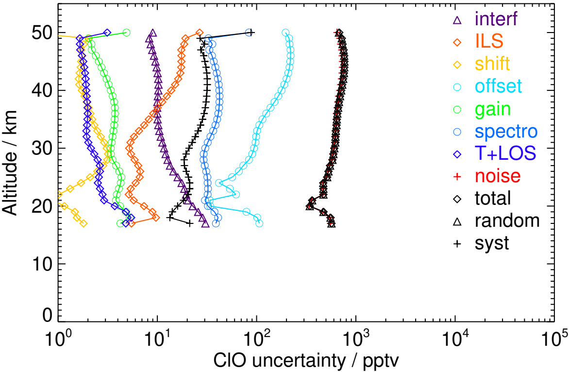
Figure S88. V8R_CLO_562 Southern midlatitude winter night
