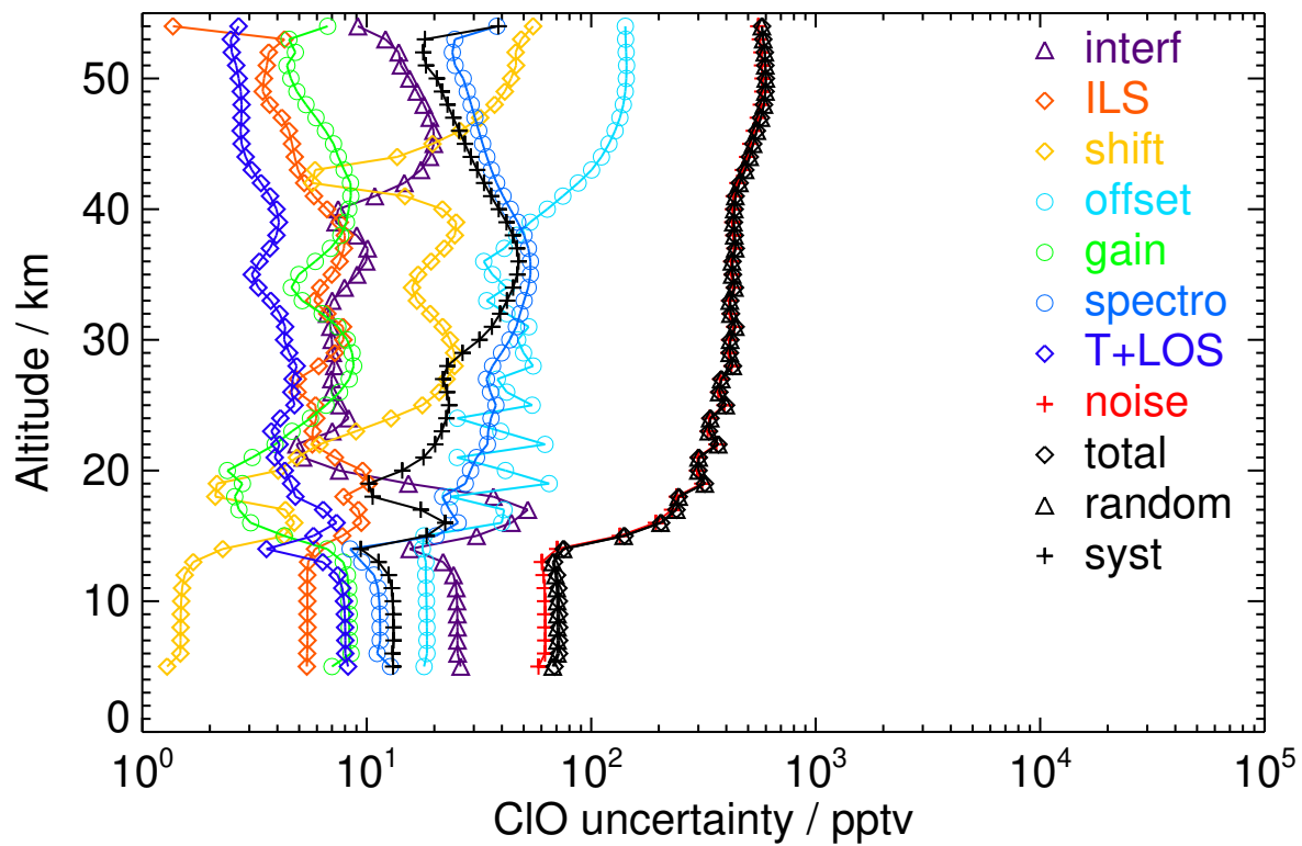
Figure S23. V8H_CLO_62 Southern midlatitude summer day
