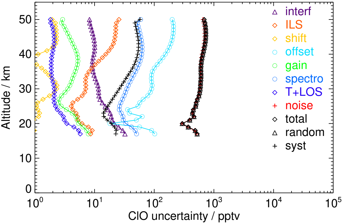
Figure S72. V8R_CLO_562 Northern polar spring night
