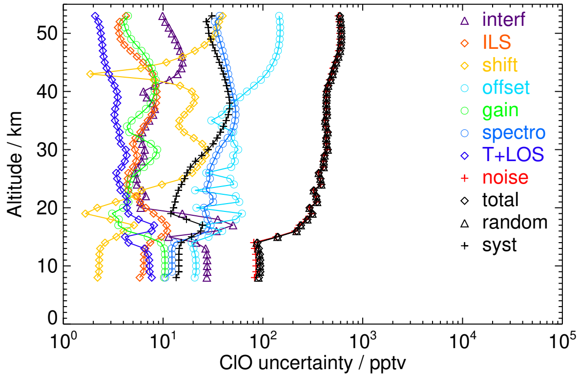
Figure S13. V8H_CLO_62 Northern midlatitude summer day
