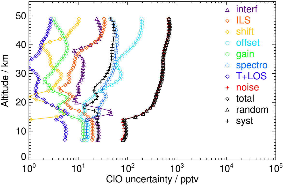
Figure S45. V8R_CLO_262 Northern midlatitude spring day
