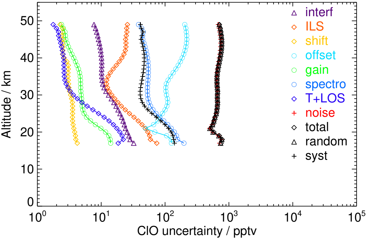
Figure S95. V8R_CLO_562 Southern polar winter day
