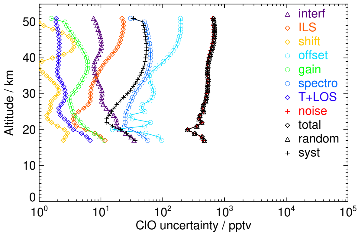
Figure S74. V8R_CLO_562 Northern polar summer night
