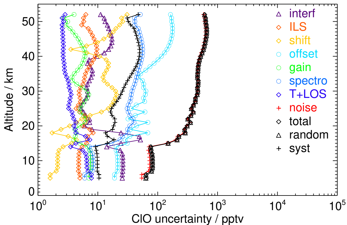
Figure S25. V8H_CLO_62 Southern midlatitude autumn day
