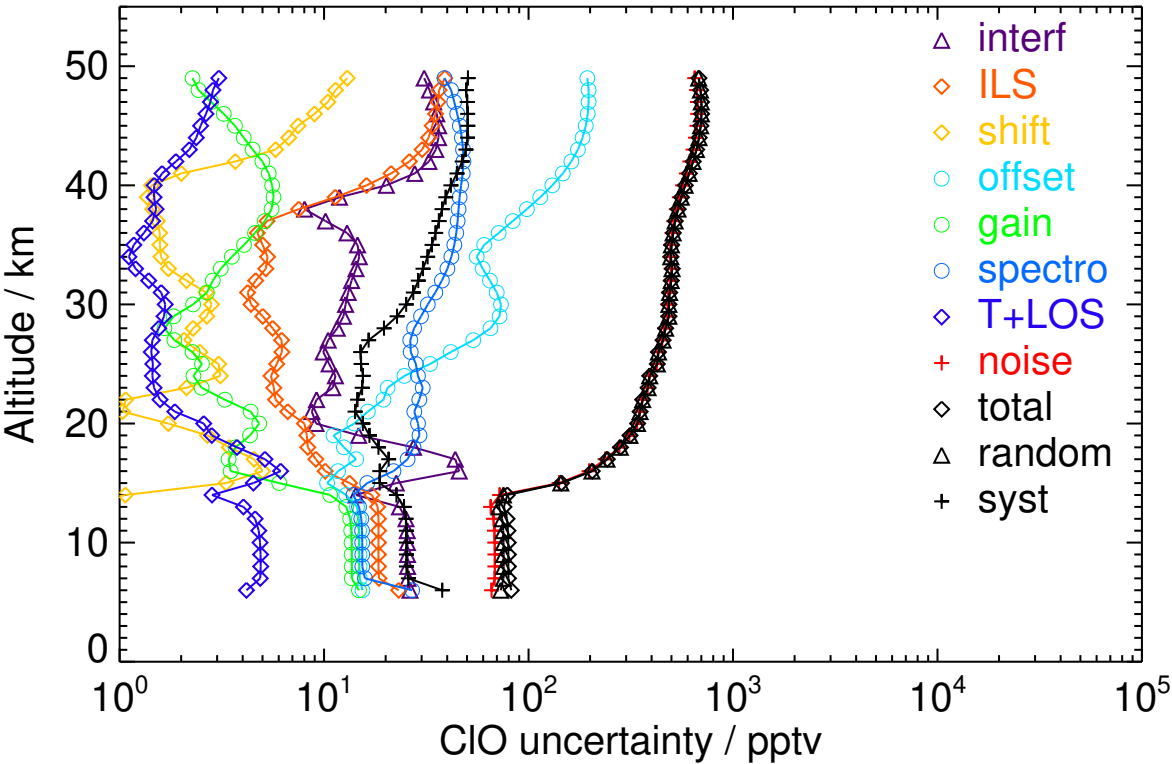
Figure S44. V8R_CLO_262 Northern midlatitude winter night
