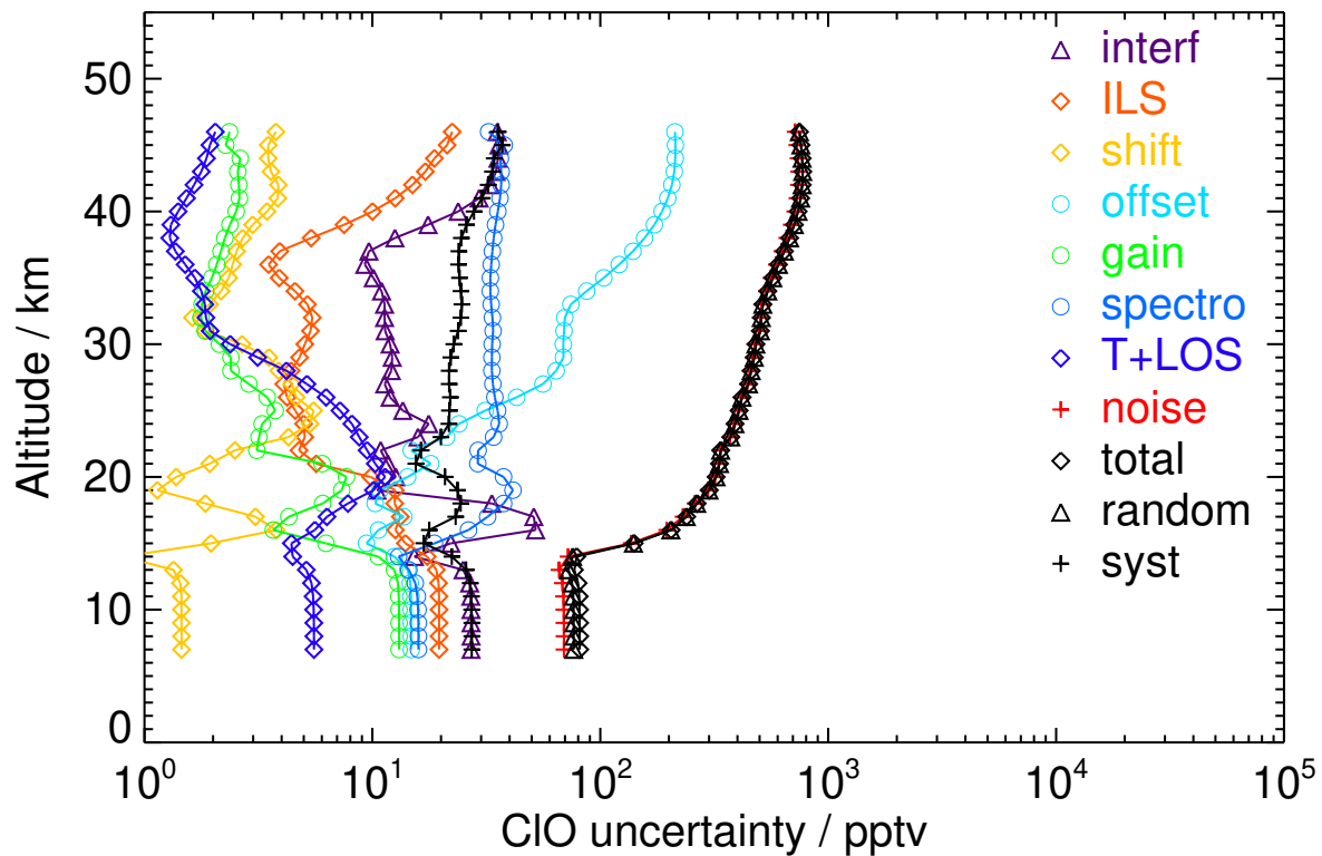
Figure S35. V8R_CLO_262 Northern polar winter day
