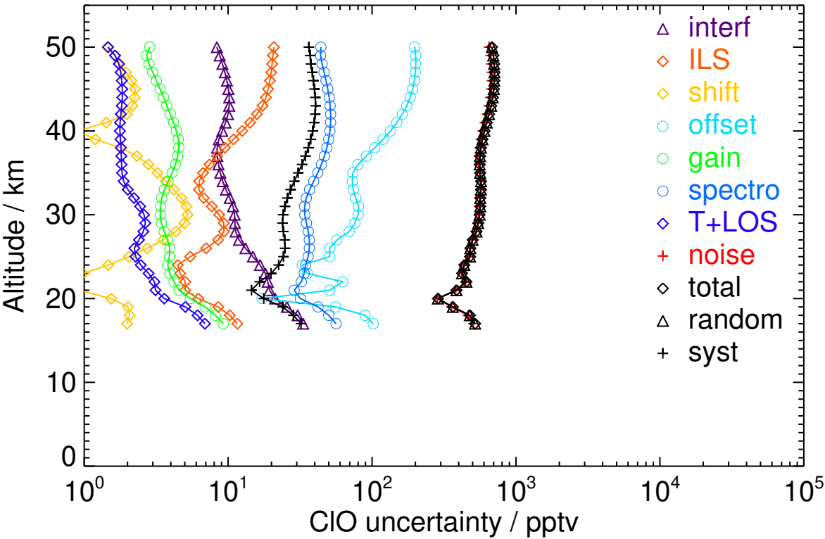
Figure S80. V8R_CLO_562 Northern midlatitude spring night
