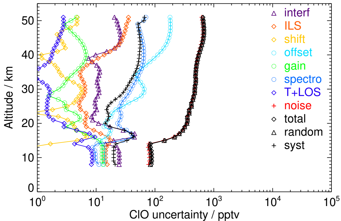
Figure S47. V8R_CLO_262 Northern midlatitude summer day
