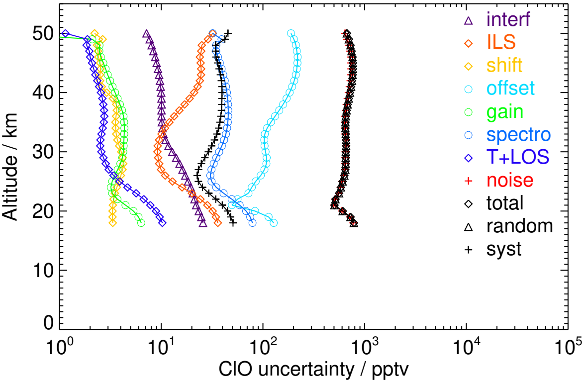
Figure S96. V8R_CLO_562 Southern polar winter night
