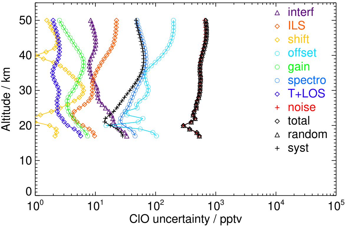
Figure S79. V8R_CLO_562 Northern midlatitude spring day
