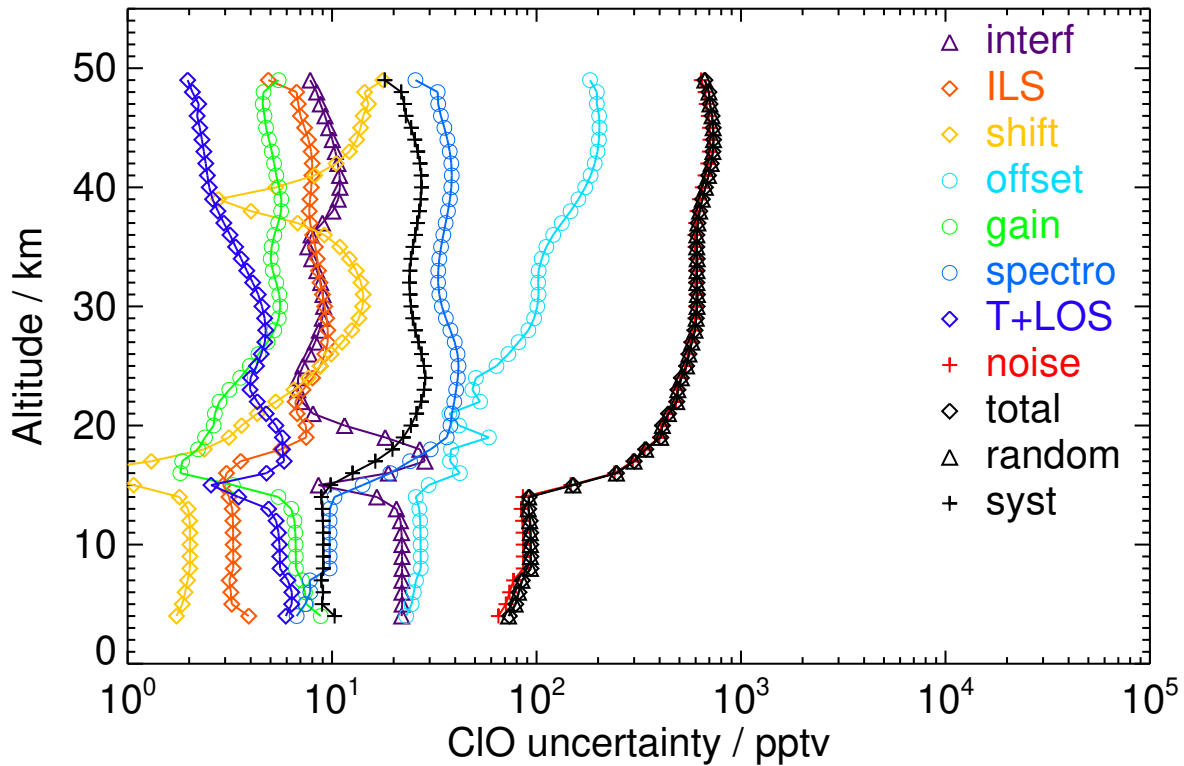
Figure S28. V8H_CLO_62 Southern polar winter night
