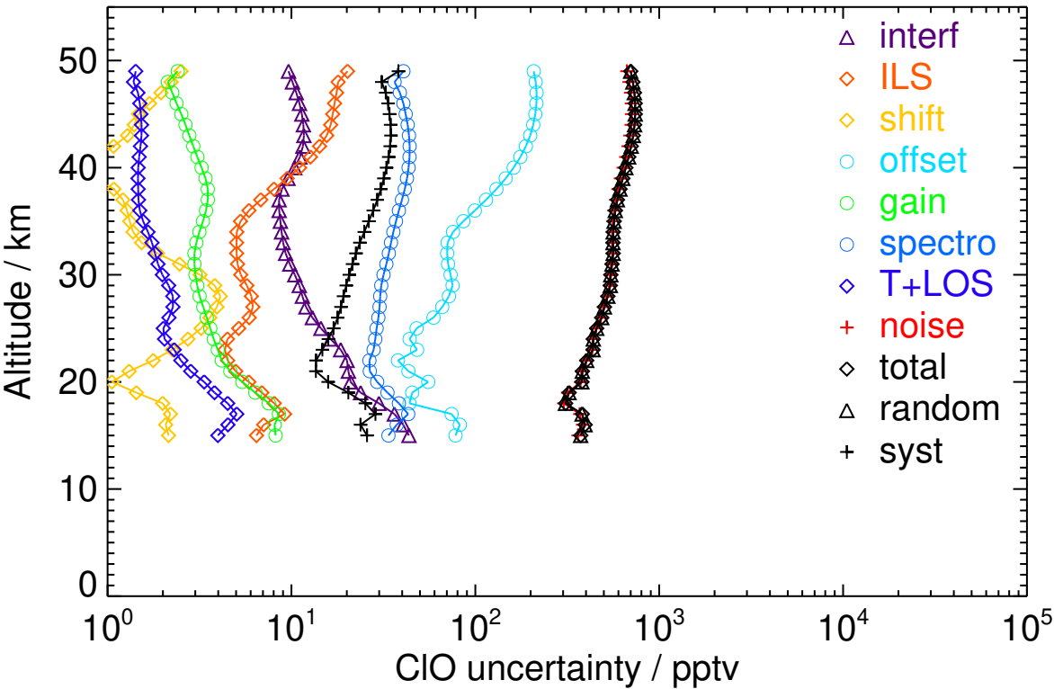
Figure S78. V8R_CLO_562 Northern midlatitude winter night
