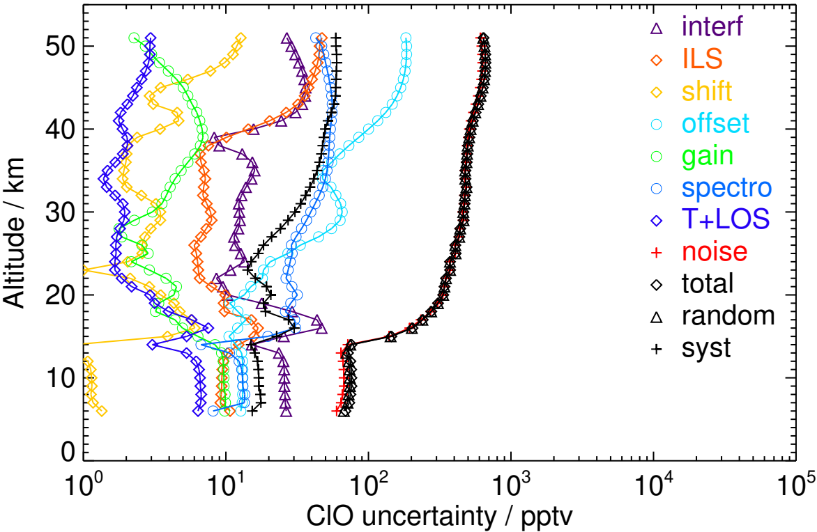
Figure S57. V8R_CLO_262 Southern midlatitude summer day
