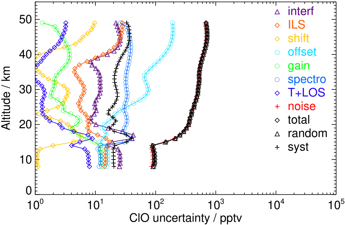
Figure S50. V8R_CLO_262 Northern midlatitude autumn night
