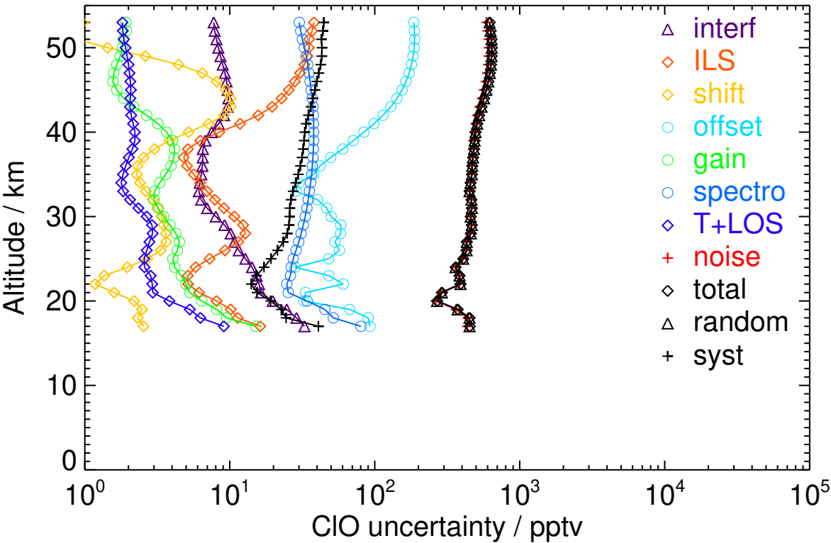
Figure S99. V8R_CLO_562 Southern polar summer day
