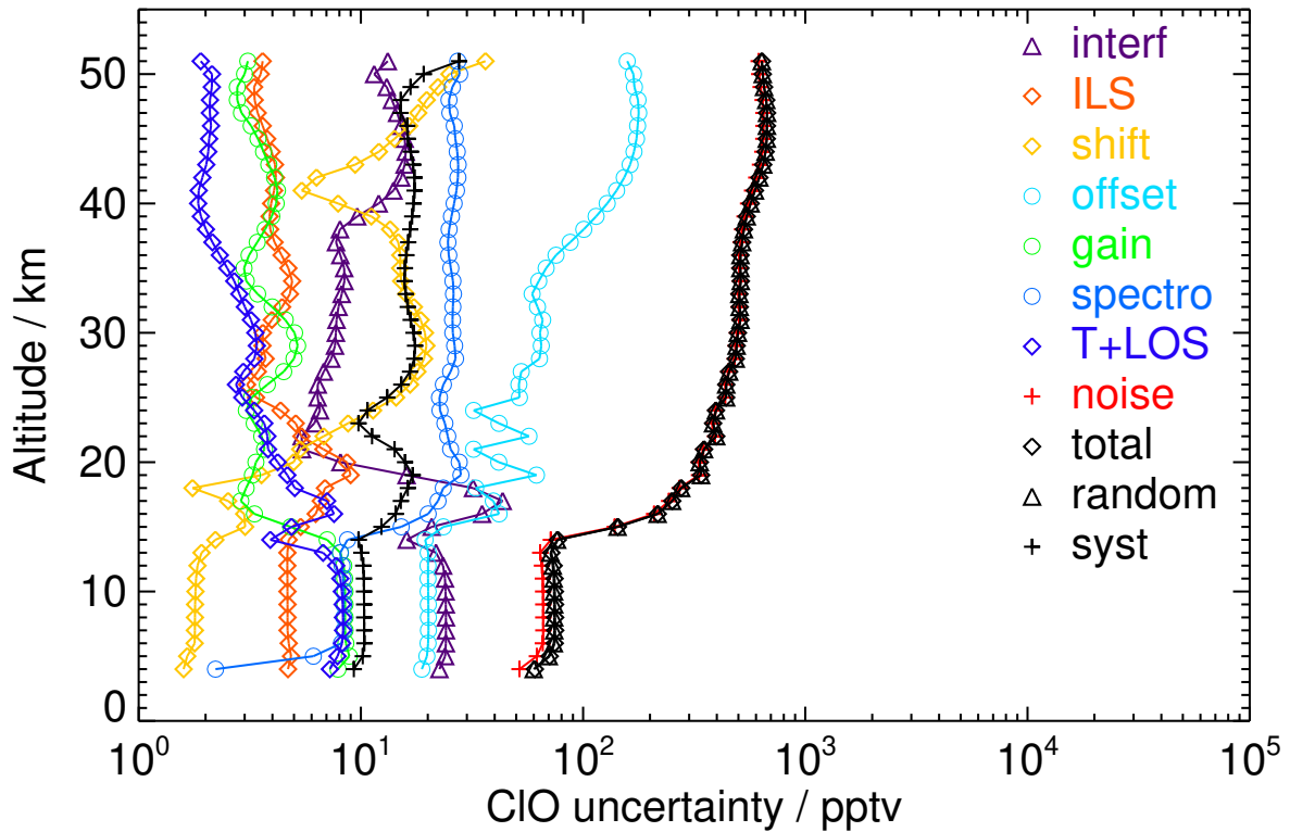
Figure S20. V8H_CLO_62 Southern midlatitude winter night
