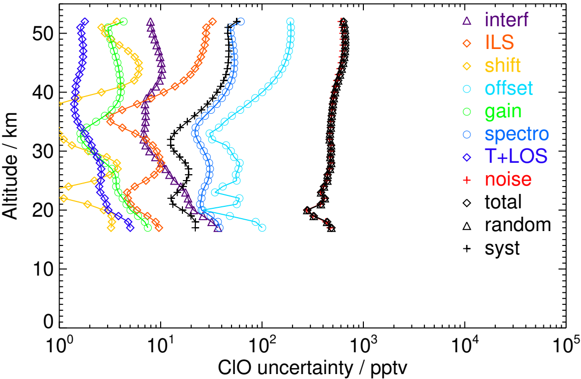
Figure S92. V8R_CLO_562 Southern midlatitude summer night
