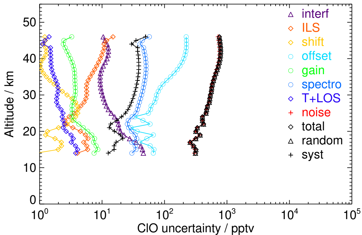
Figure S69. V8R_CLO_562 Northern polar winter day
