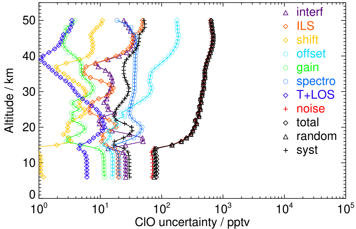
Figure S36. V8R_CLO_262 Northern polar winter night
