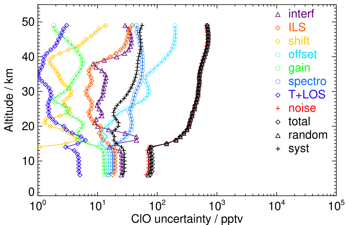
Figure S43. V8R_CLO_262 Northern midlatitude winter day
