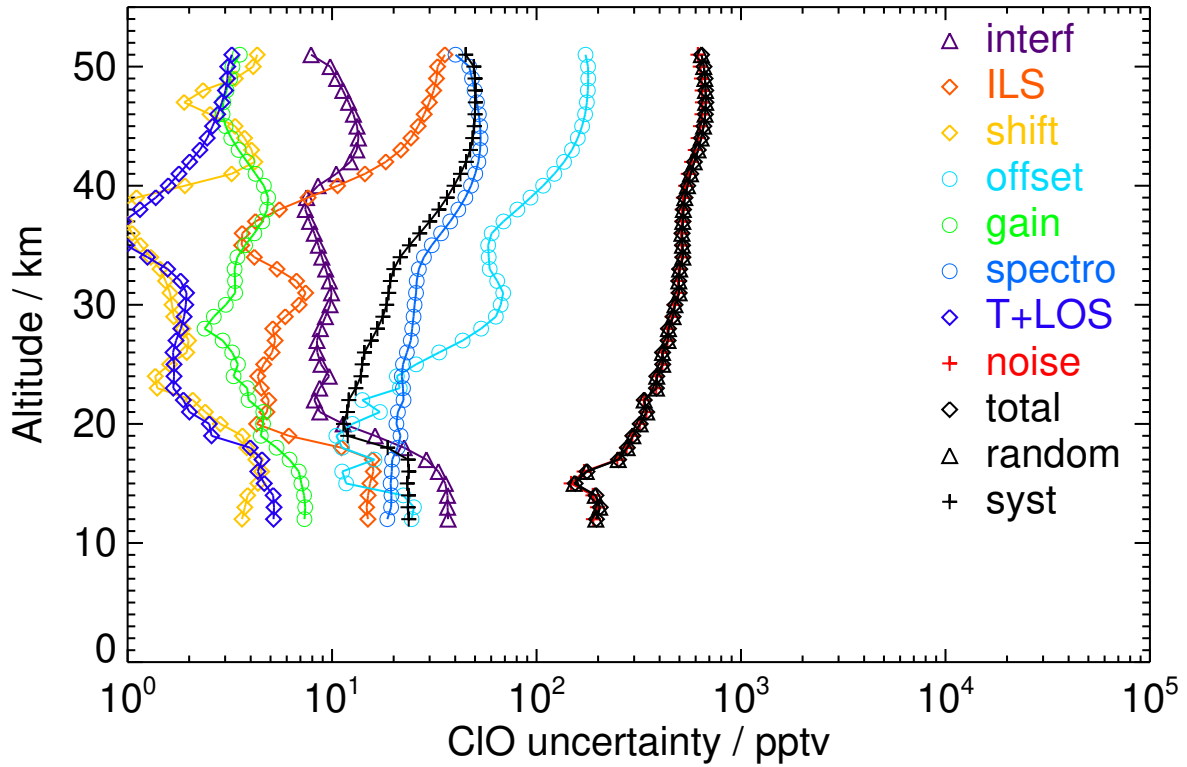
Figure S40. V8R_CLO_262 Northern polar summer night
