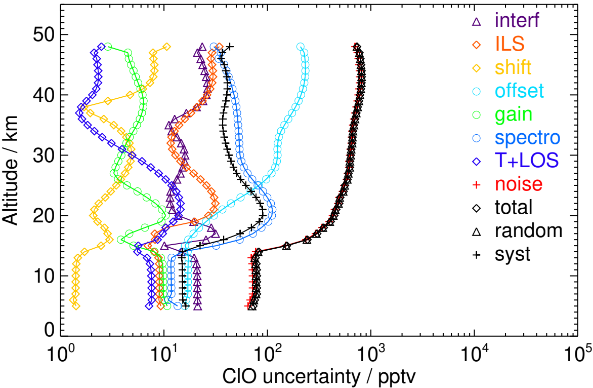
Figure S61. V8R_CLO_262 Southern polar winter day
