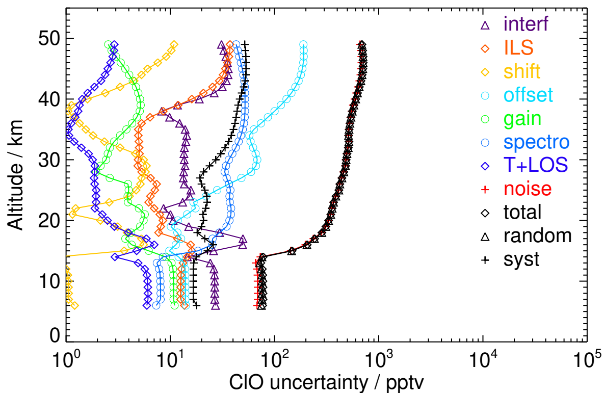
Figure S55. V8R_CLO_262 Southern midlatitude spring day
