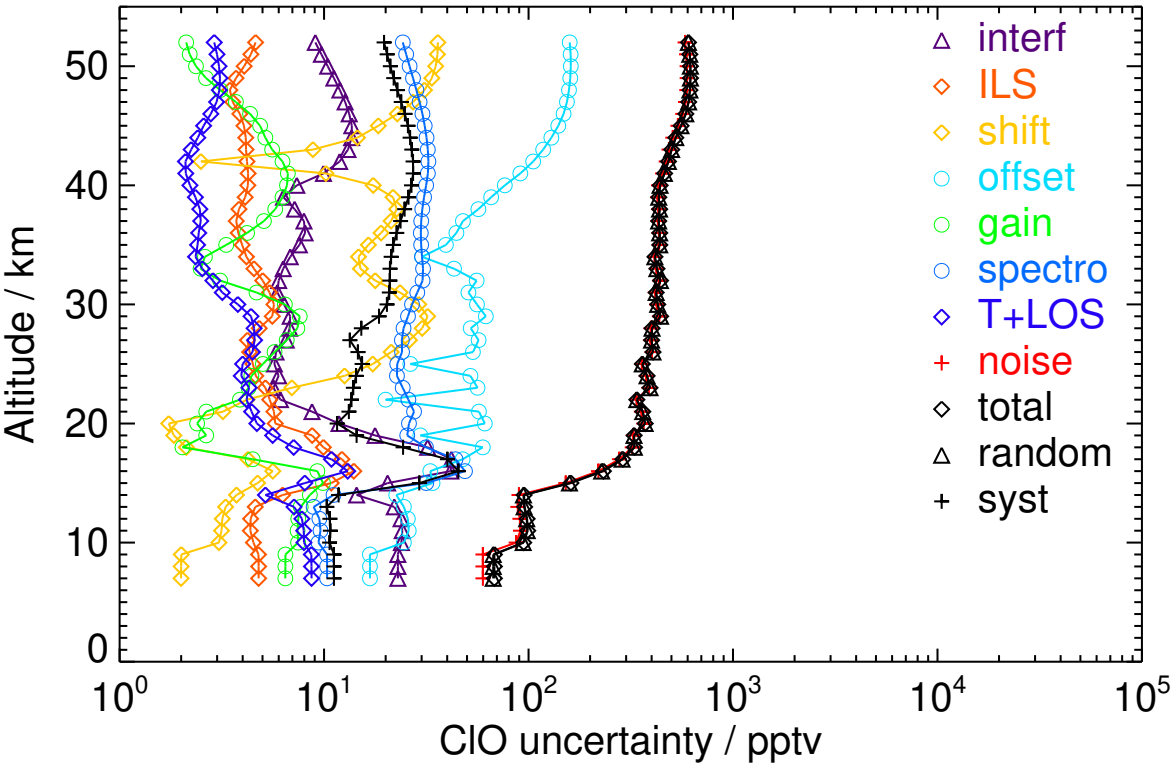
Figure S18. V8H_CLO_62 Tropics night
