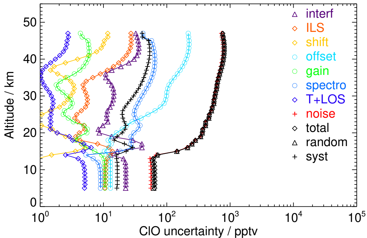
Figure S67. V8R_CLO_262 Southern polar autumn day
