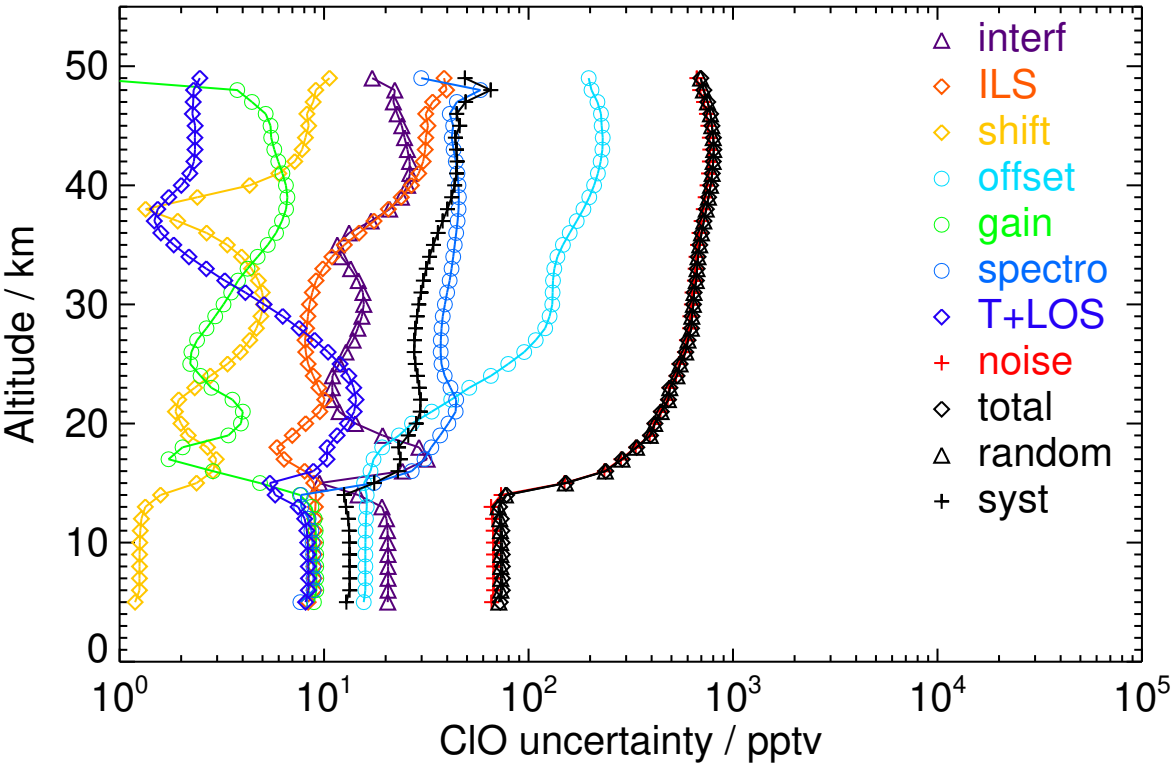
Figure S62. V8R_CLO_262 Southern polar winter night
