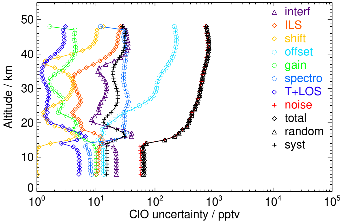
Figure S68. V8R_CLO_262 Southern polar autumn night
