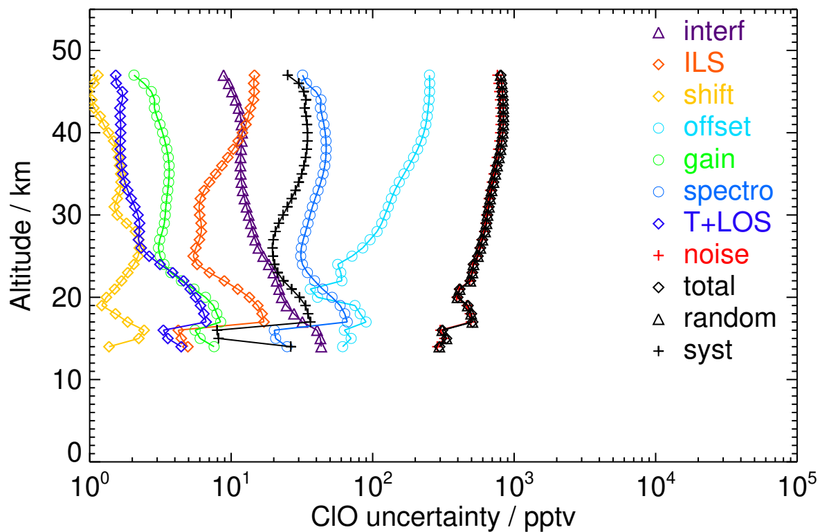
Figure S70. V8R_CLO_562 Northern polar winter night
