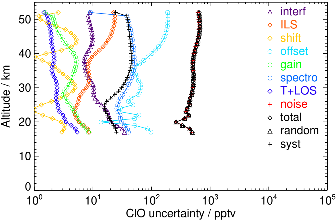
Figure S81. V8R_CLO_562 Northern midlatitude summer day
