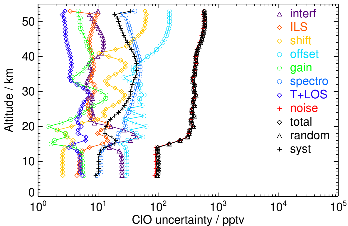
Figure S29. V8H_CLO_62 Southern polar spring day
