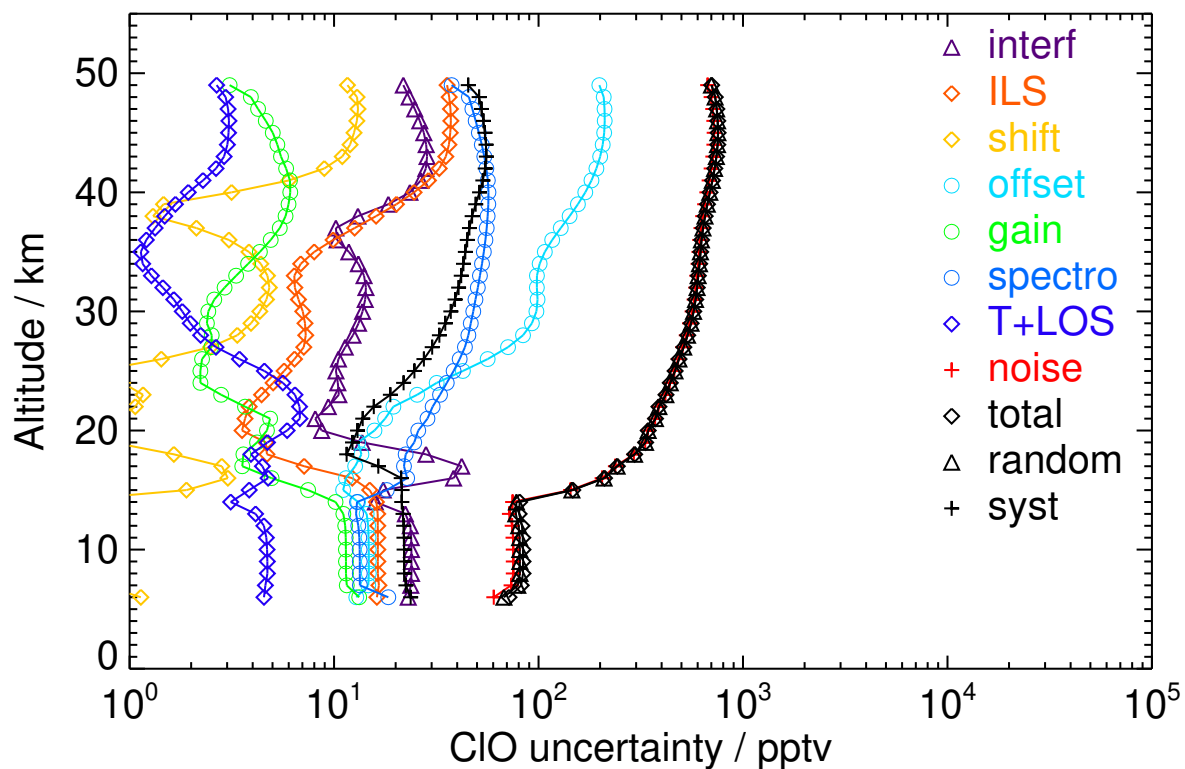
Figure S37. V8R_CLO_262 Northern polar spring day
