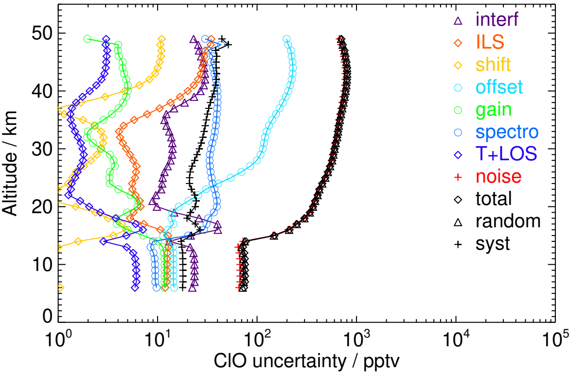
Figure S53. V8R_CLO_262 Southern midlatitude winter day
