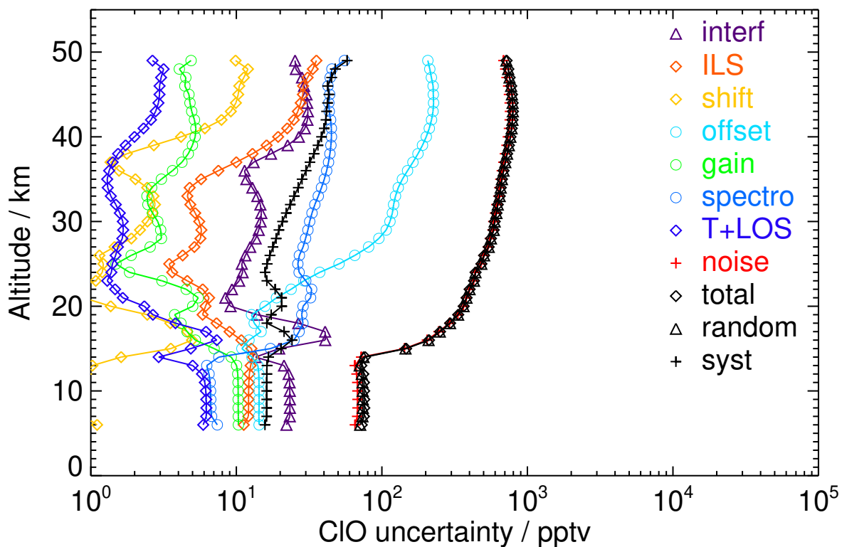
Figure S54. V8R_CLO_262 Southern midlatitude winter night
