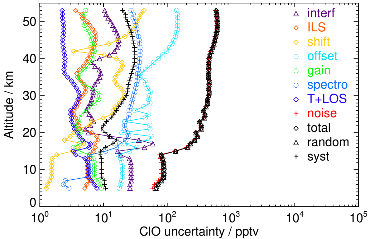
Figure S32. V8H_CLO_62 Southern polar summer night
