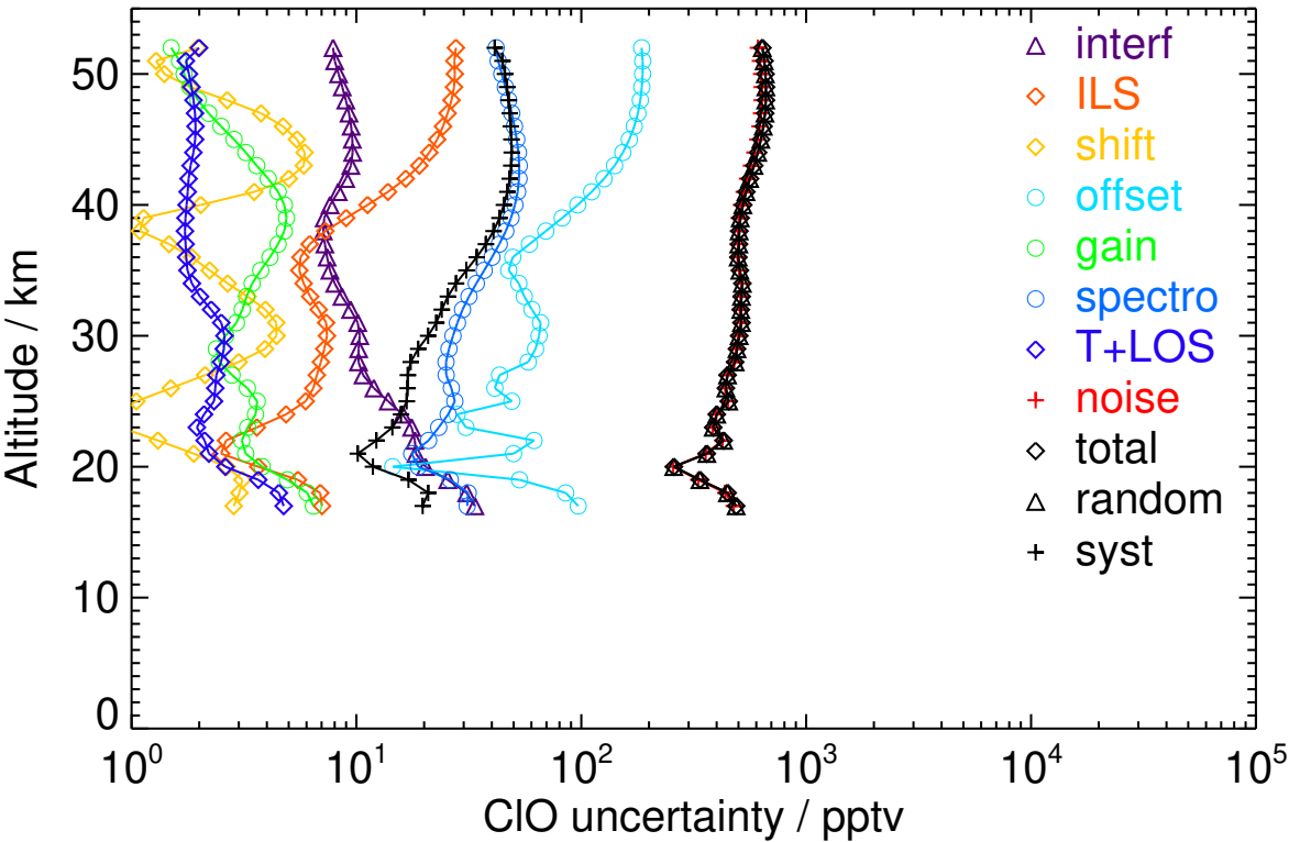
Figure S82. V8R_CLO_562 Northern midlatitude summer night
