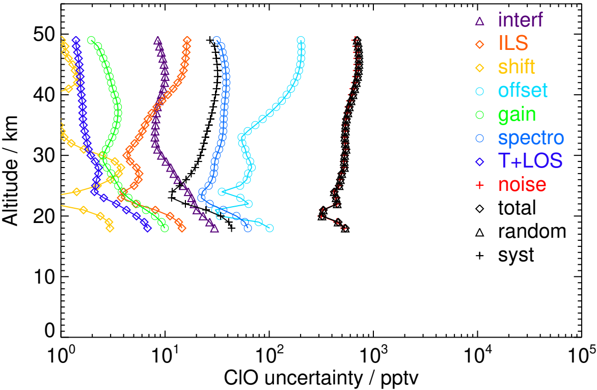
Figure S94. V8R_CLO_562 Southern midlatitude autumn night
