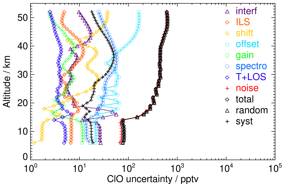
Figure S11. V8H_CLO_62 Northern midlatitude spring day
