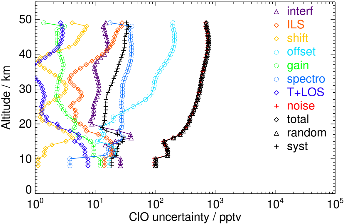
Figure S42. V8R_CLO_262 Northern polar autumn night
