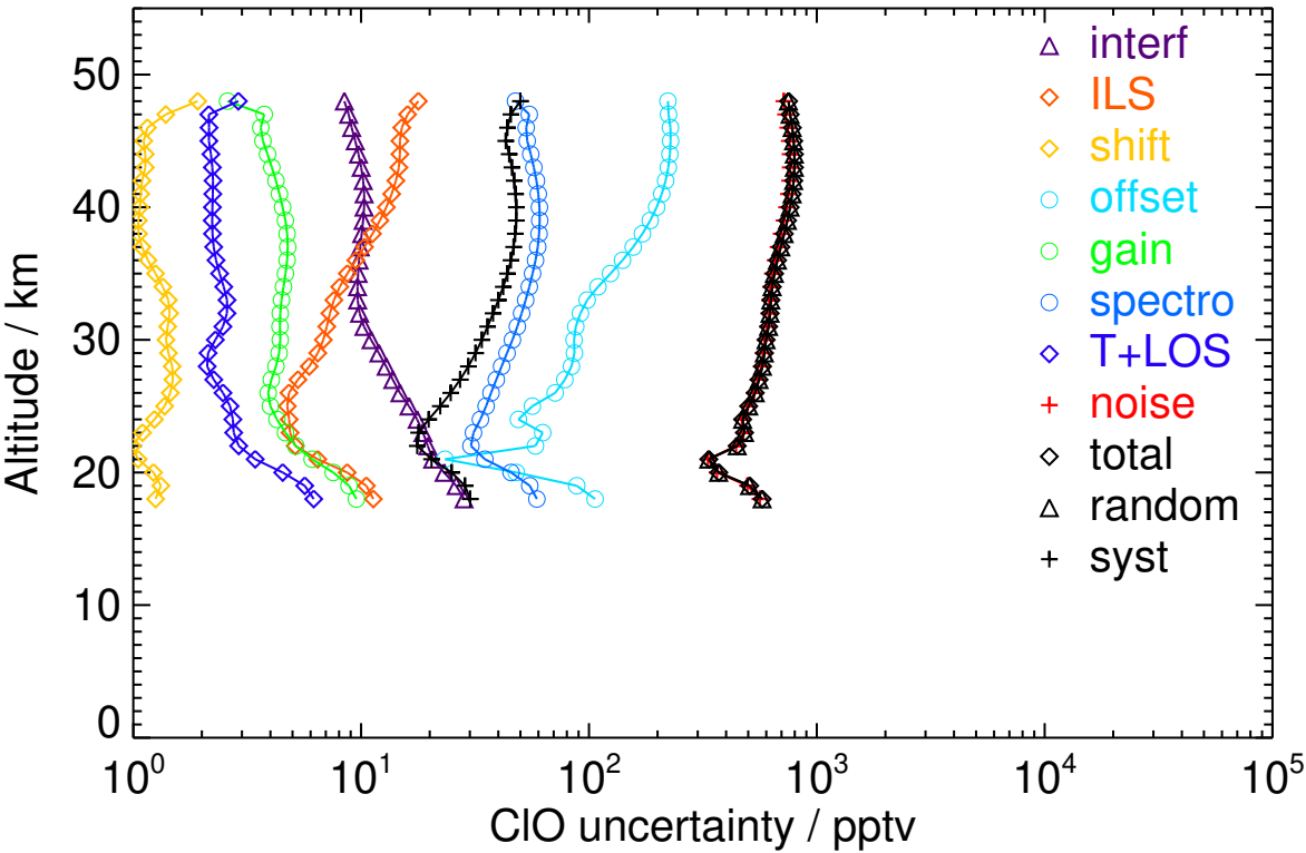
Figure S101. V8R_CLO_562 Southern polar autumn day
