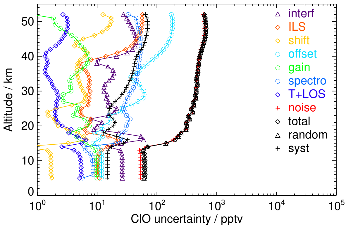
Figure S65. V8R_CLO_262 Southern polar summer day
