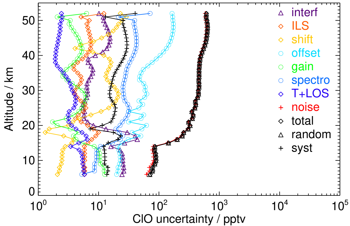
Figure S16. V8H_CLO_62 Northern midlatitude autumn night
