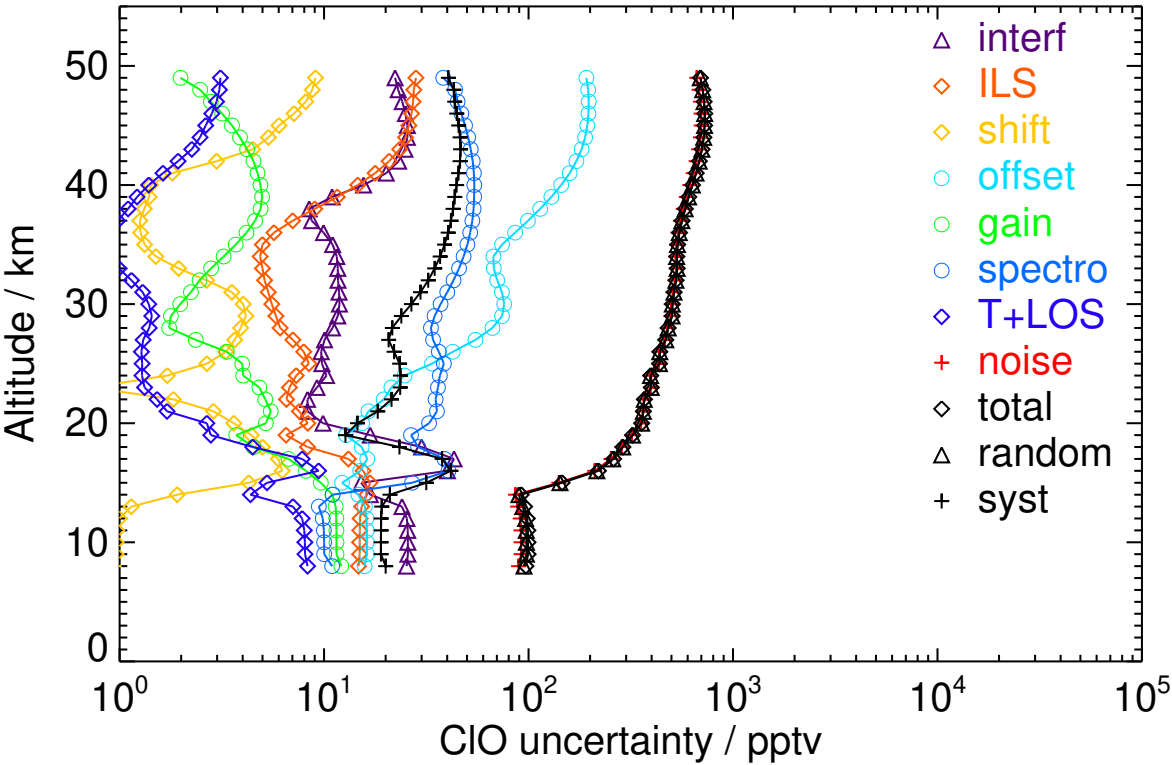
Figure S49. V8R_CLO_262 Northern midlatitude autumn day
