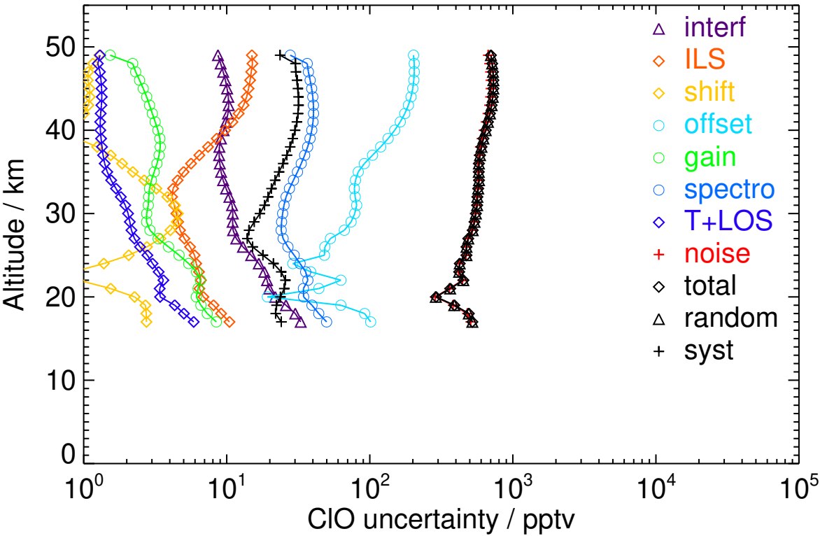
Figure S84. V8R_CLO_562 Northern midlatitude autumn night
