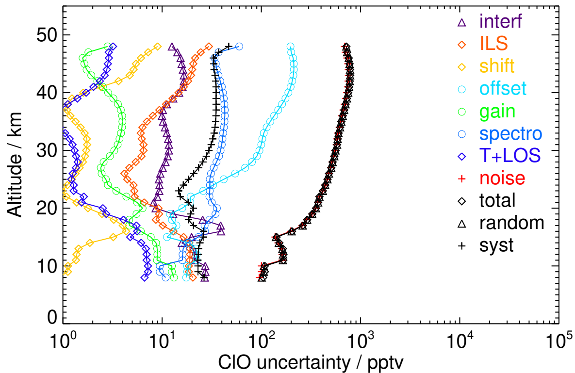
Figure S41. V8R_CLO_262 Northern polar autumn day
