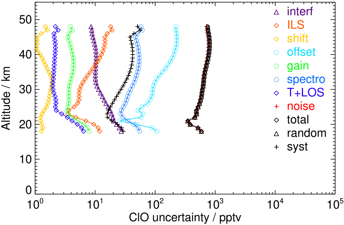
Figure S102. V8R_CLO_562 Southern polar autumn night
