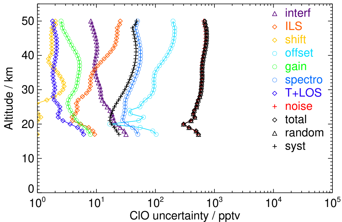
Figure S71. V8R_CLO_562 Northern polar spring day
