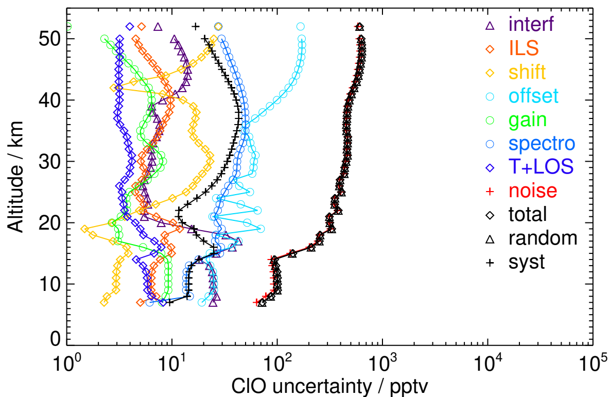
Figure S15. V8H_CLO_62 Northern midlatitude autumn day
