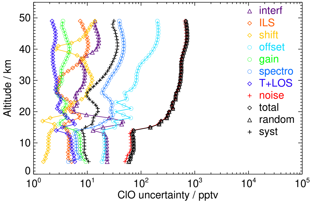
Figure S34. V8H_CLO_62 Southern polar autumn night
