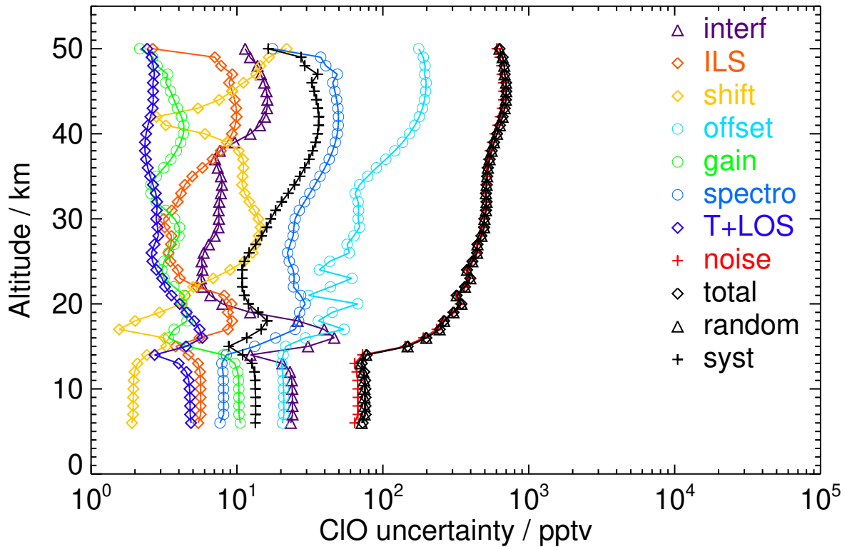
Figure S8. V8H_CLO_62 Northern polar autumn night
