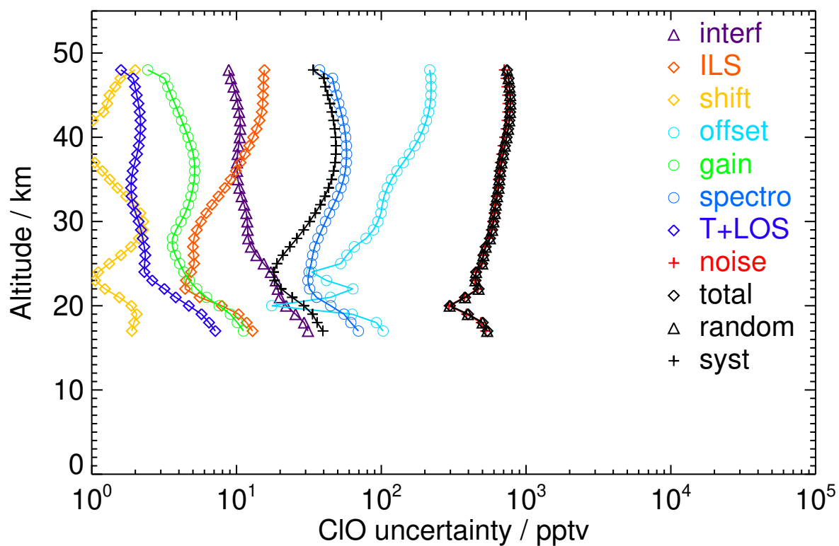
Figure S75. V8R_CLO_562 Northern polar autumn day
