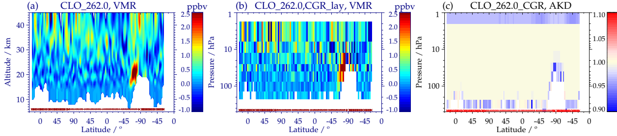
Figure 7. (a) Regular and (b) coarse grid representation of MIPAS V8 CIO, measured on 4 September 2007 during Envisat orbit 28825. Nighttime measurements are indicated by red crosses and daytime measurements by red plus signs at the bottom of the plots. White areas are missing data due to clouds, in particular PSCs near the South Pole. Fig.7a is repeated from Fig.5b, but with a truncated vertical range. (c) Diagonal elements of the averaging kernels of the V8 CIO coarse grid retrieval.
