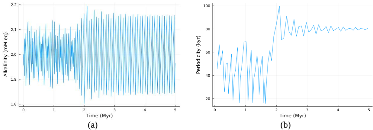
Figure 1. C-A system under orbital forcing ( A(0) = 2.0 mM eq, C(0) = 4 * 10^{-5} mM eq, \alpha = 0.012 , T = 40 kyr): (a) alkalinity, (b) dominant period as a function of time
