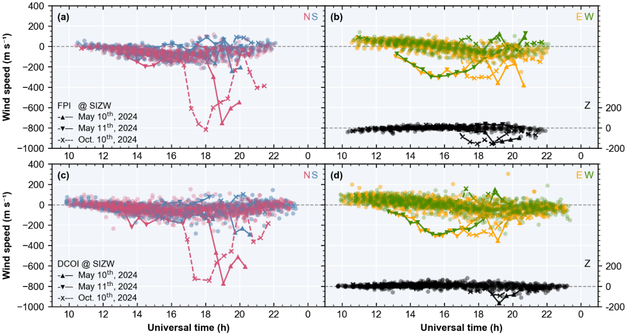
179 Figure 2: Storm-time (Kp>3) thermospheric wind speed statistics at SIZW
