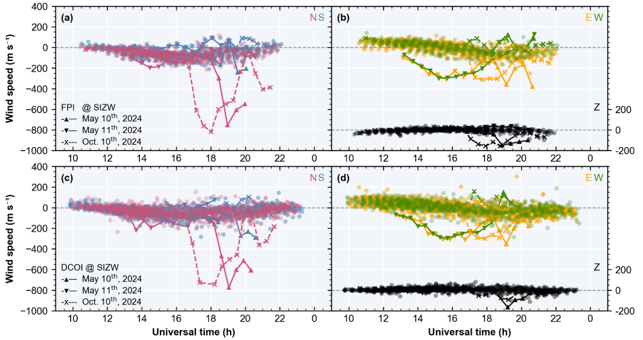
Figure 2: Storm-time (Kp>3) thermospheric wind speed statistics at SIZW
