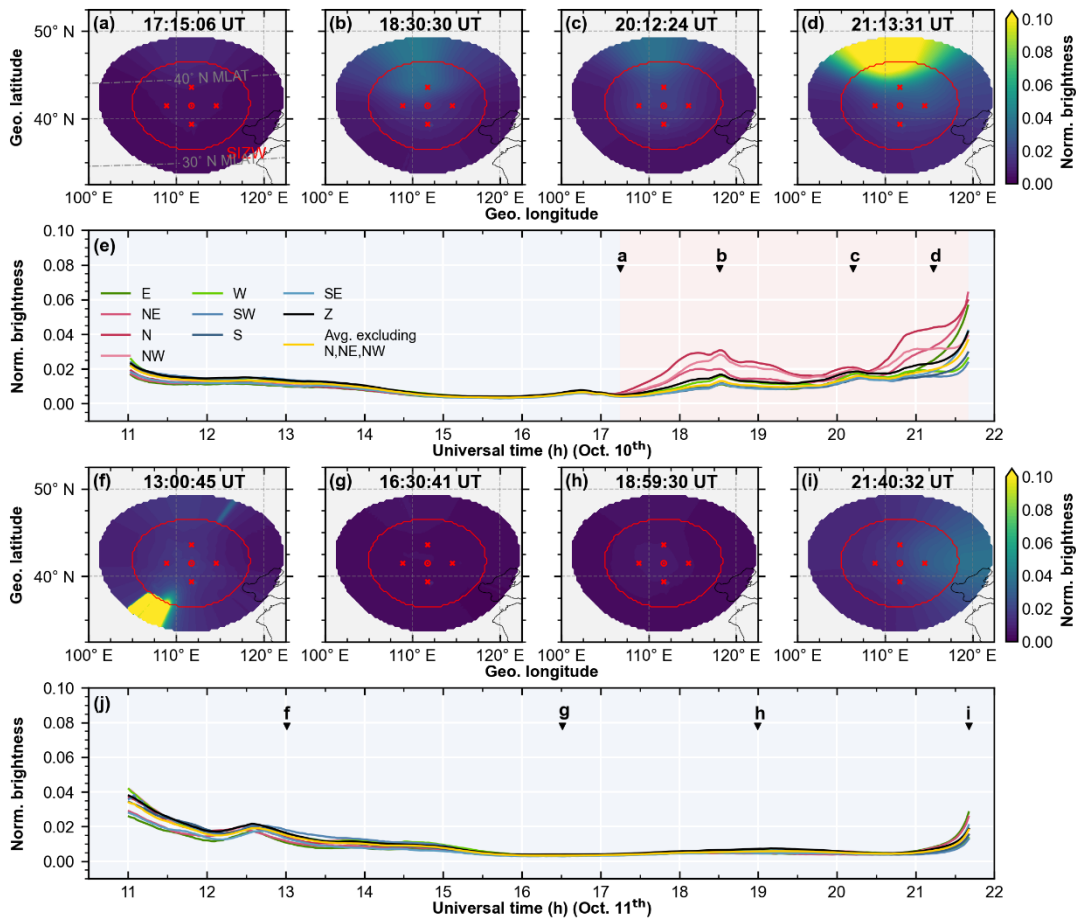
286 Figure 6: Auroral distribution observed by DCAI on the nights of Oct. 10 th and 11 th , 2024, at SIZW 287 Figure 6 is analogous to Fig. 4, but for Oct. 10 th and 11 th . 288
