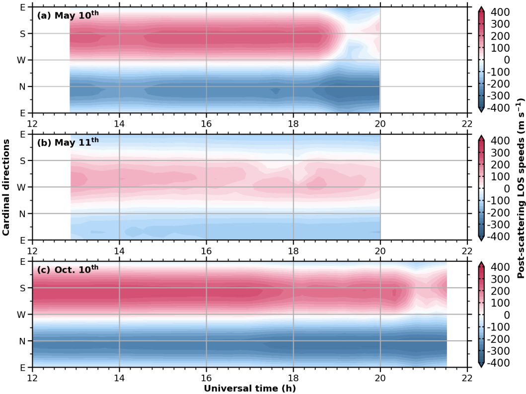
337 338 Figure 7: Post-scattering LOS speeds at 45° zenith angle
