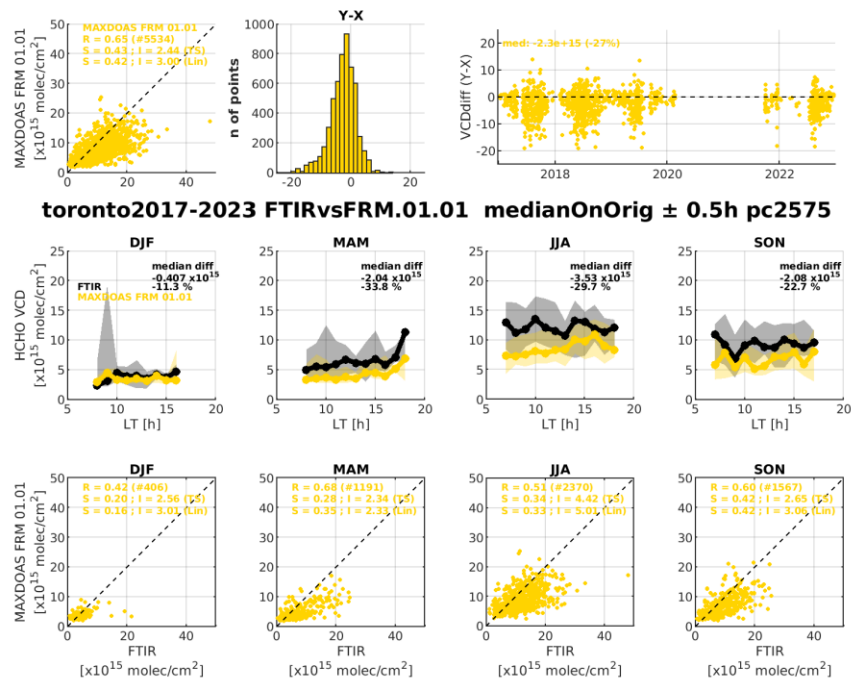
Figure ans4: as Fig3 of the paper, but for Toronto FTIR vs MAX-DOAS MMF for Bremen over 2019-2022.
